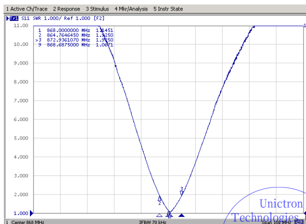
VSWR ( S_{11} )
