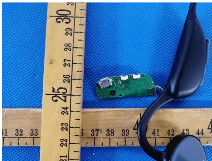
INTERNAL VIEW-5 OF EUT
