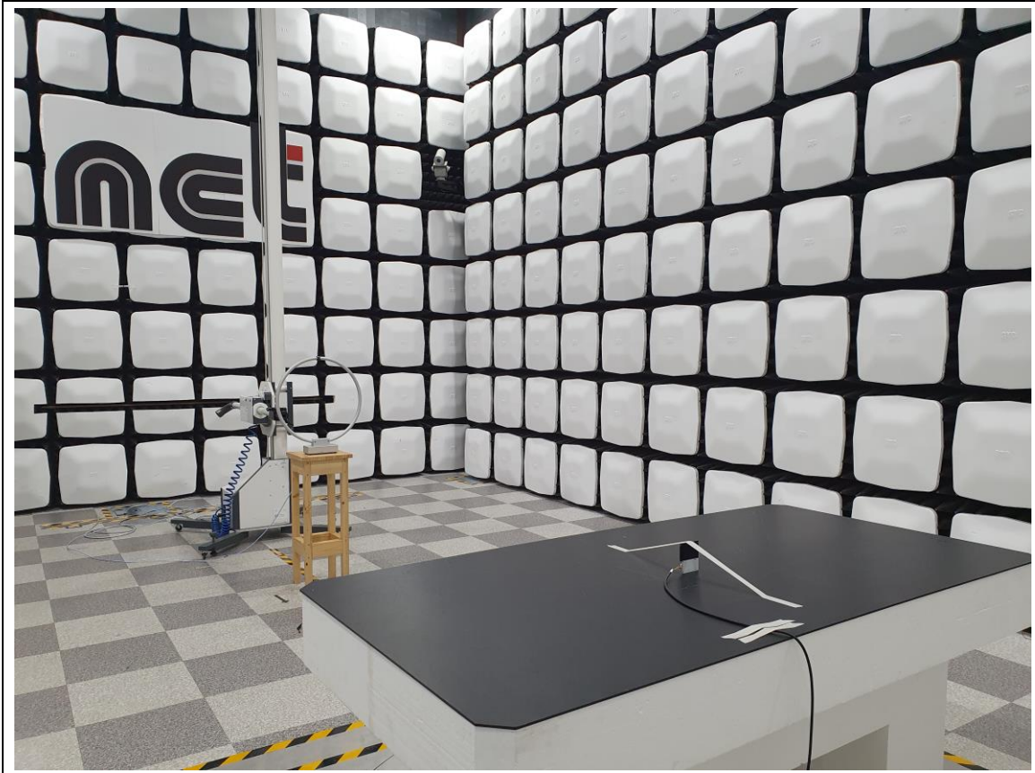
Below 30 MHz
