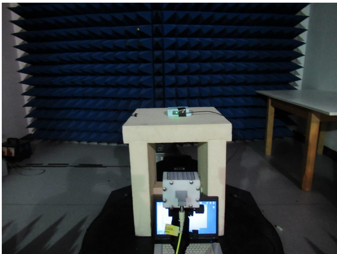
40 GHz – 200 GHz
