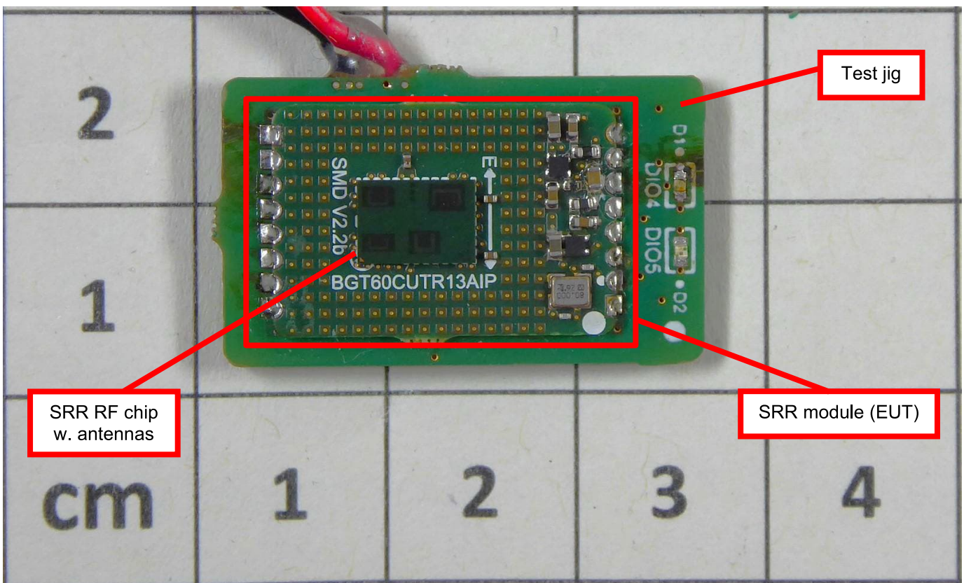
(EUT mounted on test jig with attached power supply cabling)
