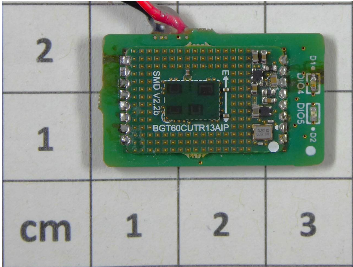
(EUT on test jig – front view)
