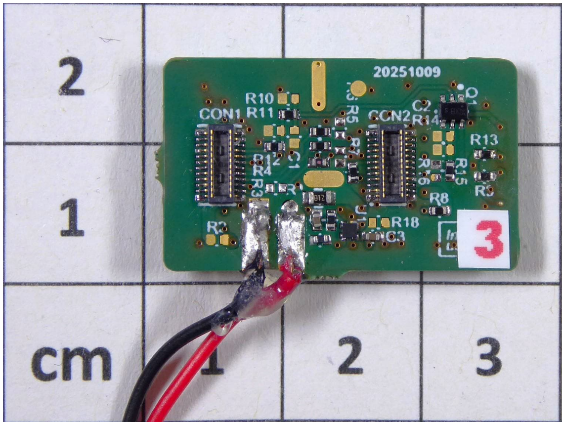
(EUT on test jig – back view)
