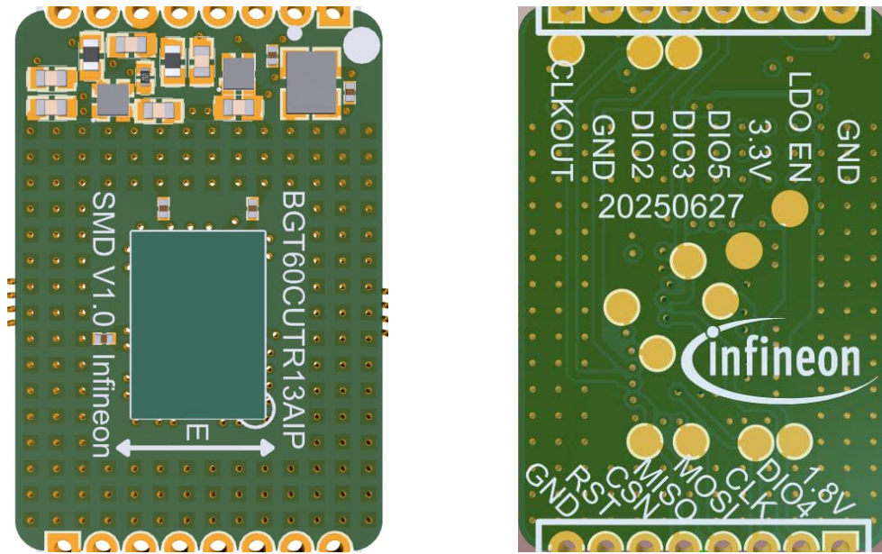
(3D pictures of the SRR module (EUT) in final version: front (left) and back (right))
