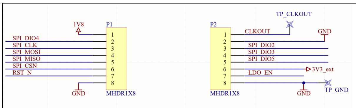
Figure 5 Schematic of the Xensiv™ BGT60CUTR13AIP SMD module half stamp hole connectors
