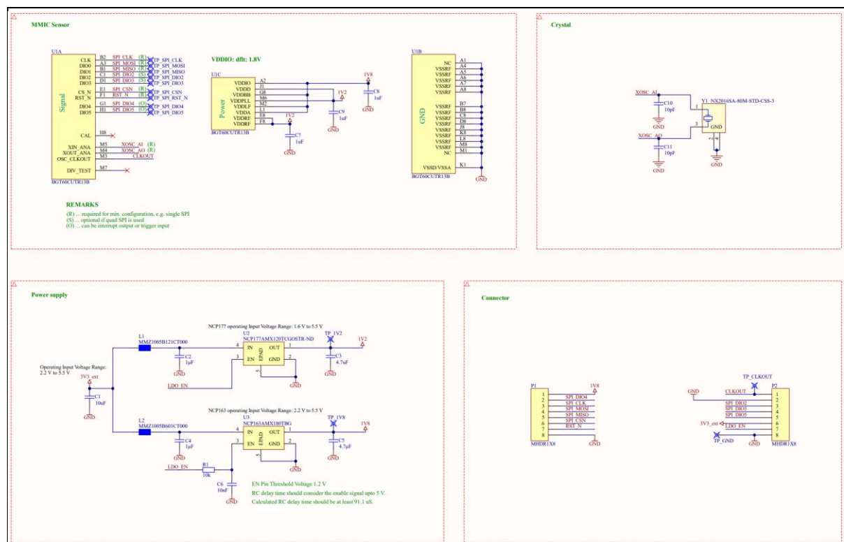
Figure 1 Schematic overview of Xensiv™ BGT60CUTR13AIP SMD module
