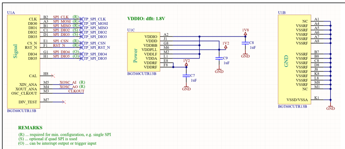
Figure 4 Schematic of the Xensiv™ BGT60CUTR13AIP SMD module radar SoC circuitry
