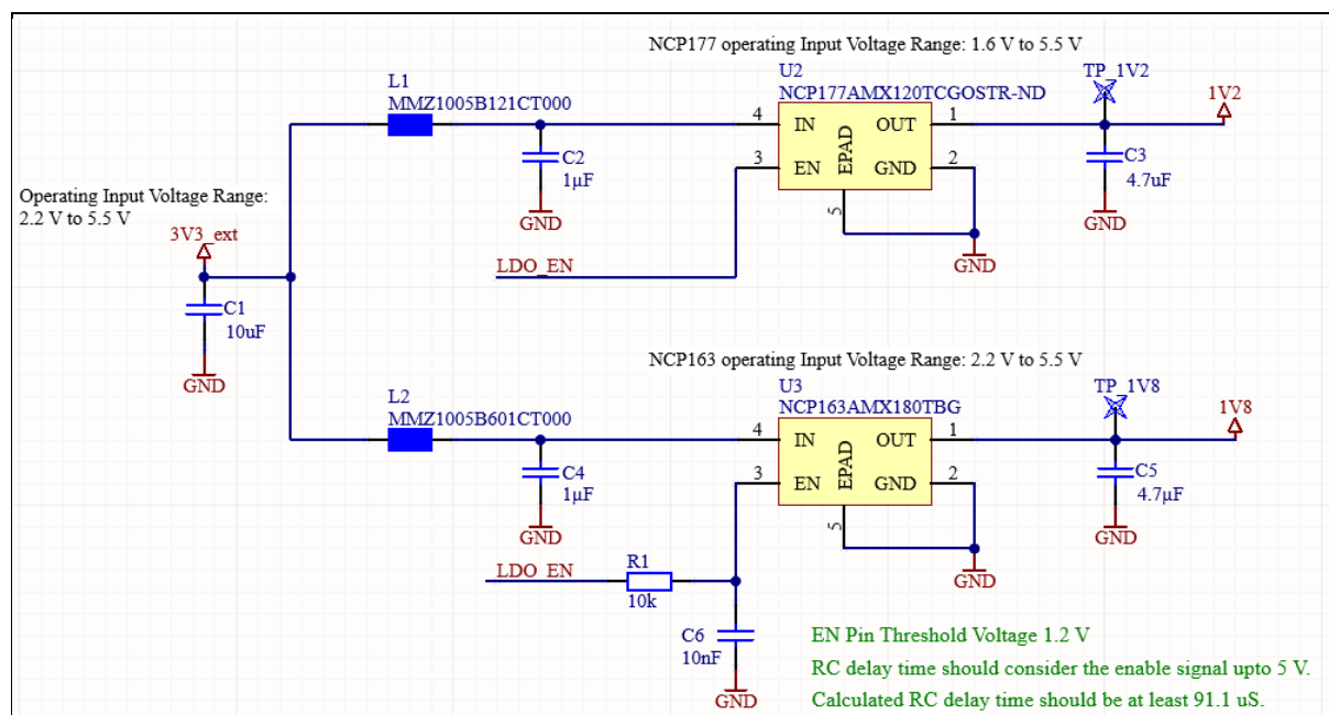
Figure 2 Schematic of the Xensiv™ BGT60CUTR13AIP SMD module power supply circuitry
