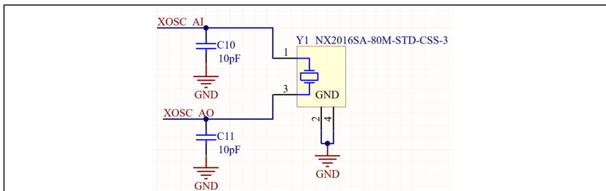
Figure 3 Schematic of the Xensiv™ BGT60CUTR13AIP SMD module XTAL resonator circuitry
