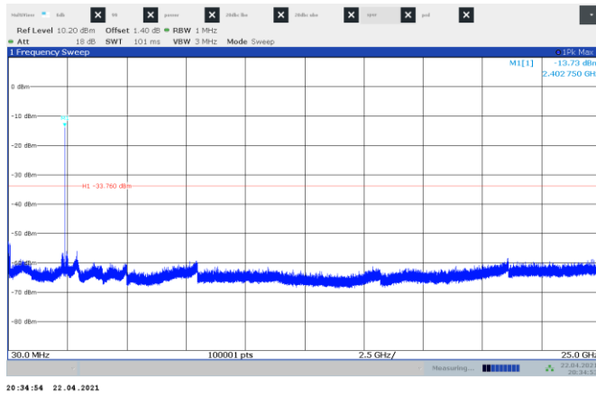
Figure 8.6-7: Conducted spurious emissions on low channel
