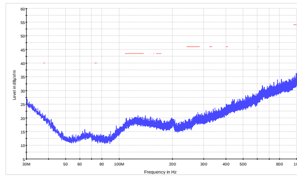
Access Tech RE scan 30 MHz to 1 GHz high channel PK+ MAXH FCC 15.209 and RSS-Gen Restricted bands average limits
