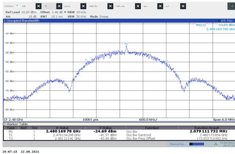
Figure 8.4-6: 99% occupied bandwidth on high channel
