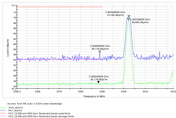
Figure 8.6-3: Radiated Restricted band edge spurious emissions low ch. -
