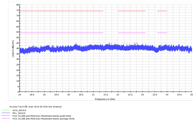
Figure 8.6-16: Radiated spurious emissions 18-25 GHz on low channel
