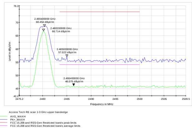
Figure 8.6-4: Radiated Restricted band edge spurious emissions high ch. -
