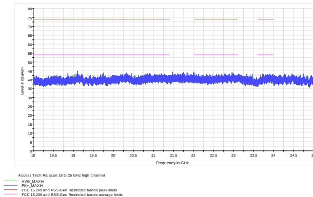
Figure 8.6-18: Radiated spurious emissions 18-25 GHz on high channel
