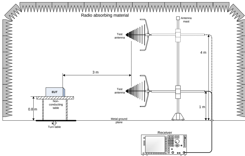
Figure 5.5-1: Radiated testing block diagram below 1 GHz
