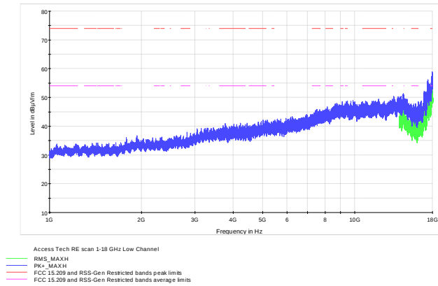
Figure 8.6-13: Radiated spurious emissions 1-18 GHz on low channel
