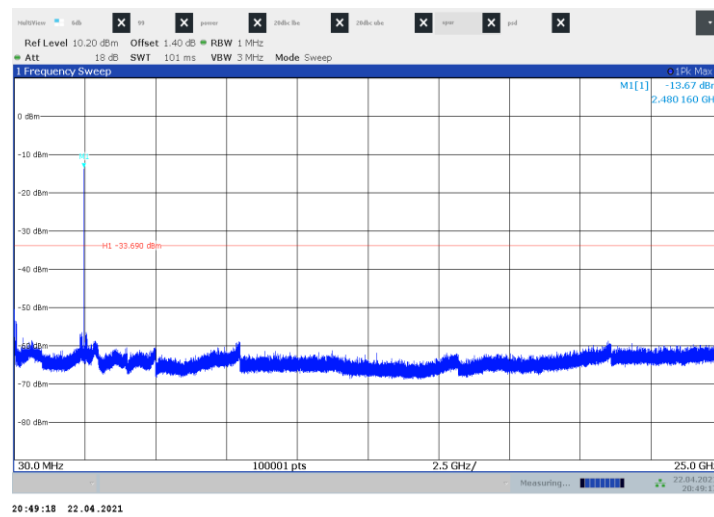
Figure 8.6-9: Conducted spurious emissions on high channel
