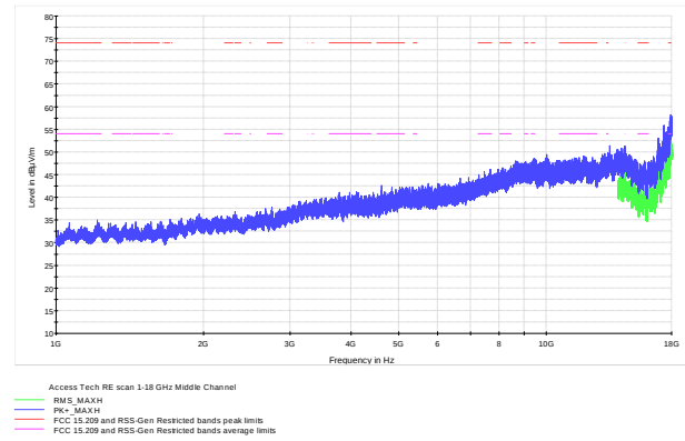
Figure 8.6-14: Radiated spurious emissions 1-18 GHz on mid channel
