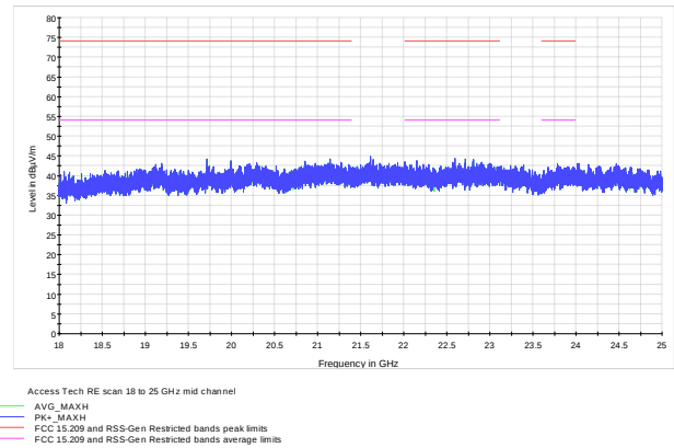
Figure 8.6-17: Radiated spurious emissions 18-25 GHz on mid channel
