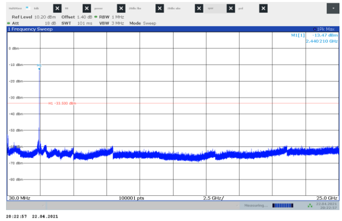
Figure 8.6-8: Conducted spurious emissions on mid channel
