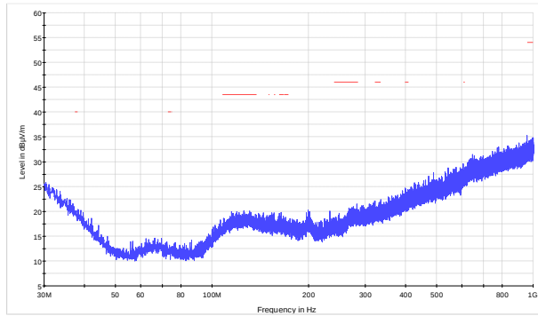
Access Tech RE scan 30 MHz to 1 GHz low channel PK+ MAXH FCC 15.209 and RSS-Gen Restricted bands average limits
