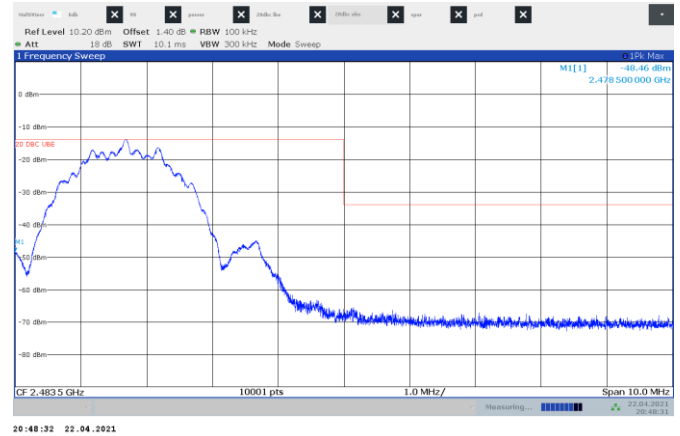
Figure 8.6-2: Conducted Band edge spurious emissions at 2483.5 MHz
