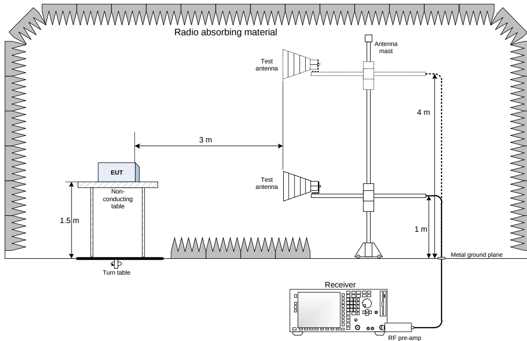
Figure 5.5-2: Radiated testing block diagram above 1 GHz
