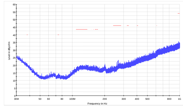
Access Tech RE scan 30 MHz to 1 GHz mid channel PK+ MAXH FCC 15.209 and RSS-Gen Restricted bands average limits
