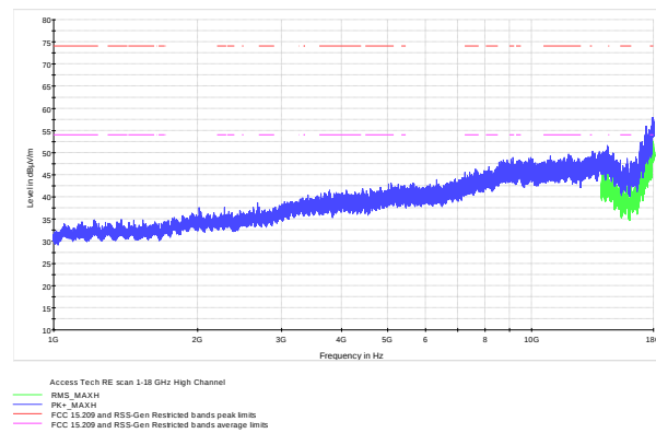
Figure 8.6-15: Radiated spurious emissions 1-18 GHz on high channel
