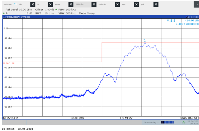
Figure 8.6-1: Conducted Band edge spurious emissions at 2400 MHz
