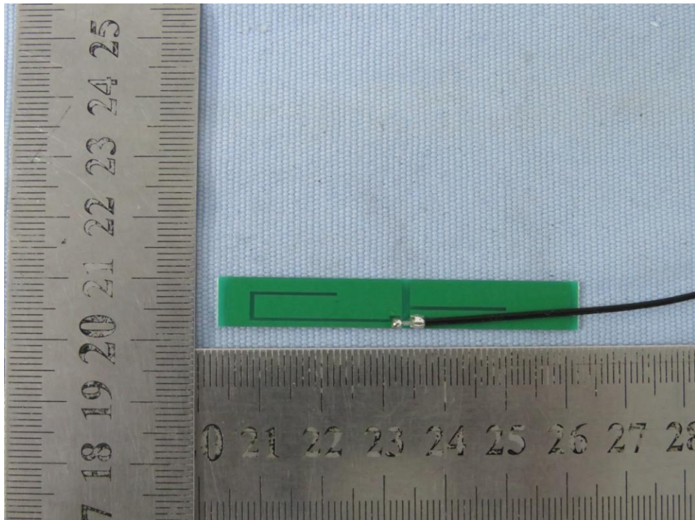
Antenna - RF915-2
