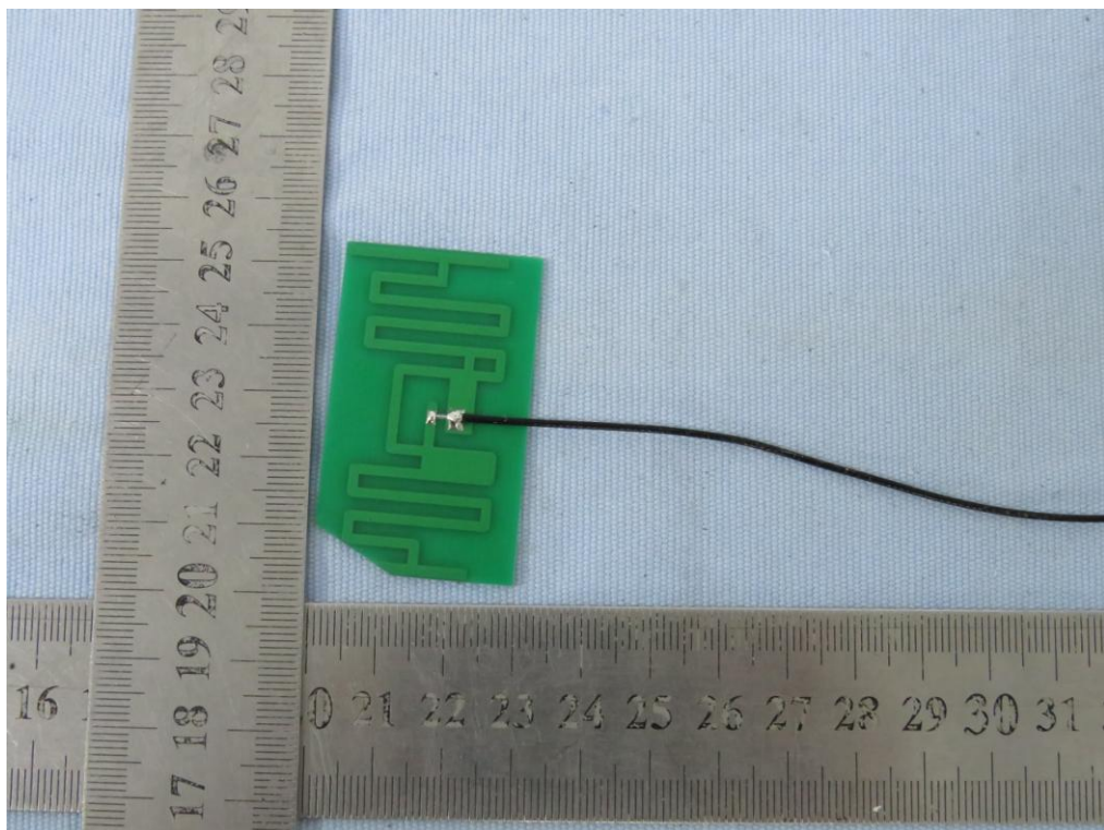
Antenna - RF915-1
