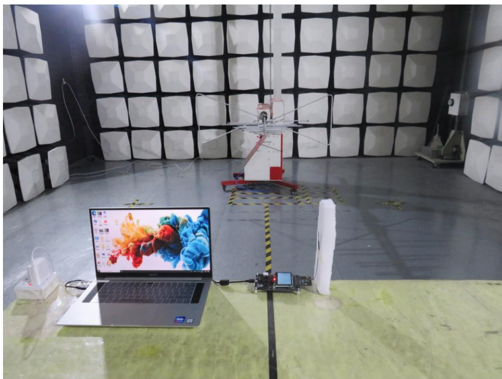
Radiated emission (Above 1GHz) -Antenna RF915-2
