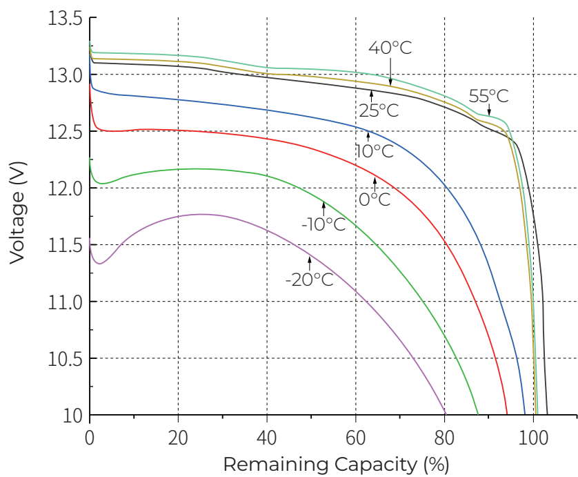
Discharge capacity at 0.5C across different temperatures
