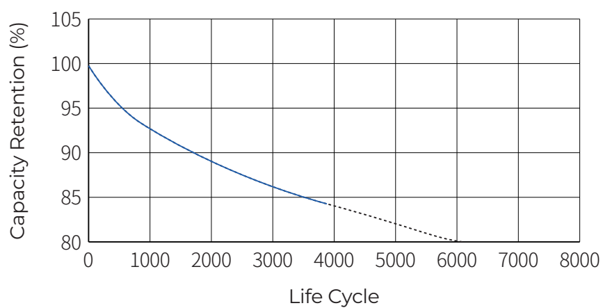
Cycle life at 0.5C, 77°F (25°C)
