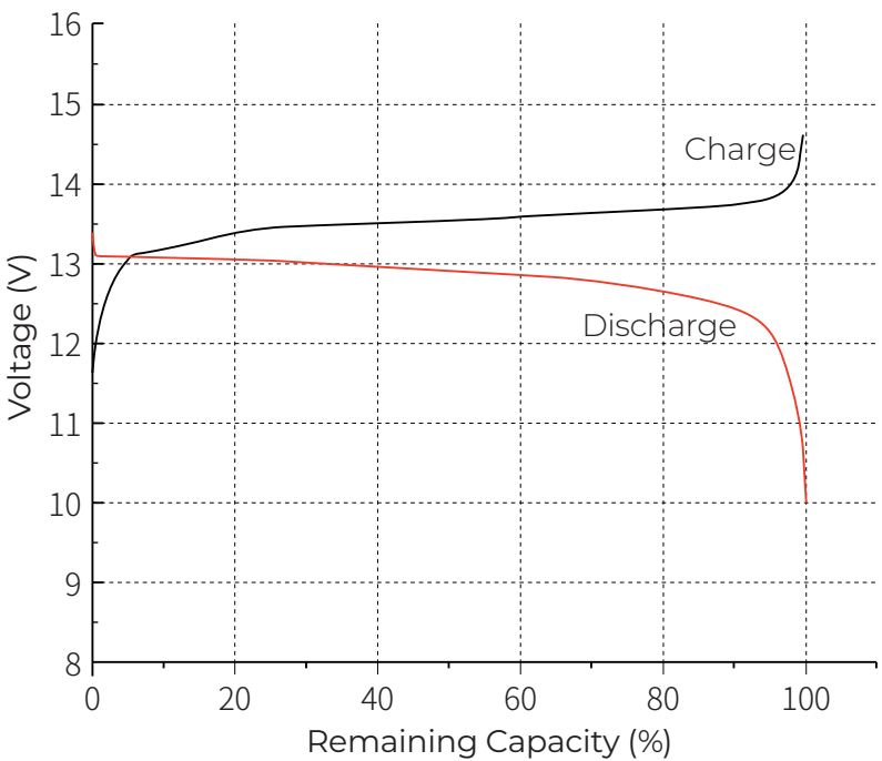
Charging & discharging curve at 0.5C, 77°F (25°C)
