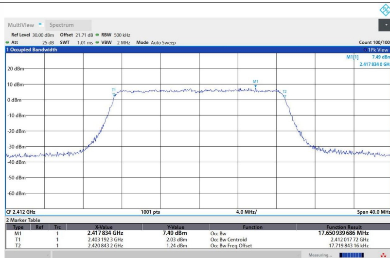
11N20SISO-Ant1-2412
