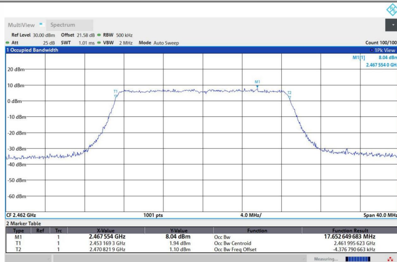
11N20SISO-Ant1-2462
