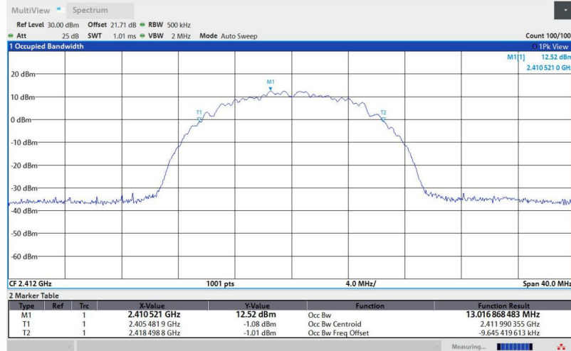
11B-Ant1-2412
