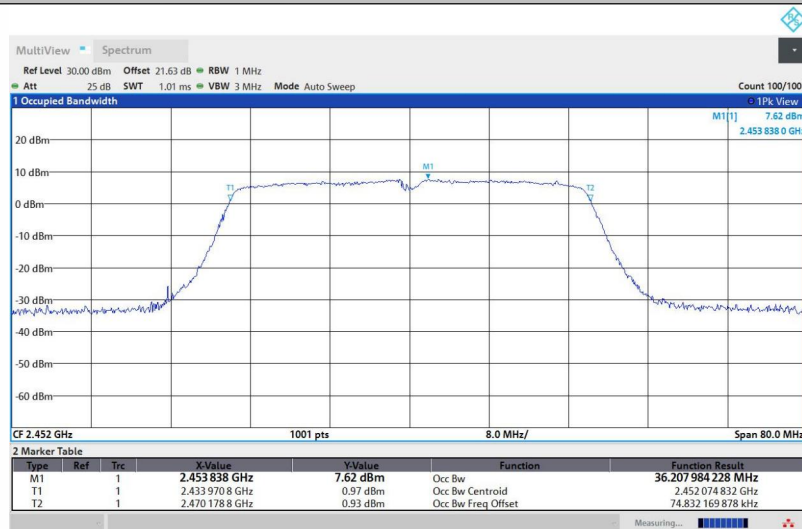
11N40SISO-Ant1-2452
