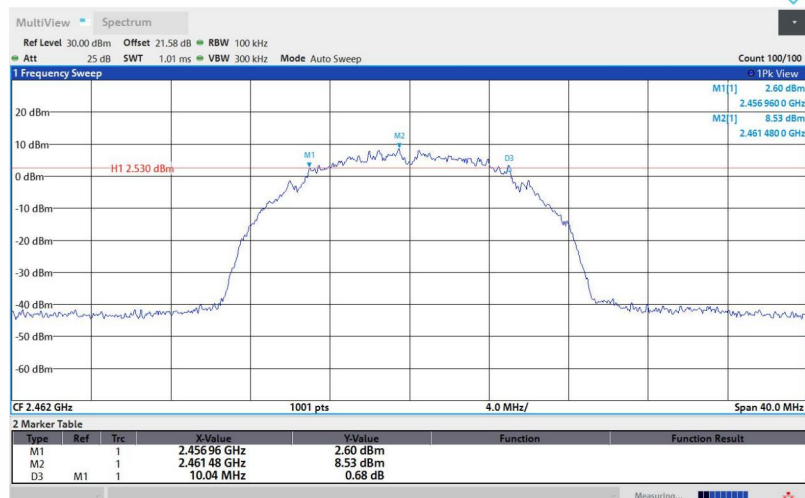
11B-Ant1-2462-PASS
