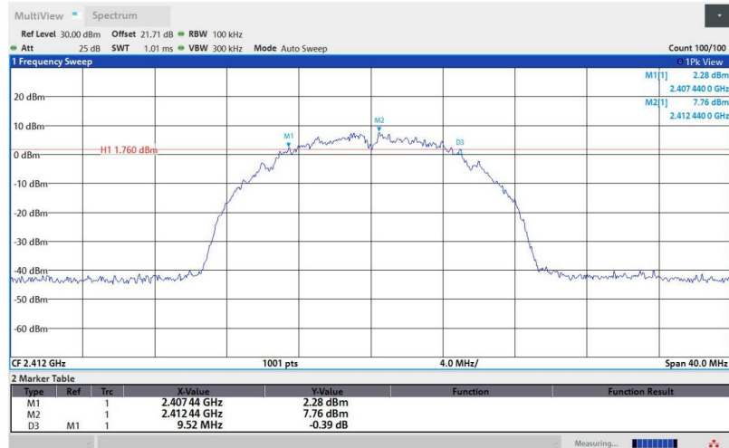
11B-Ant1-2412-PASS
