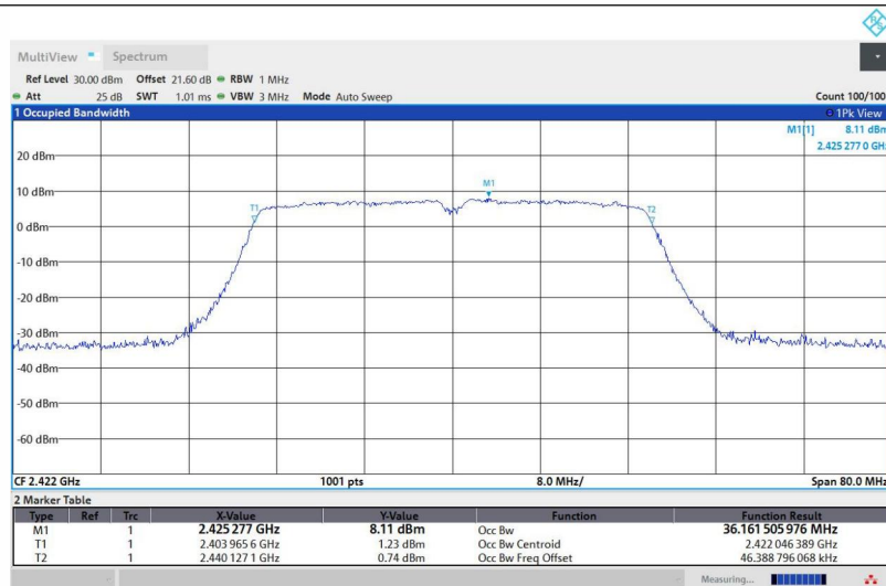
11N40SISO-Ant1-2422
