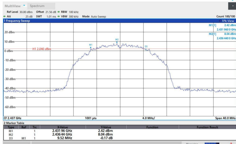
11B-Ant1-2437-PASS
