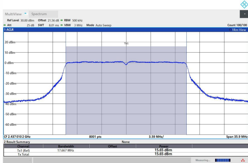
11N20ISO-Ant1-2437-PASS
