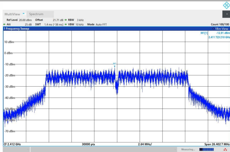
11G-Ant1-2412-PASS
