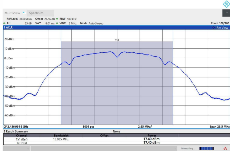
11B-Ant1-2437-PASS
