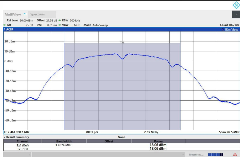
11B-Ant1-2462-PASS
