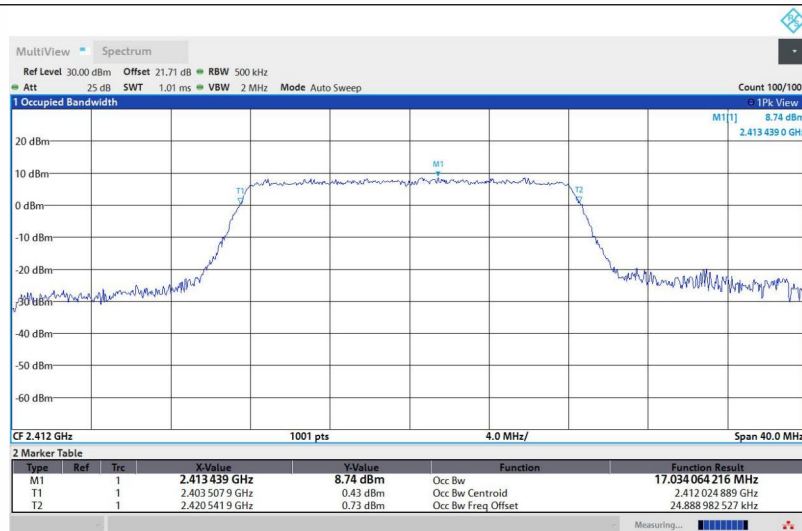
11G-Ant1-2412
