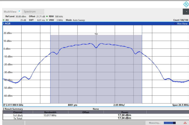
11B-Ant1-2412-PASS
