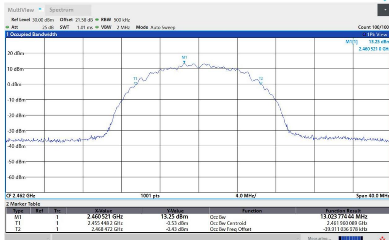
11B-Ant1-2462
