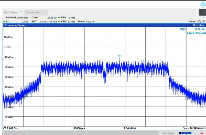
11G-Ant1-2462-PASS
