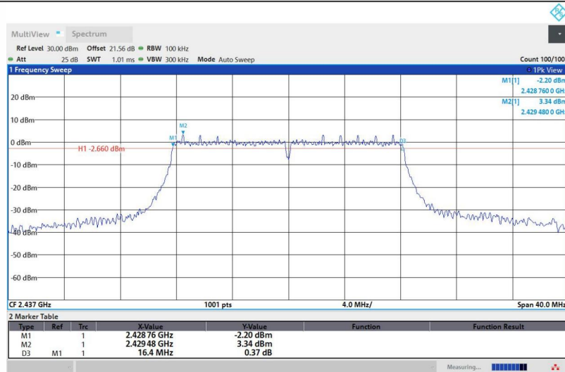
11G-Ant1-2437-PASS
