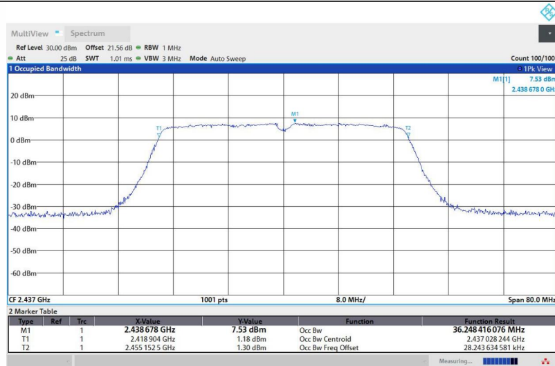
11N40SISO-Ant1-2437
