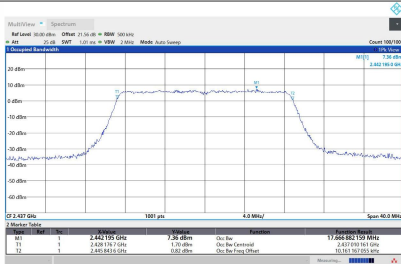
11N20SISO-Ant1-2437
