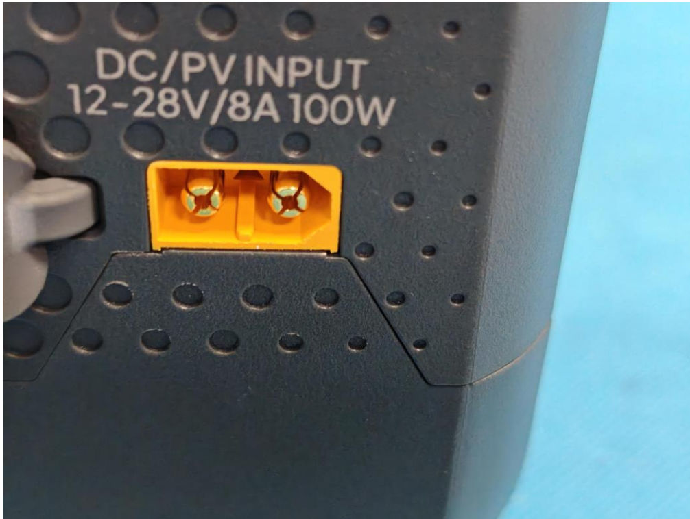
Port-1 View of EUT
