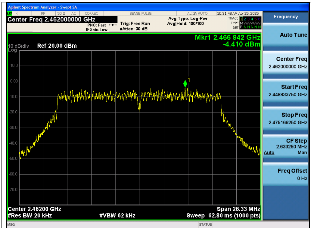
Test_Graph_802.11n20_ANT1_2462_MCS0_PSD
