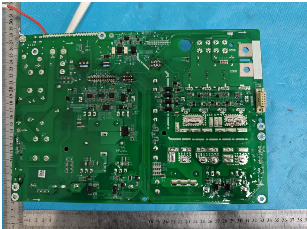
Internal view-10 of EUT
