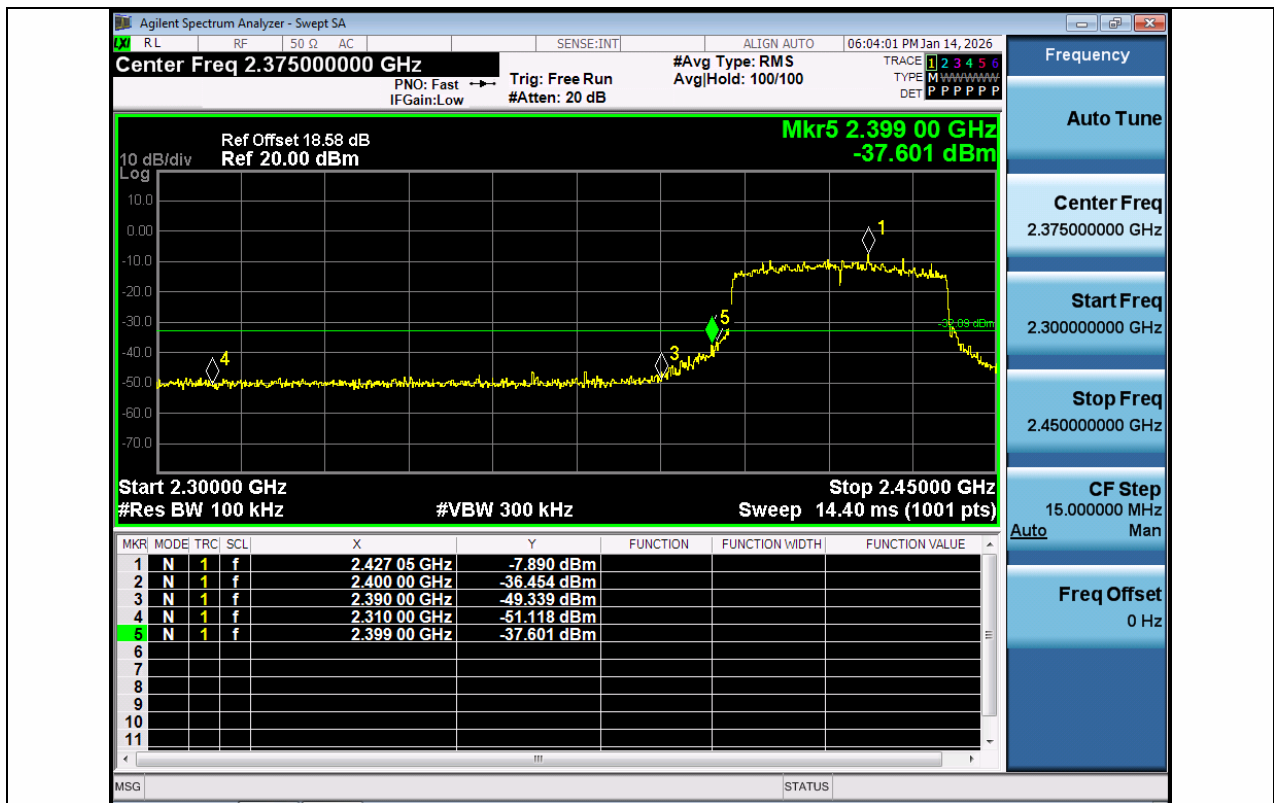
11AX40SISO-Ant1-2422-PASS
