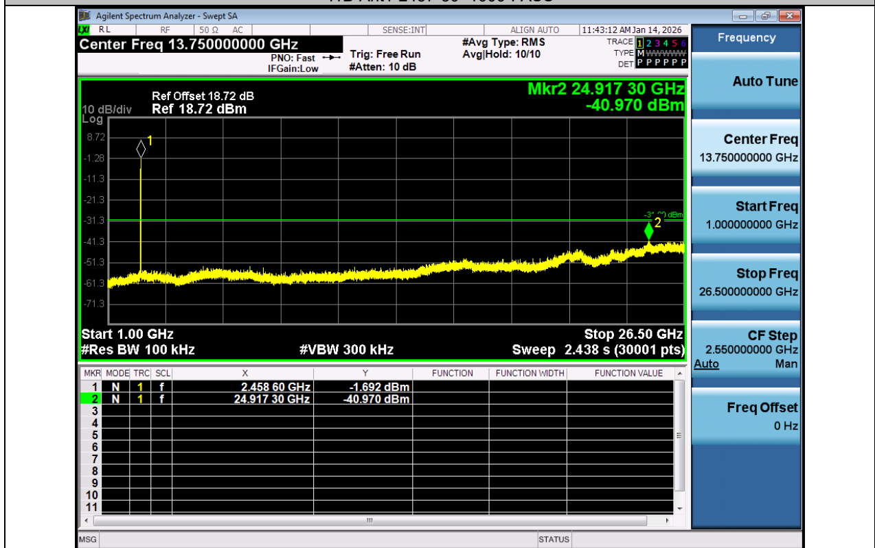
11B-Ant1-2457-1000~26500-PASS
