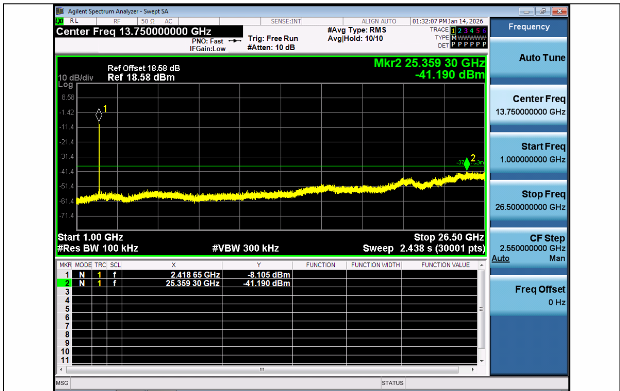
11G-Ant1-2417-1000~26500-PASS
