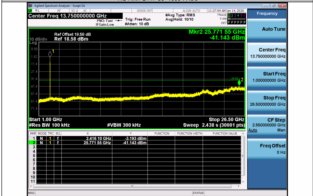
11B-Ant1-2417-1000~26500-PASS
