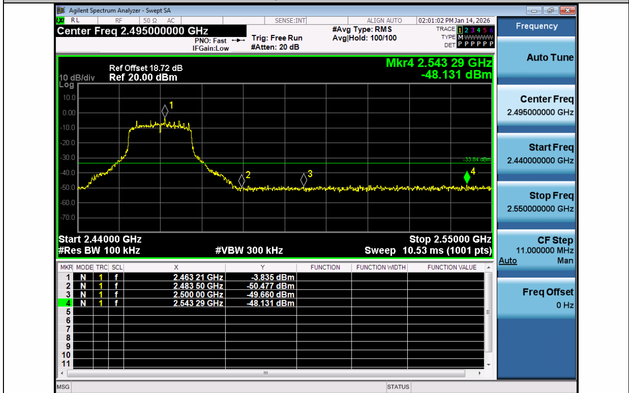
11G-Ant1-2462-PASS
