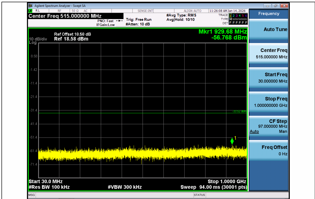
11B-Ant1-2417-30~1000-PASS
