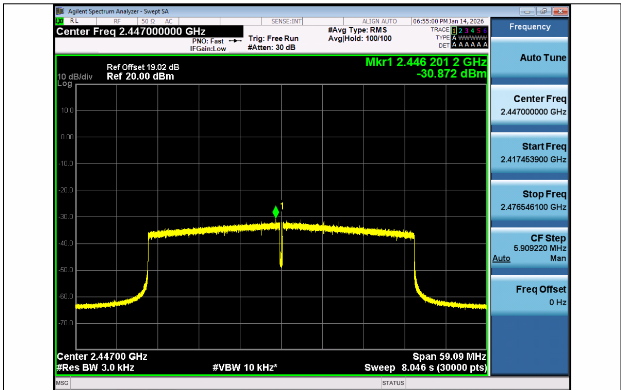
11AX40SISO-Ant1-2447-PASS
