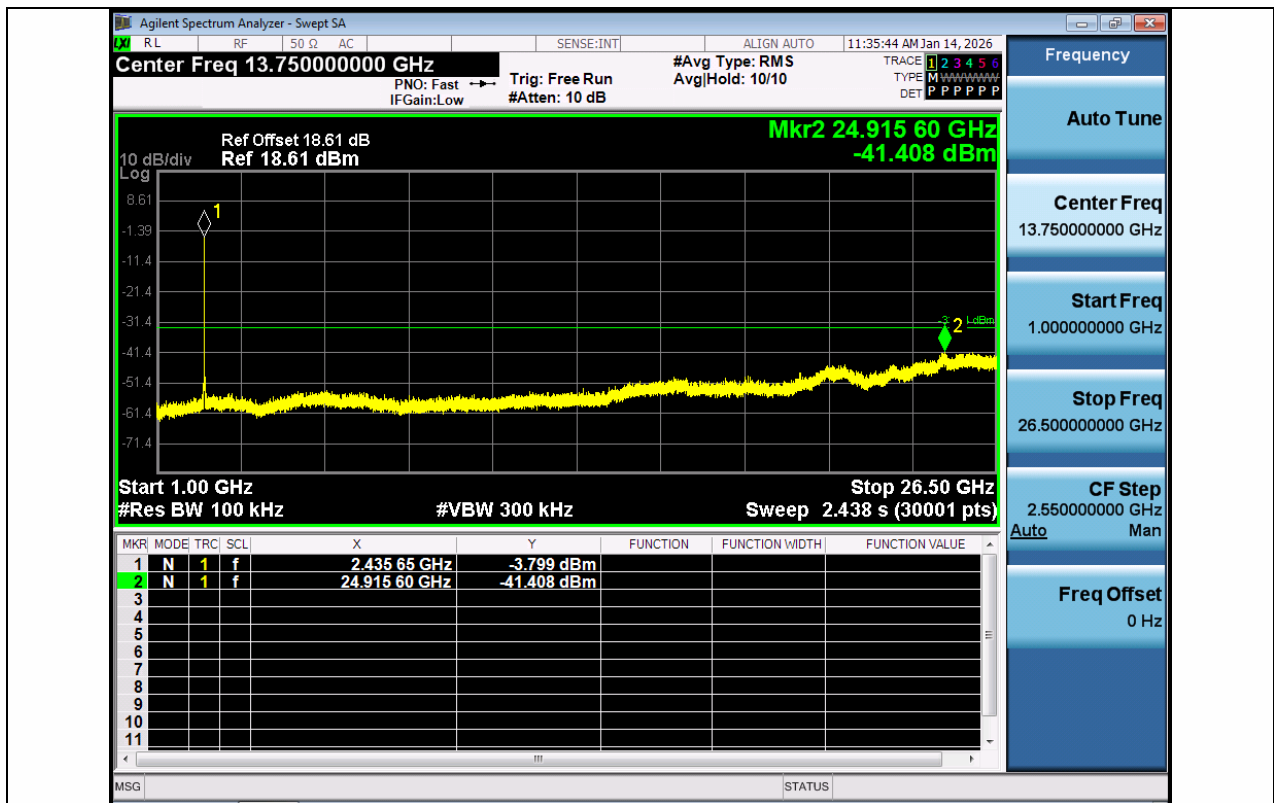
11B-Ant1-2437-1000~26500-PASS
