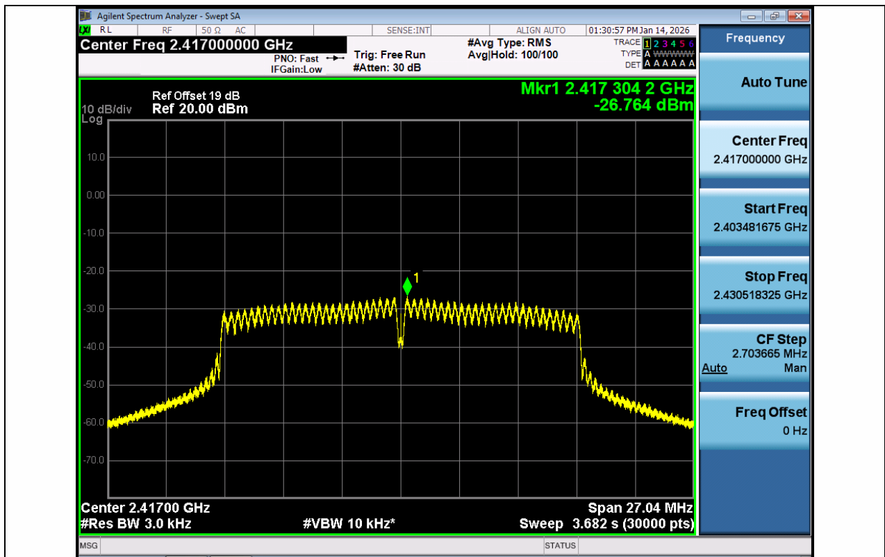
11G-Ant1-2417-PASS
