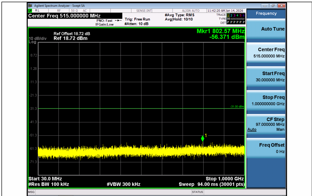
11B-Ant1-2457-30~1000-PASS
