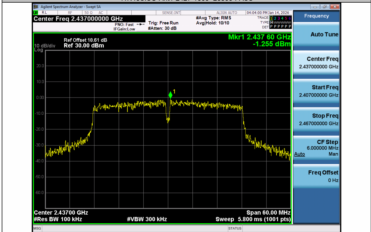
11N40SISO-Ant1-2437-0~Reference-PASS
