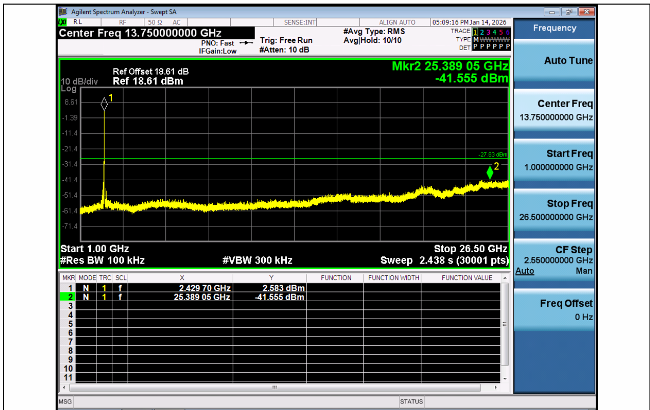
11AX20SISO-Ant1-2437-1000~26500-PASS
