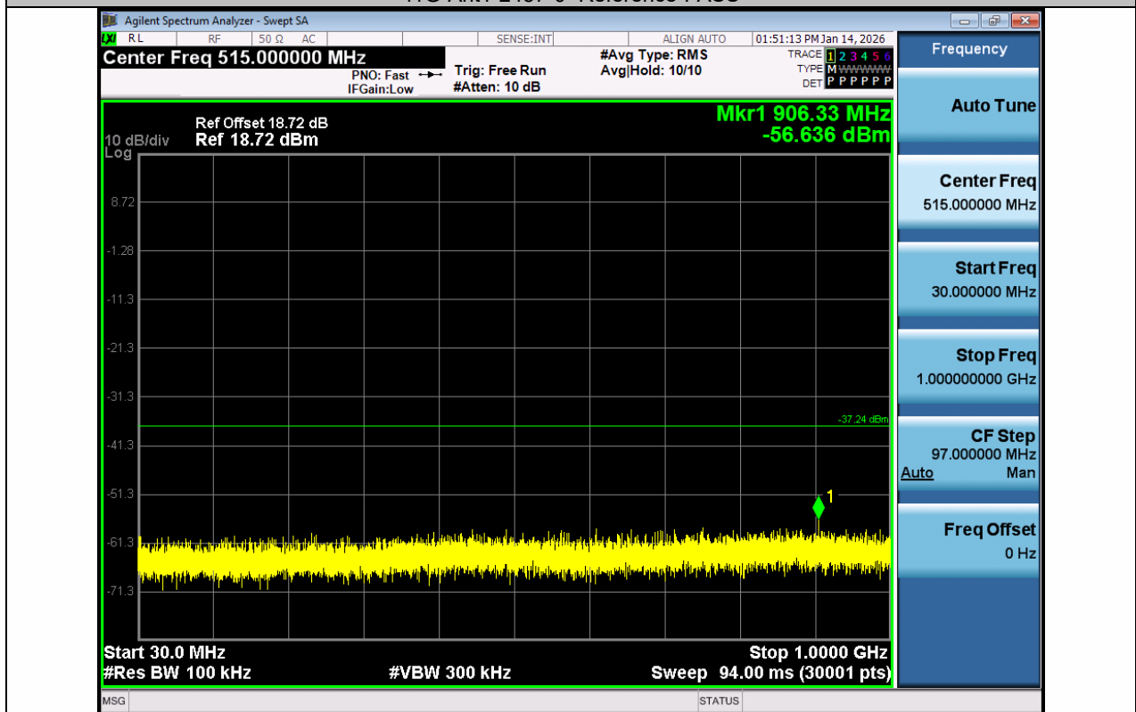
11G-Ant1-2457-30~1000-PASS
