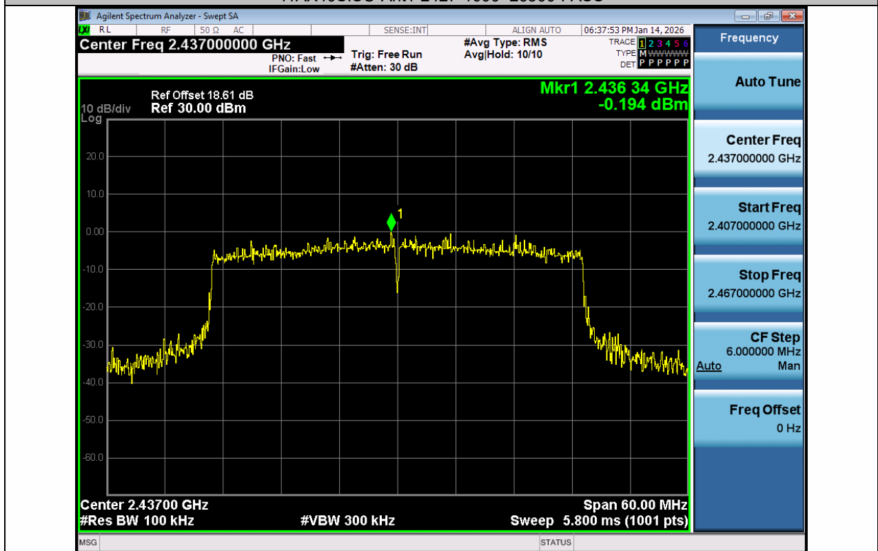
11AX40SISO-Ant1-2437-0~Reference-PASS
