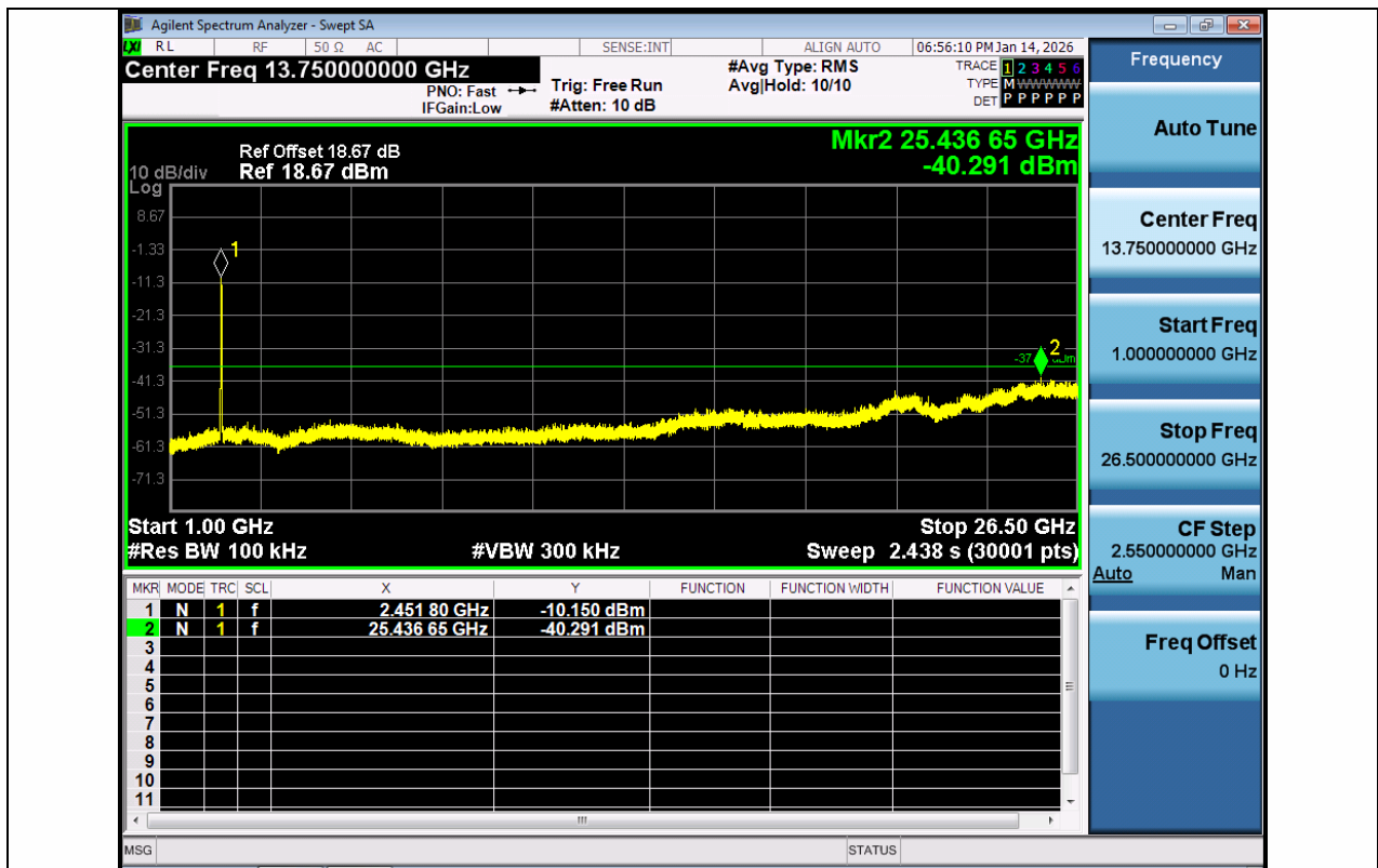
11AX40SISO-Ant1-2447-1000~26500-PASS
