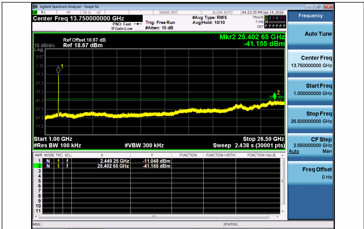
11N40SISO-Ant1-2447-1000~26500-PASS
