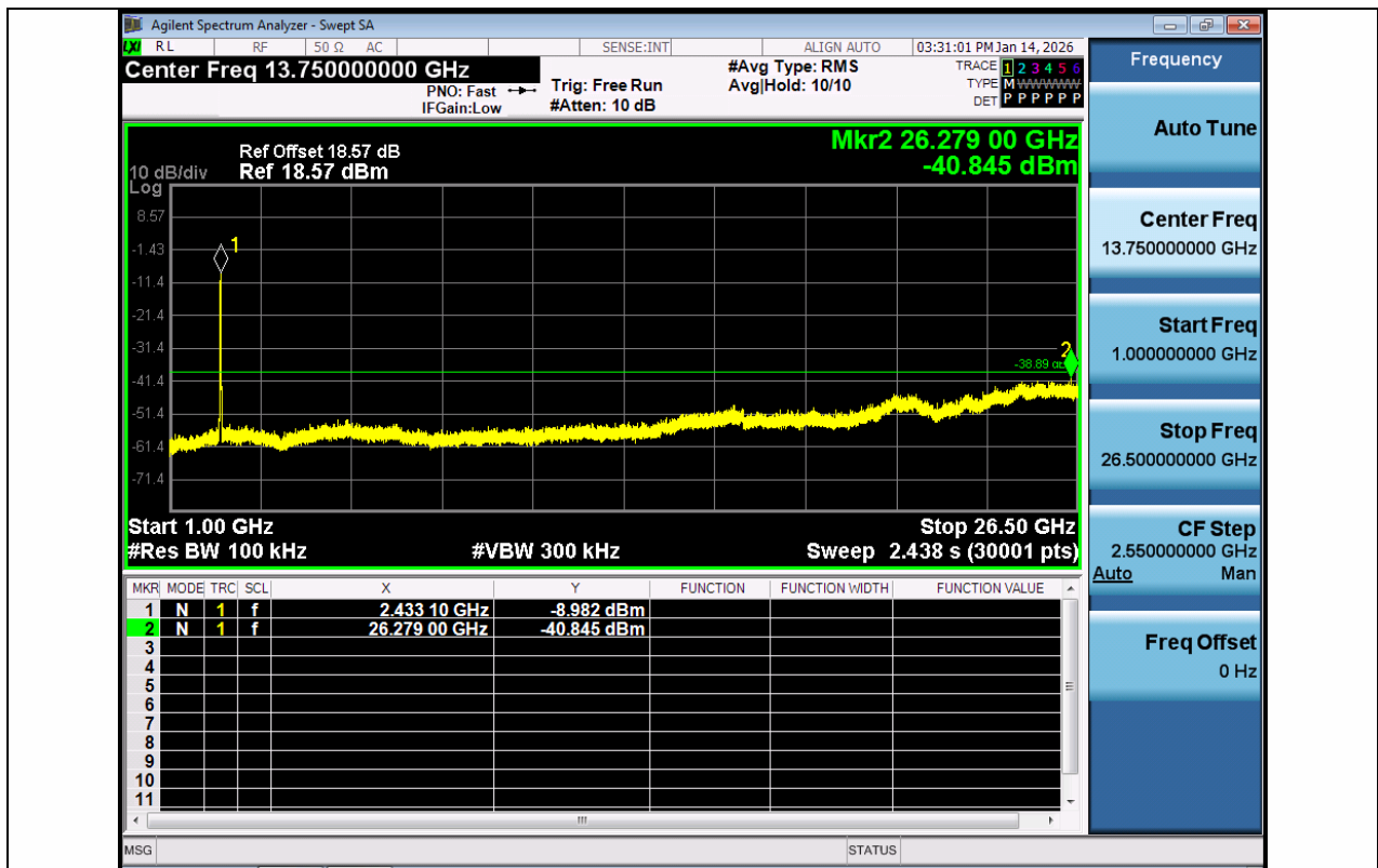
11N40SISO-Ant1-2427-1000~26500-PASS
