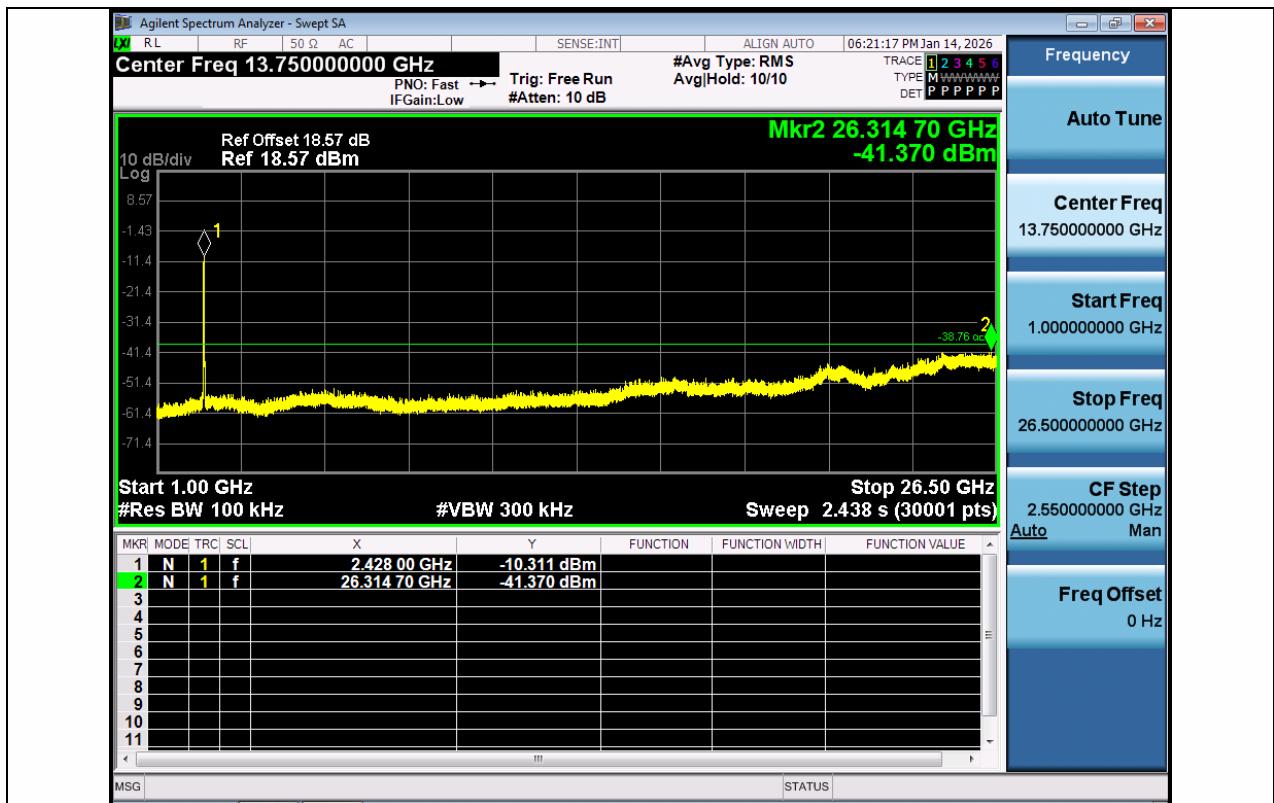
11AX40SISO-Ant1-2427-1000~26500-PASS
