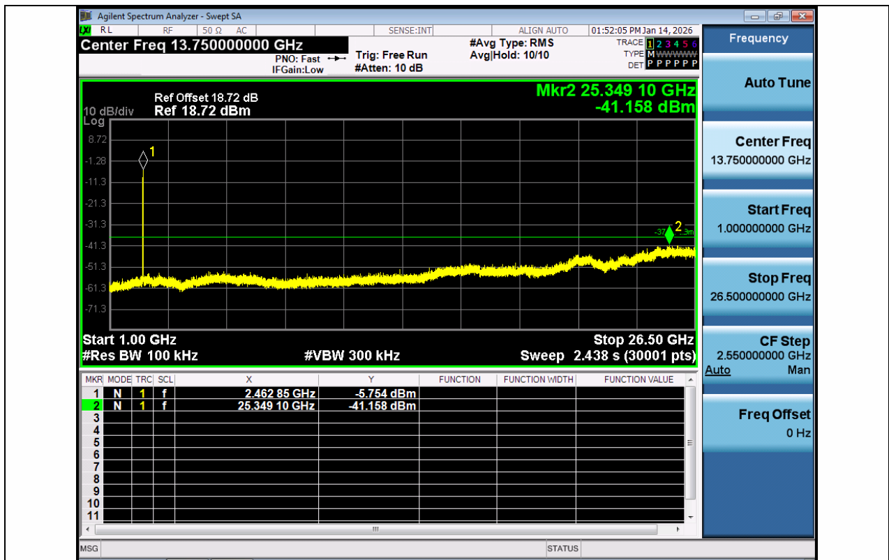
11G-Ant1-2457-1000~26500-PASS
