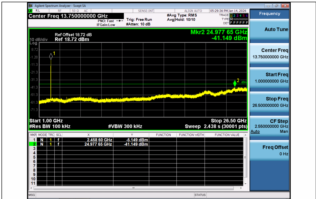
11AX20SISO-Ant1-2462-1000~26500-PASS
