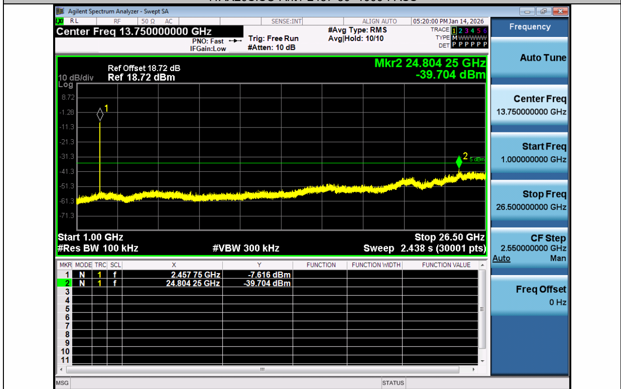
11AX20SISO-Ant1-2457-1000~26500-PASS
