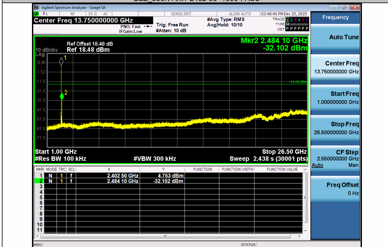
BLE_500K-Ant1-2402-1000~26500-PASS
