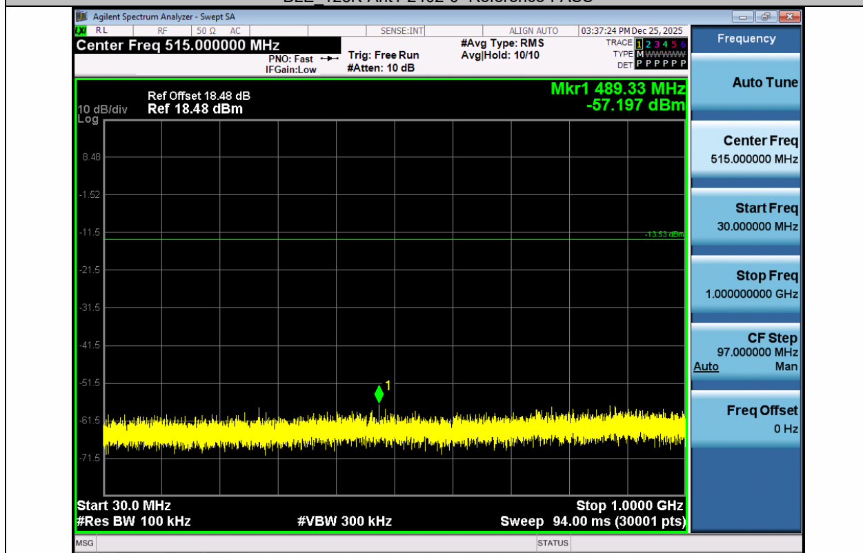
BLE_125K-Ant1-2402-30~1000-PASS
