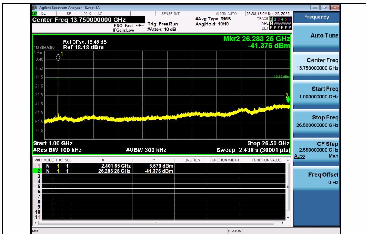
BLE_125K-Ant1-2402-1000~26500-PASS
