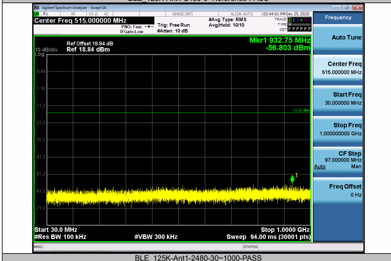
BLE_125K-Ant1-2480-30~1000-PASS
