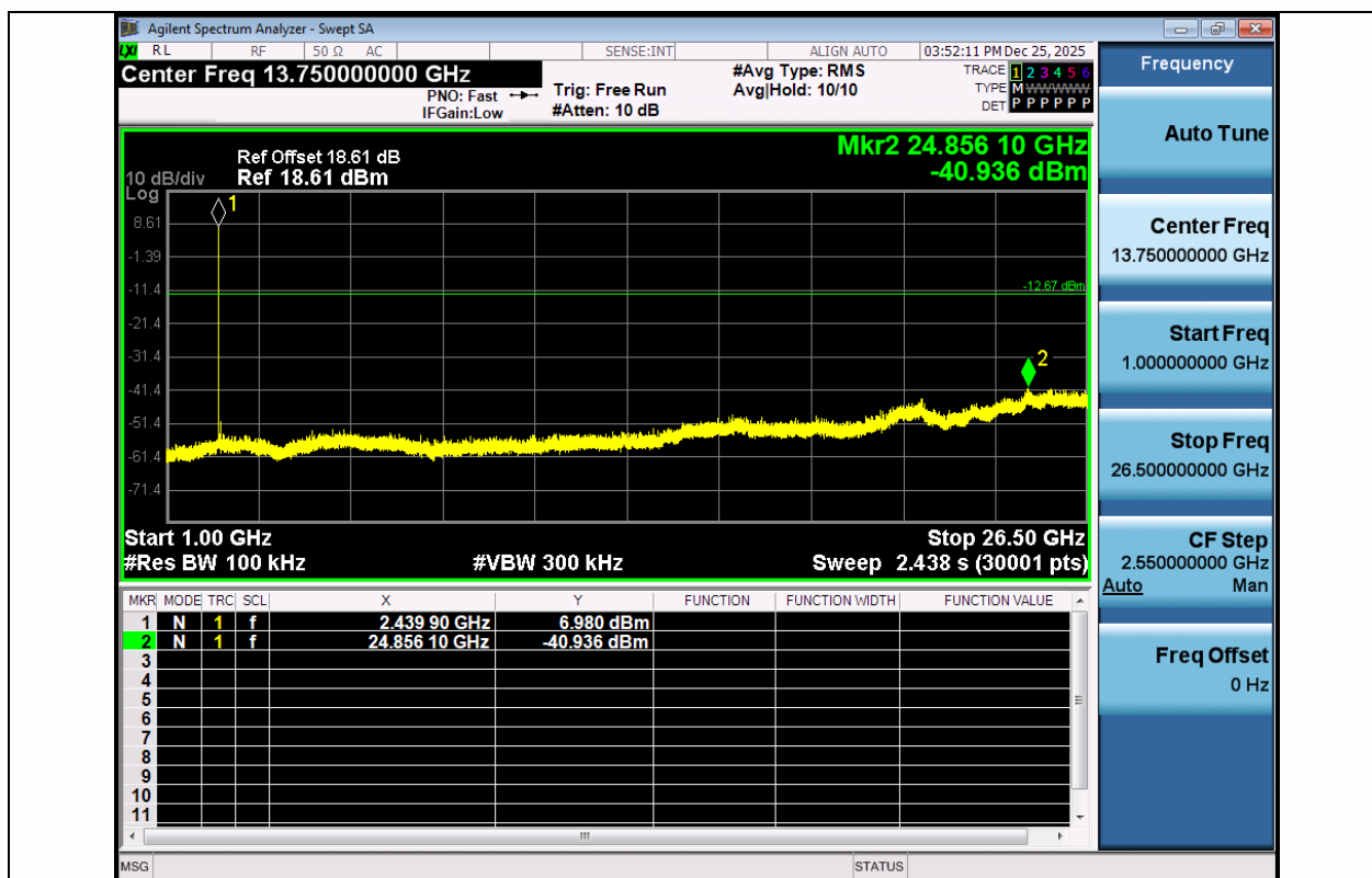
BLE_500K-Ant1-2440-1000~26500-PASS
