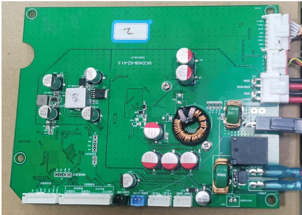
Power PCB view
