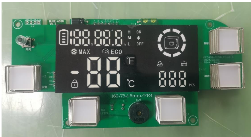
Control PCB view
