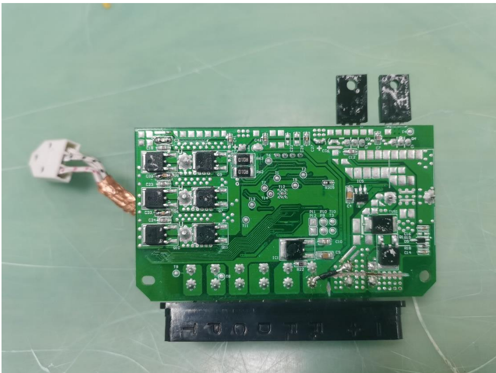
Compressor control PCB
