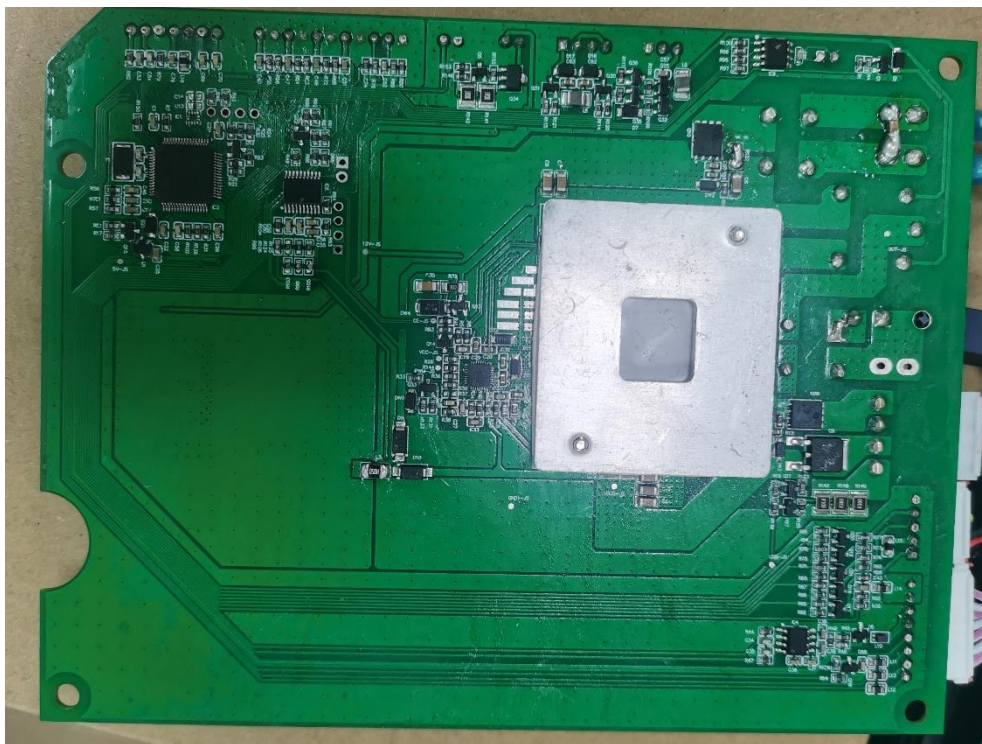
Power PCB view
