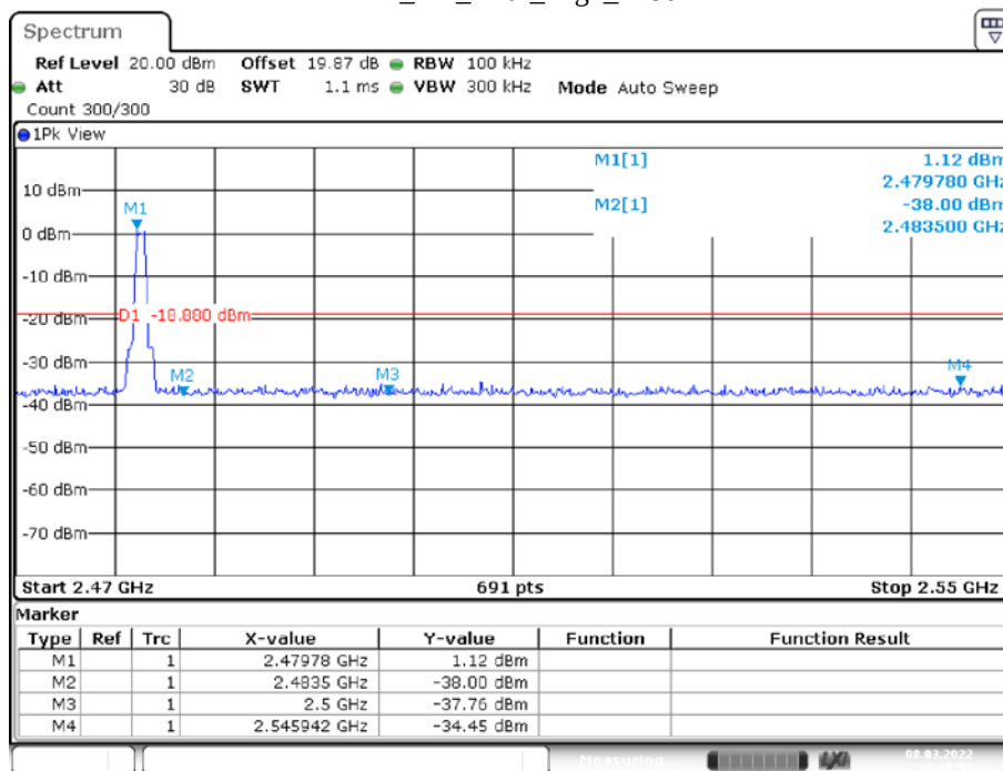
BLE_1M_Ant1_High_2480
