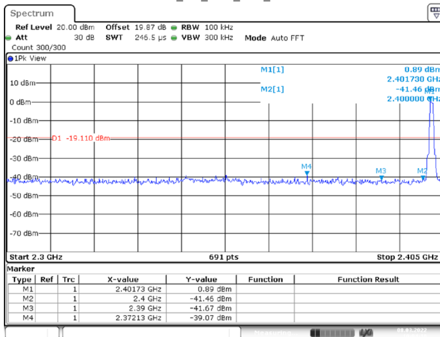
BLE_1M_Ant1_Low_2402
