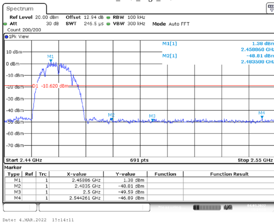
11B_Ant1_High_2462
