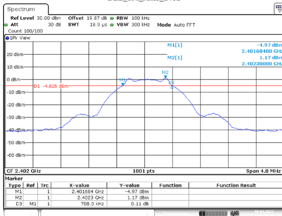
BLE_1M_Ant1_2402
