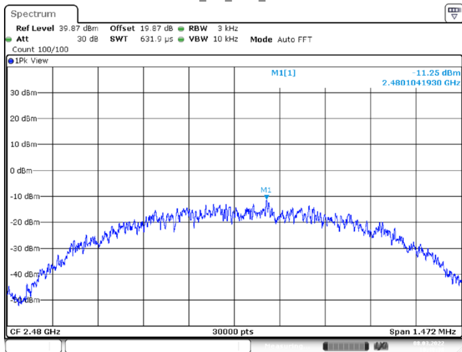
BLE_1M_Ant1_2480
