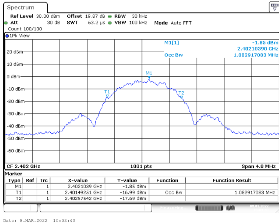
BLE_1M_Ant1_2402
