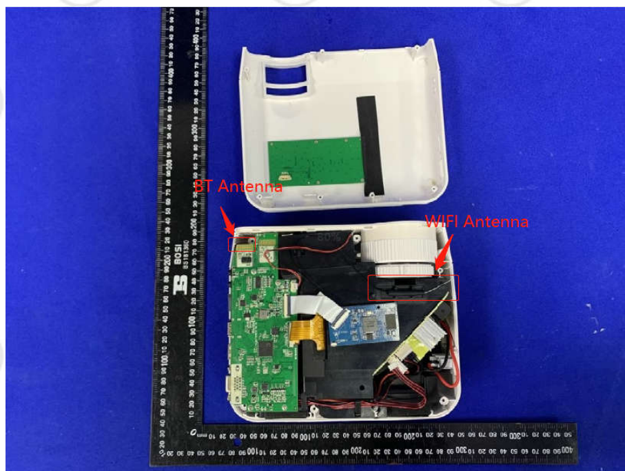
View of Product-24(Antenna)
