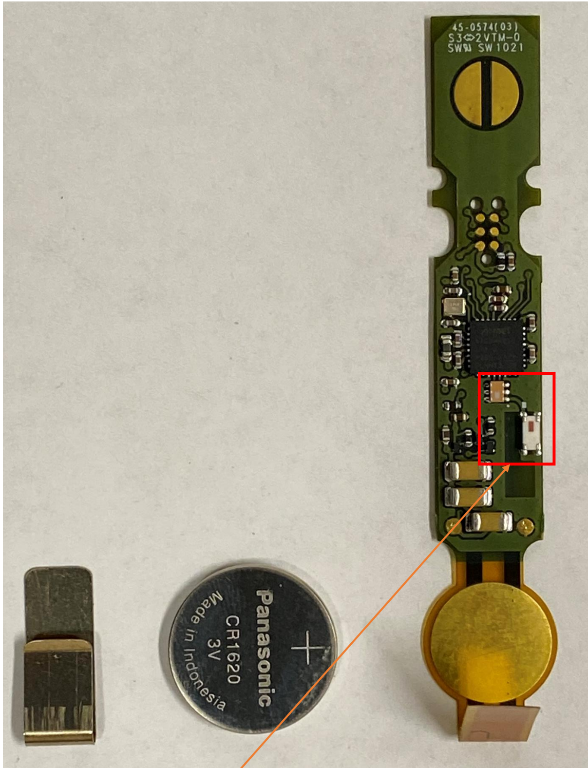
RF section: Antenna chip AE1 and Balun B1
