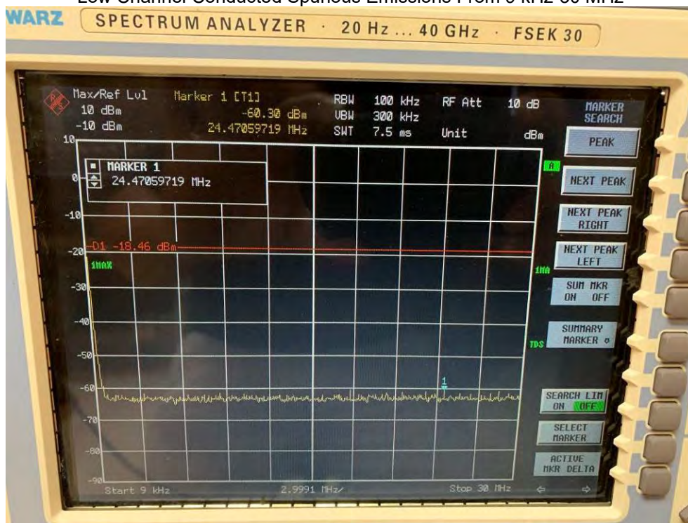
Low Channel Conducted Spurious Emissions From 9 kHz-30 MHz
