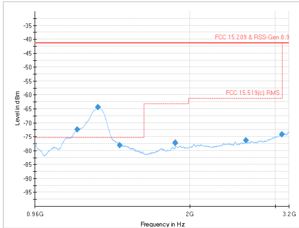
Plot 25: 960 MHz to 3.2 GHz, UWB emissions are turned off
