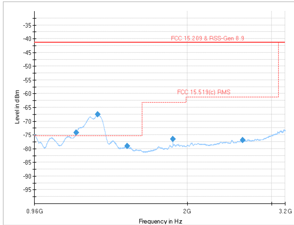
Plot 12: 960 MHz to 3.2 GHz, UWB test mode, Channel 2
