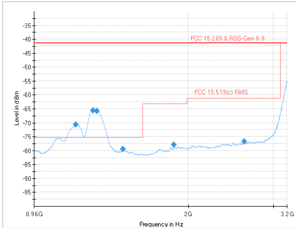
Plot 11: 960 MHz to 3.2 GHz, UWB test mode, Channel 1
