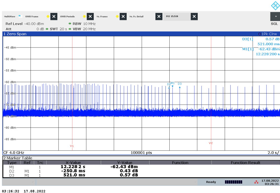
Plot 29: Emissions of the EUT, only at the beginning with associated receiver (Normal mode), Channel 2
