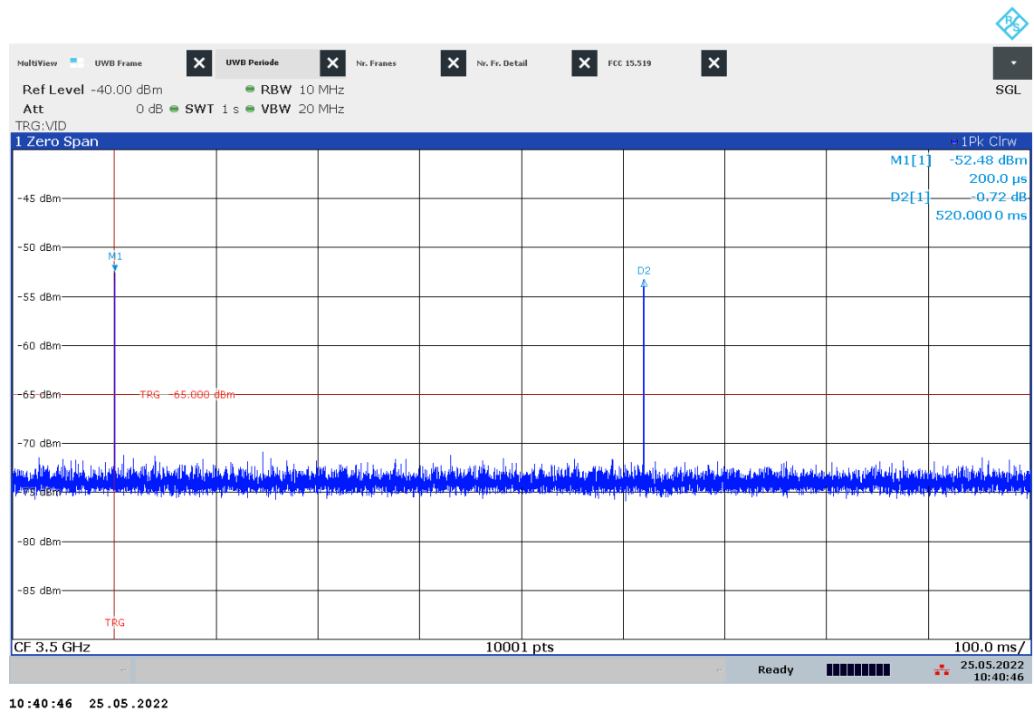
Plot 28: Emission of EUT without associated receiver (for comparison), normal mode, Channel 1
