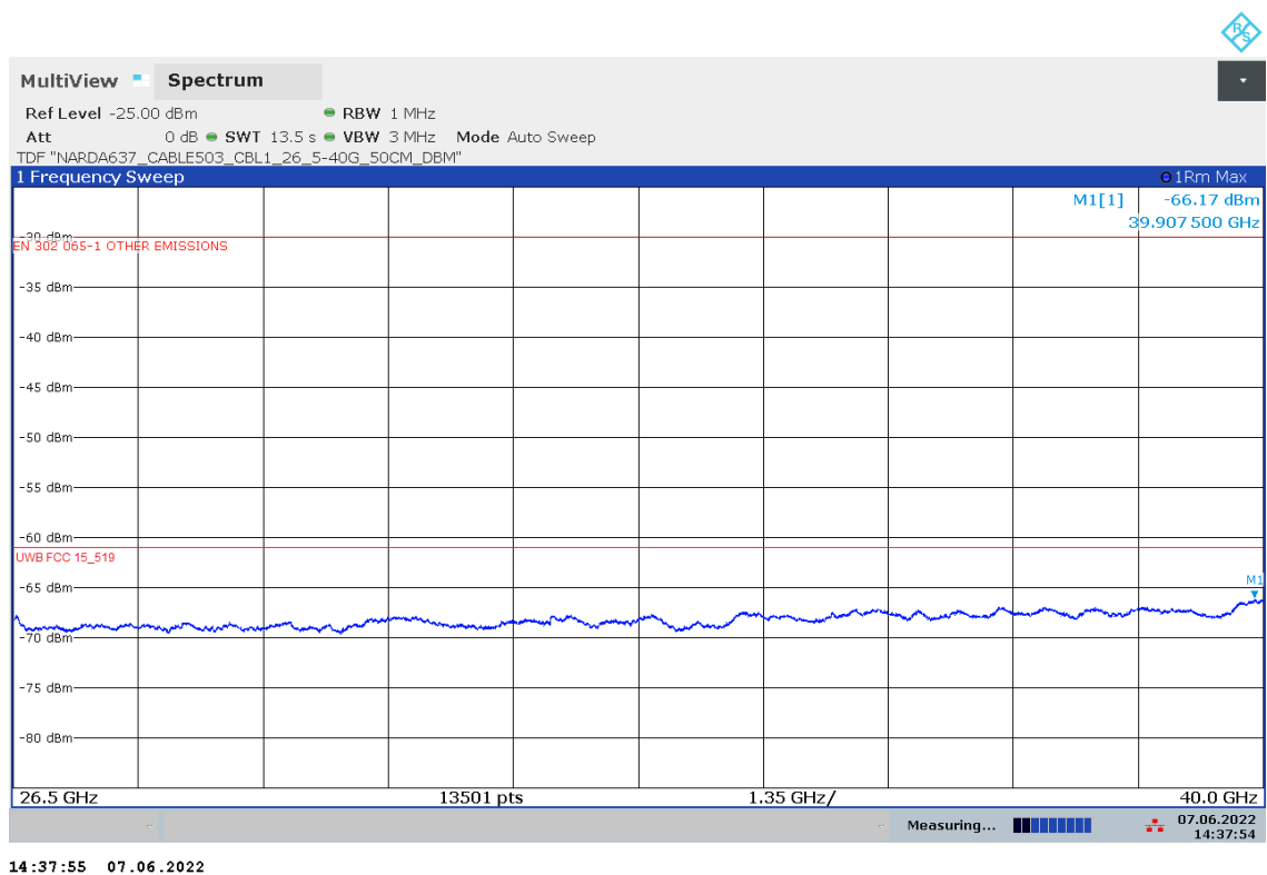
Plot 18: 26.5 GHz to 40.0 GHz, UWB test mode, Channel 1
