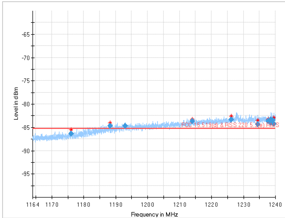
Plot 26: 1164 MHz to 1240 MHz, UWB emissions are turned off
