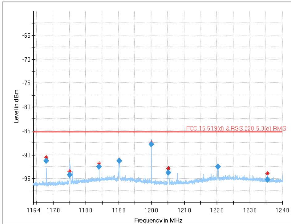
Plot 33: 1164 MHz to 1240 MHz GPS lower band UWB test mode channel 5
