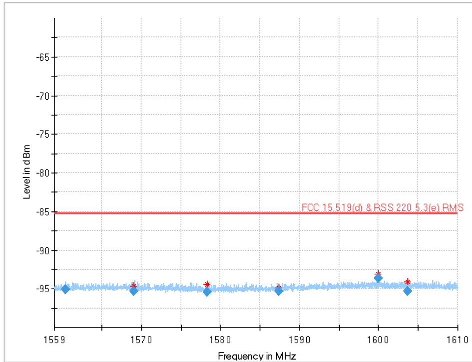
Plot 34: 1559 MHz to 1610 MHz GPS upper band, UWB test mode channel 1
