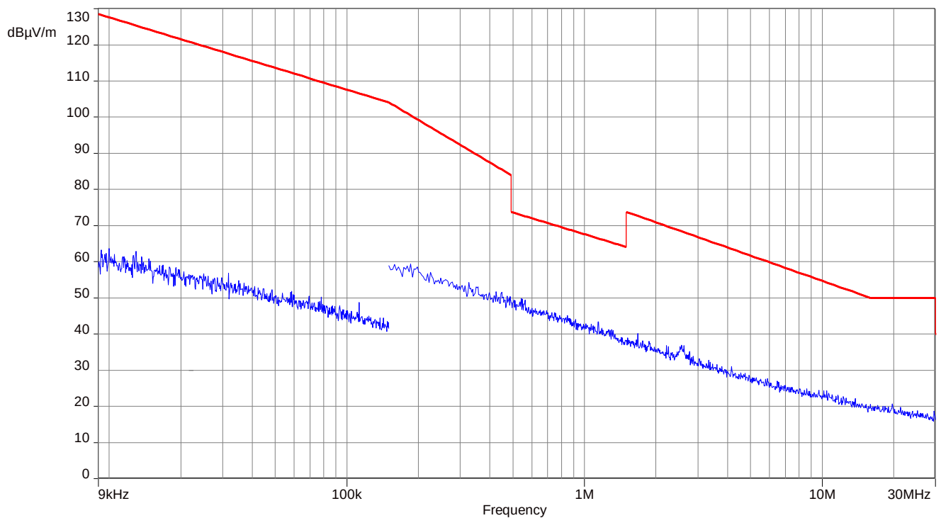
Plot 11: 9 kHz to 30 MHz, UWB test mode channel 2
