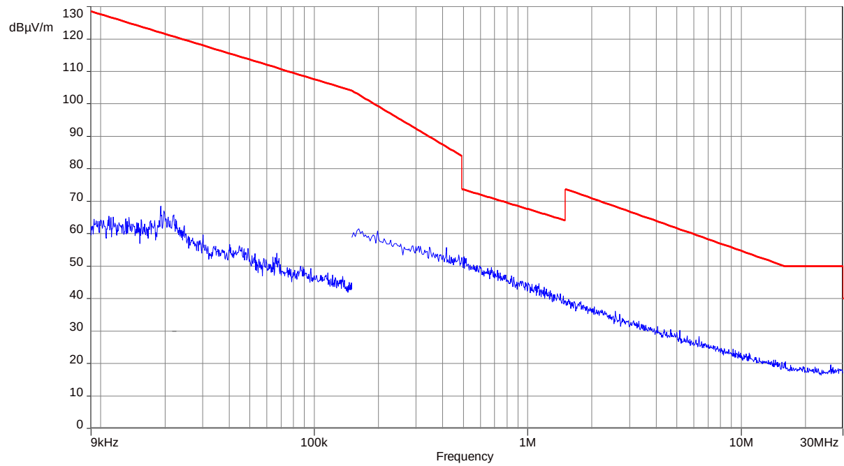
Plot 12: 9 kHz to 30 MHz, UWB test mode channel 5
