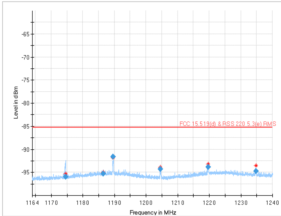
Plot 32: 1164 MHz to 1240 MHz GPS lower band, UWB test mode channel 2
