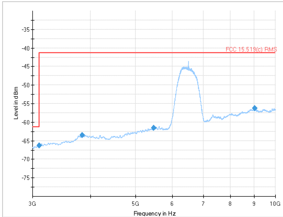
Plot 21: 3 GHz to 10 GHz, UWB test mode channel 5
