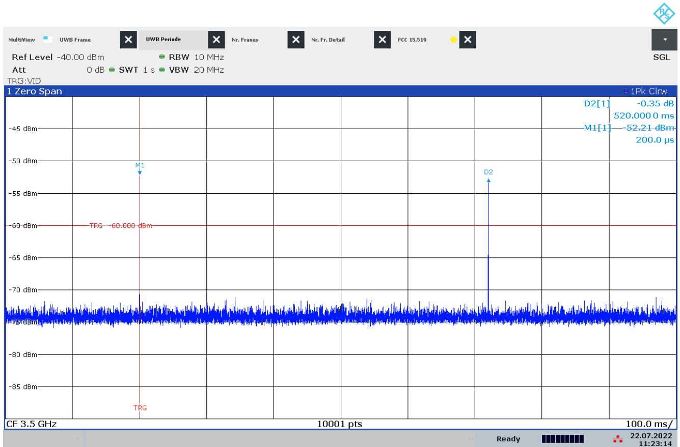
Plot 38: Emission of EUT without associated receiver (for comparison), normal mode, channel 1
