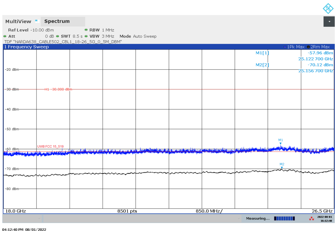
Plot 26: 18 GHz to 26.5 GHz, UWB test mode channel 2
