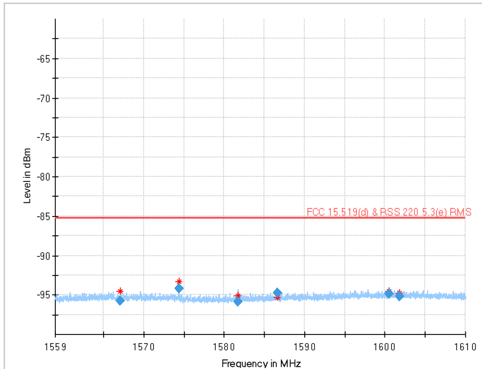
Plot 35: 1559 MHz to 1610 MHz GPS upper band UWB test mode channel 2
