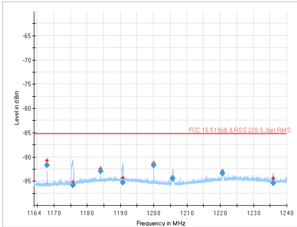
Plot 31: 1164 MHz to 1240 MHz GPS lower band, UWB test mode channel 1
