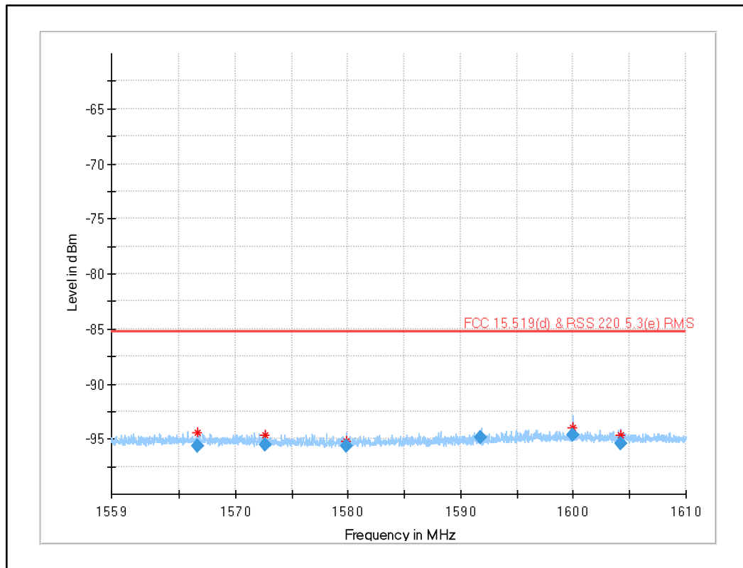
Plot 36: 1559 MHz to 1610 MHz GPS upper band UWB test mode channel 5
