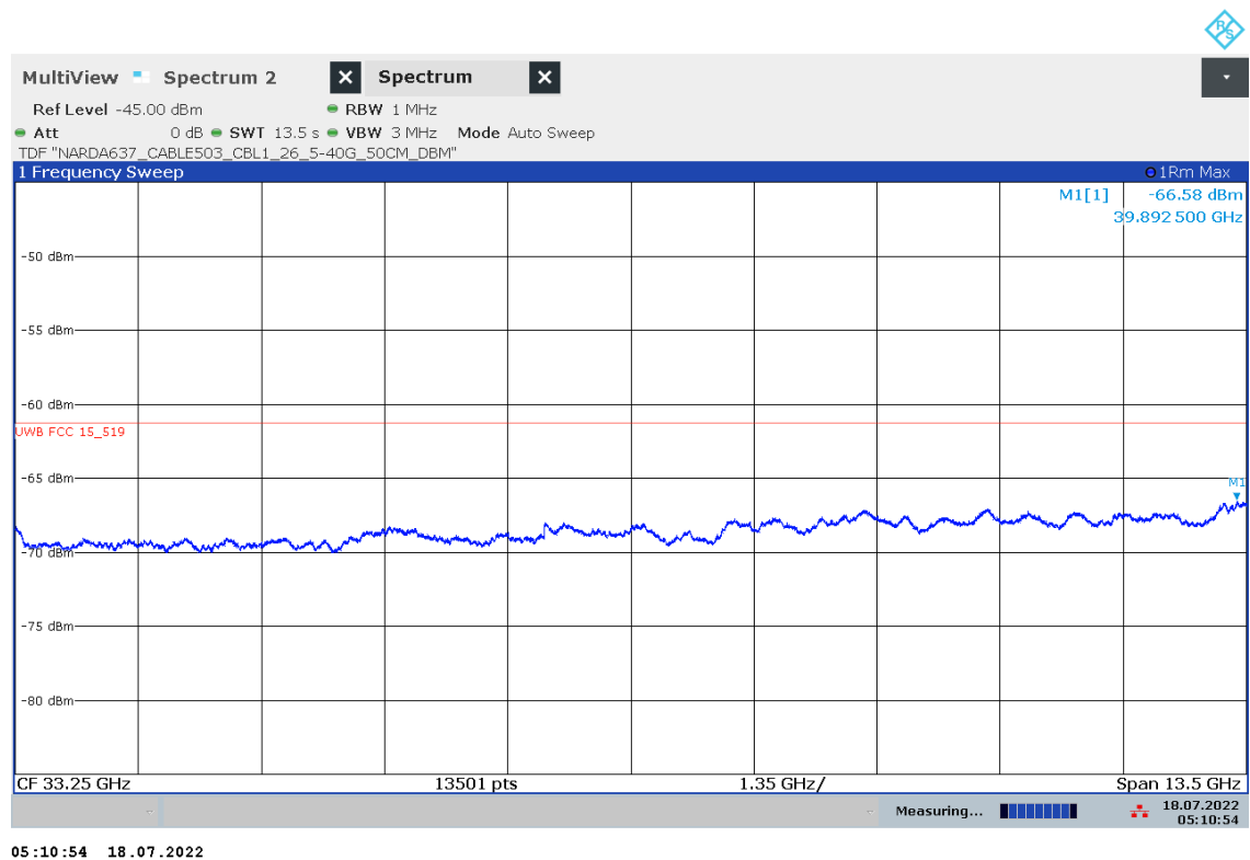
Plot 28: 26.5 GHz to 40.0 GHz, UWB test mode channel 1
