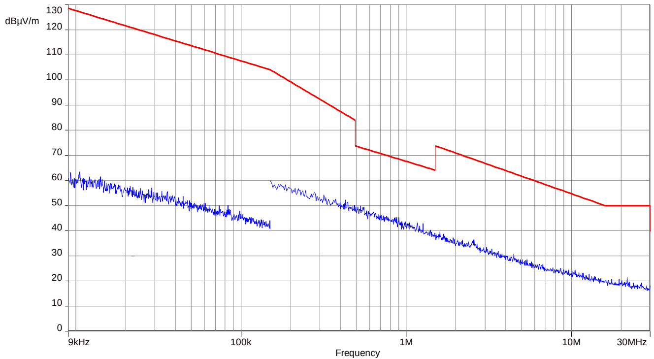
Plot 10: 9 kHz to 30 MHz, UWB test mode channel 1
