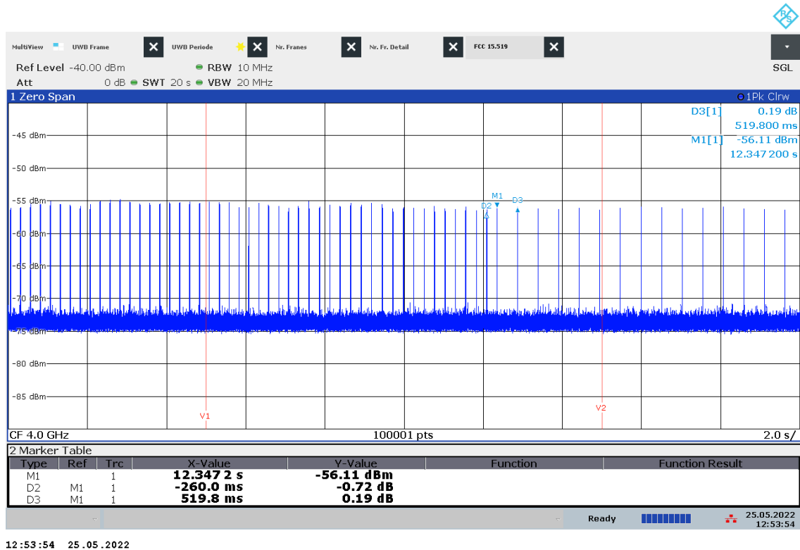
Plot 39: Emissions of the EUT, only at the beginning with associated receiver (Normal mode), channel 2
