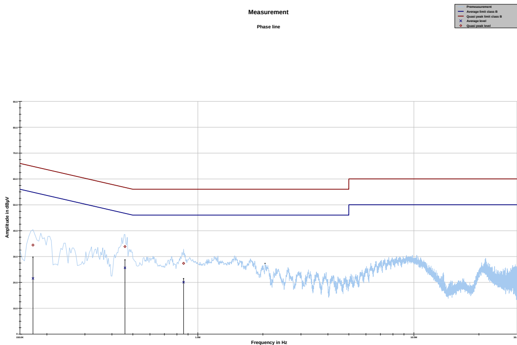
Plot 42: Phase line
