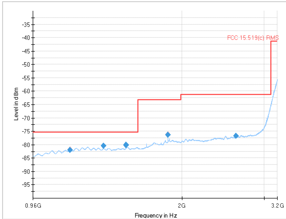
Plot 11: 960 MHz to 3.2 GHz (Limit acc. to §15.519 (c)), UWB test mode, Channel 1
