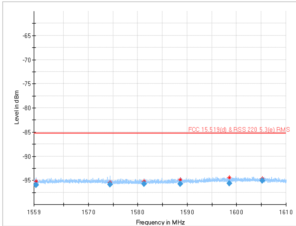
Plot 23: 1559 MHz to 1610 MHz (§15.519 (d)), UWB test mode, Channel 1
