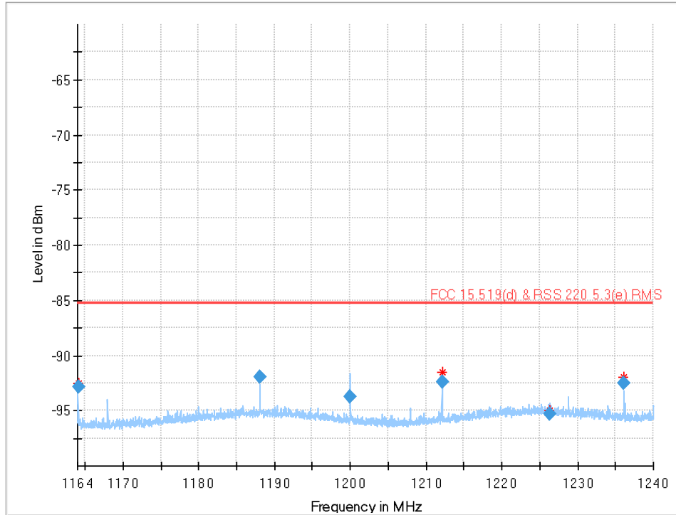
Plot 22: 1164 MHz to 1240 MHz (§15.519 (d)), UWB test mode, Channel 2
