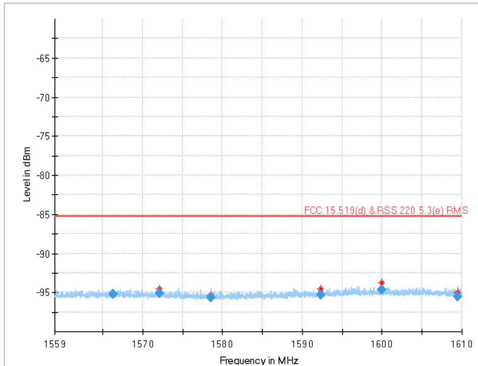
Plot 24: 1559 MHz to 1610 MHz (§15.519 (d)), UWB test mode, Channel 2
