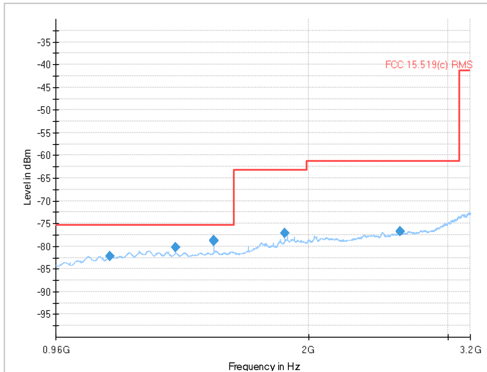
Plot 12: 960 MHz to 3.2 GHz (Limit acc. to §15.519 (c)), UWB test mode, Channel 2
