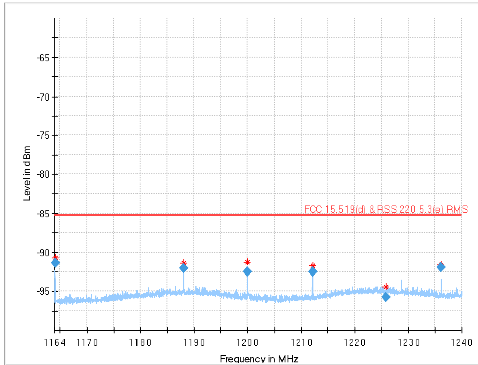
Plot 21: 1164 MHz to 1240 MHz (§15.519 (d)), UWB test mode, Channel 1
