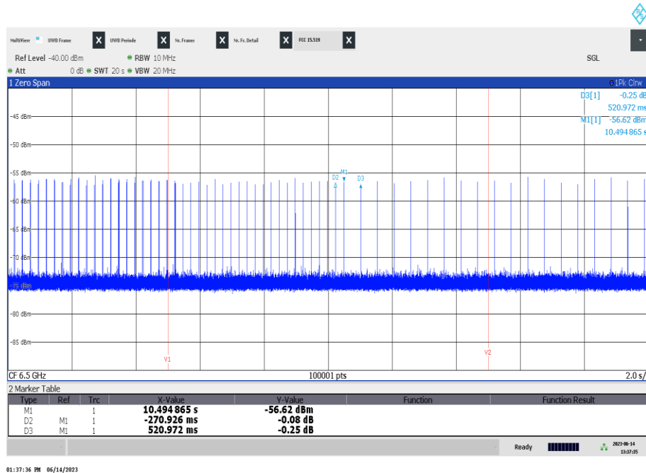
Plot 40: Emissions of the EUT, only at the beginning with associated receiver (Normal mode), channel 5
