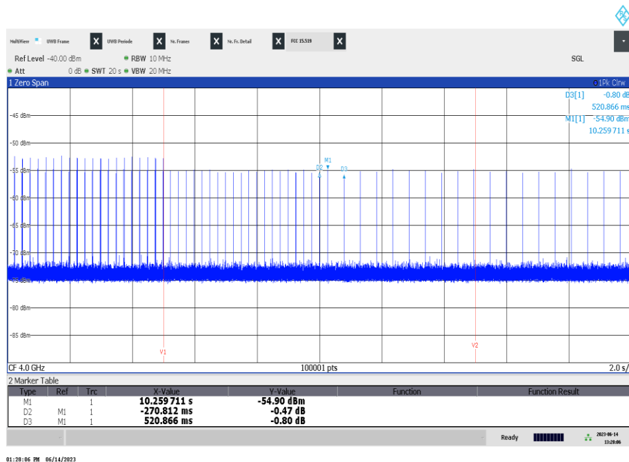
Plot 39: Emissions of the EUT, only at the beginning with associated receiver (Normal mode), channel 2
