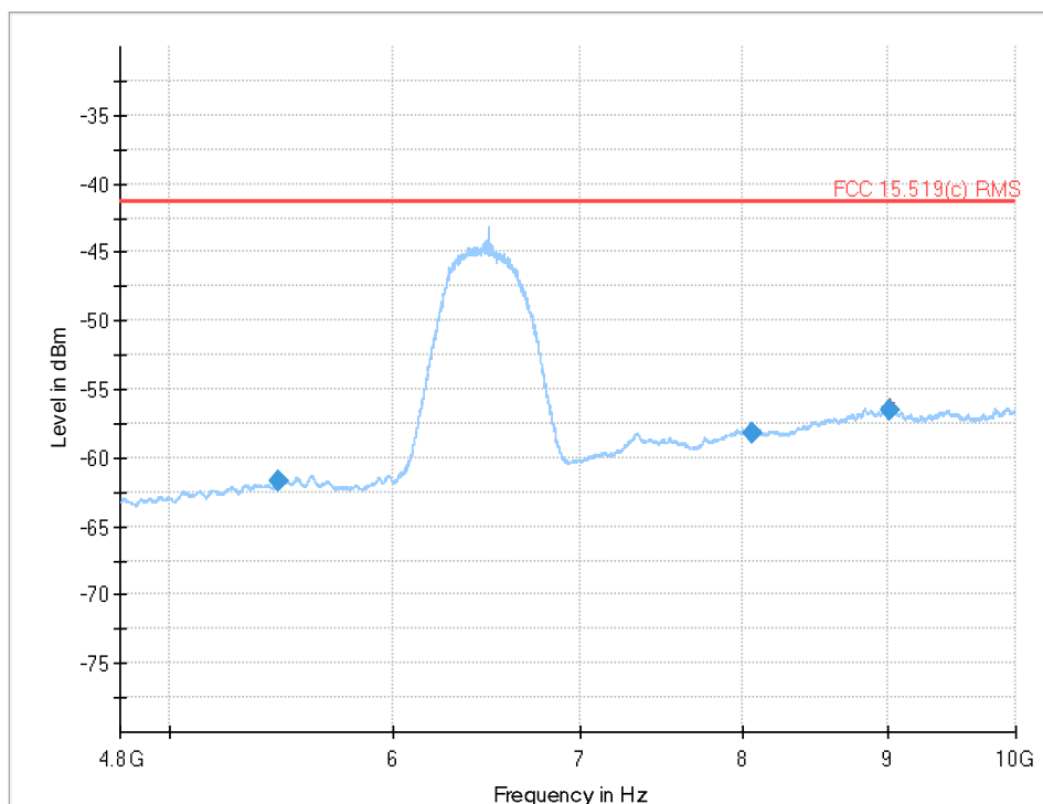
Plot 21: 4.8 GHz to 10 GHz, UWB test mode channel 5
