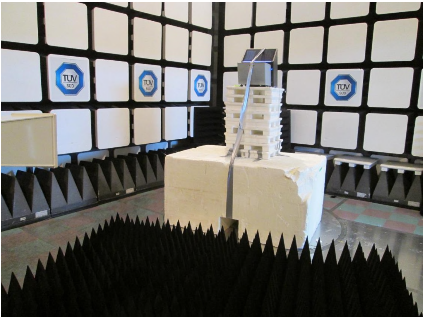
Test setup photo 4 Radiated measurements, 6 GHz – 10 GHz
