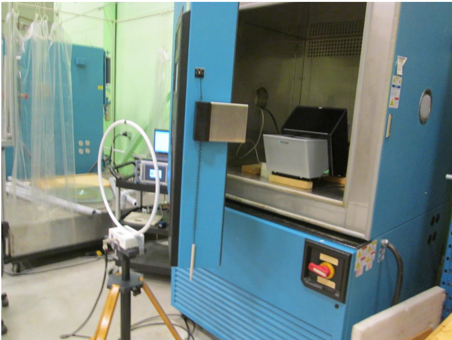
Test setup photo 9 Frequency Stability at Extreme Temperatures
