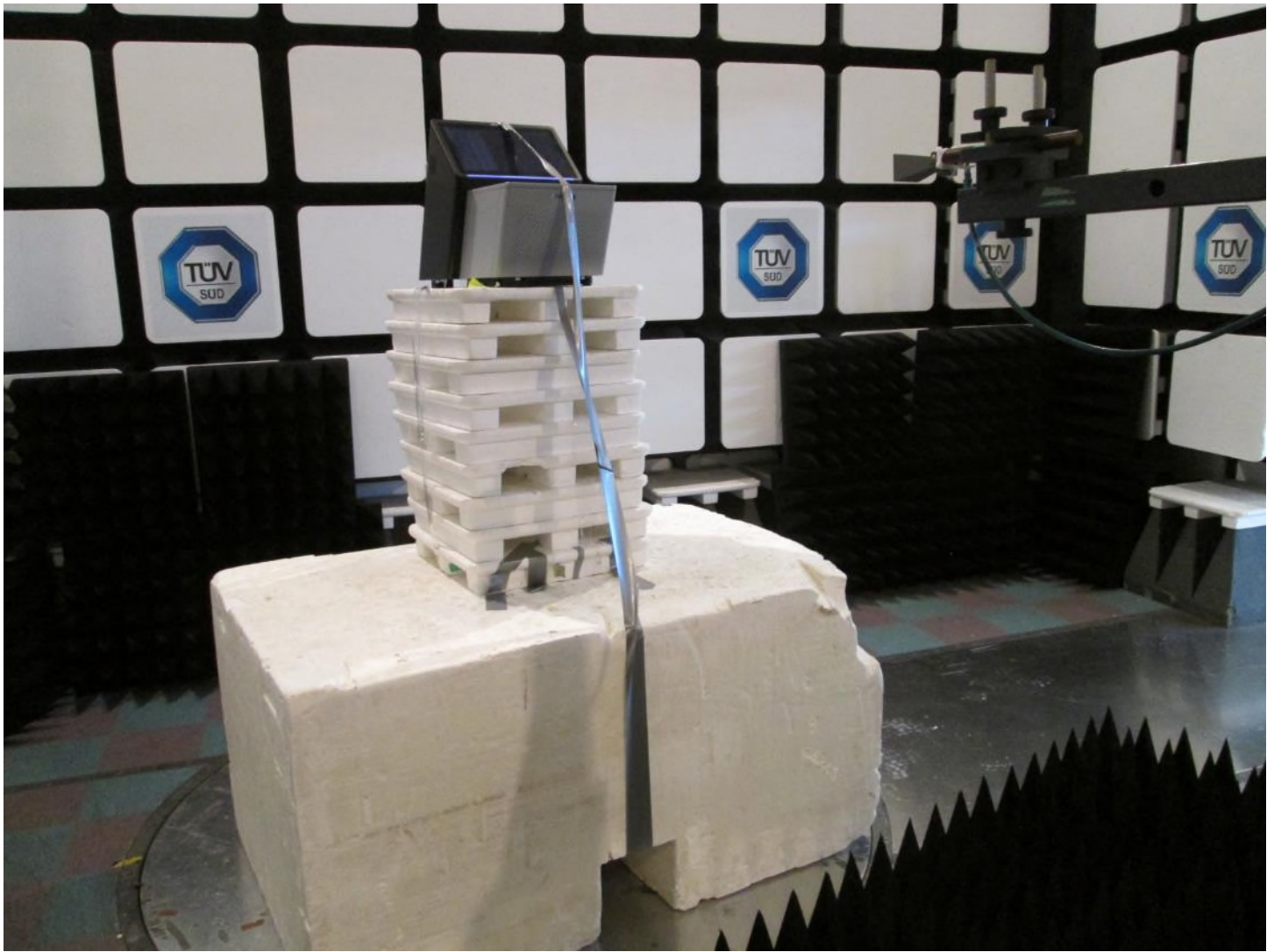
Test setup photo 6 Radiated measurements, 18 GHz – 26.5 GHz
