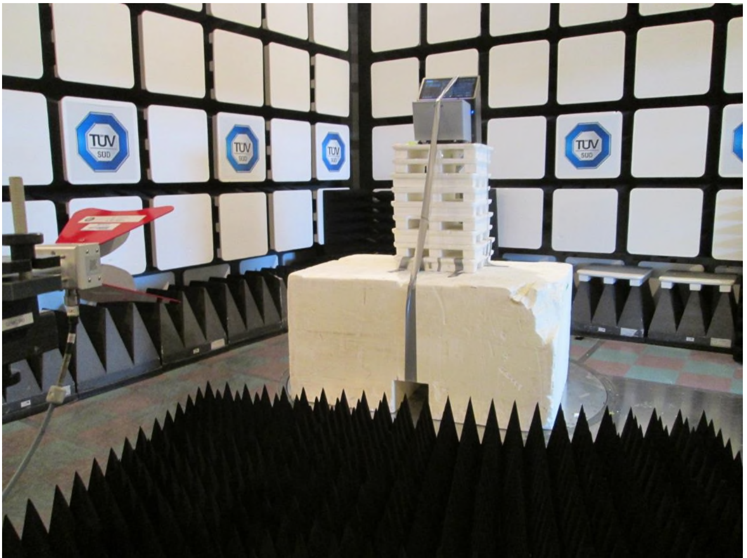
Test setup photo 3 Radiated measurements, 1 GHz – 6 GHz
