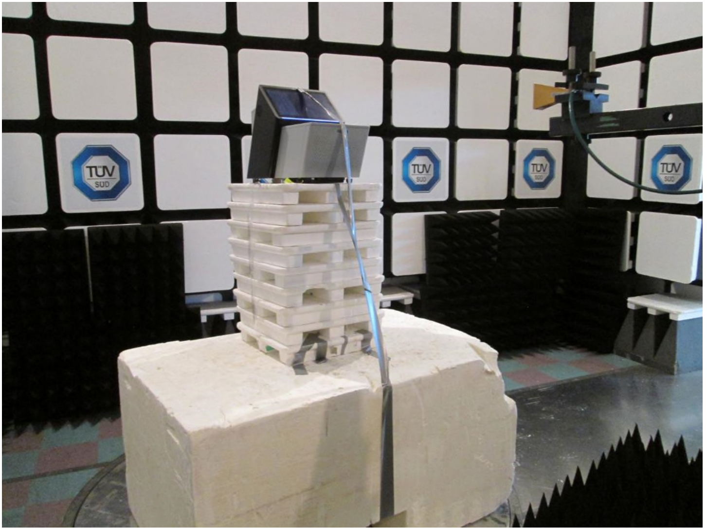
Test setup photo 7 Radiated measurements, 26.5 GHz – 40 GHz
