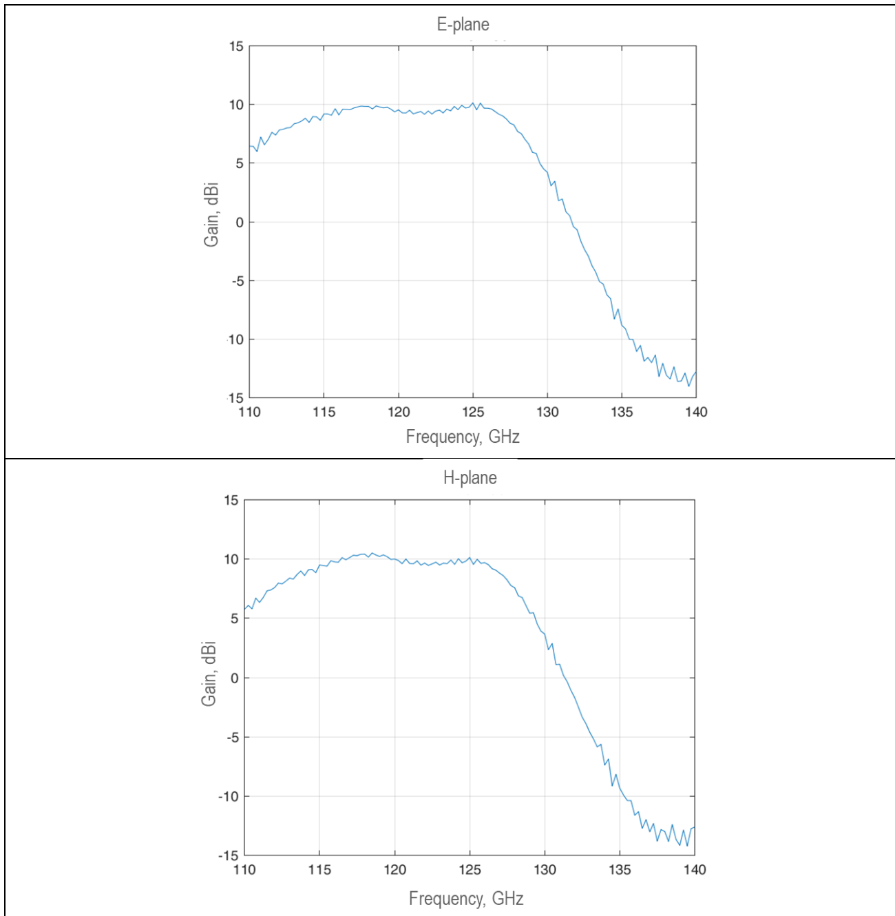
Figure 2 RX antenna gain vs frequency.
