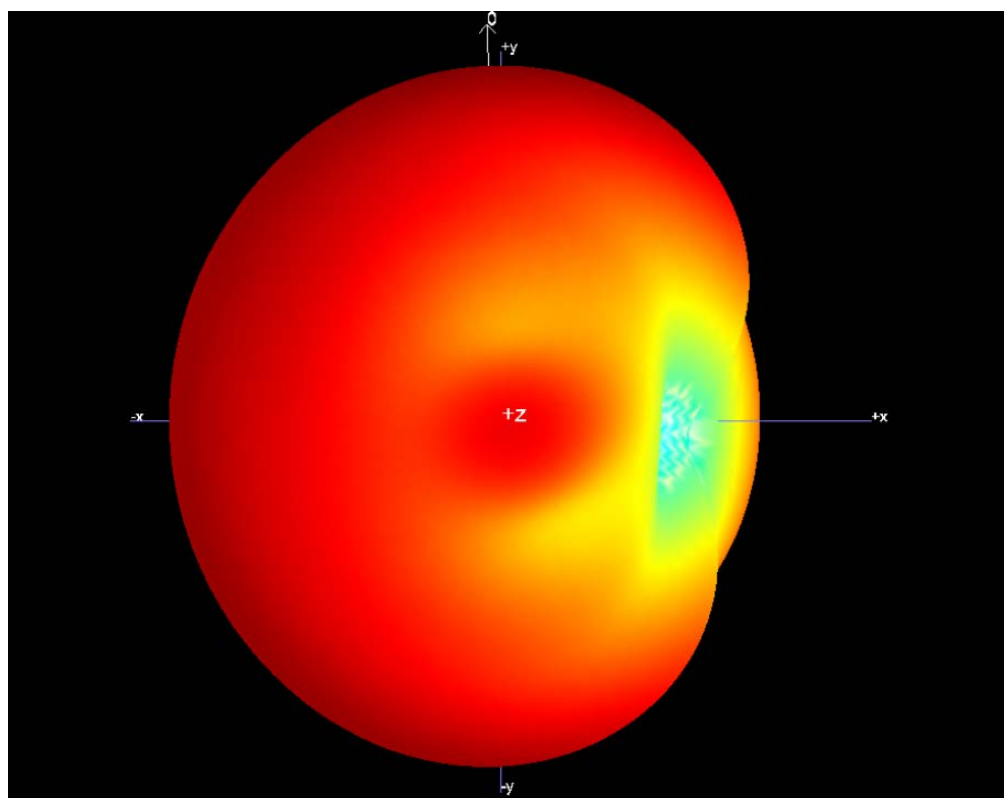
Frequency: 2800MHz
