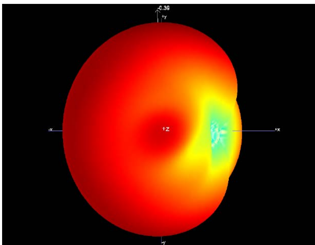
Frequency: 2500MHz
