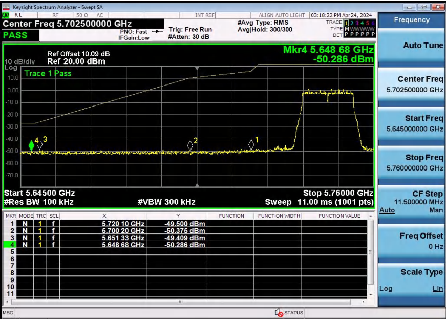
11N20SISO-5745-PASS
