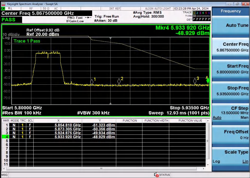
11N20SISO-5825-PASS
