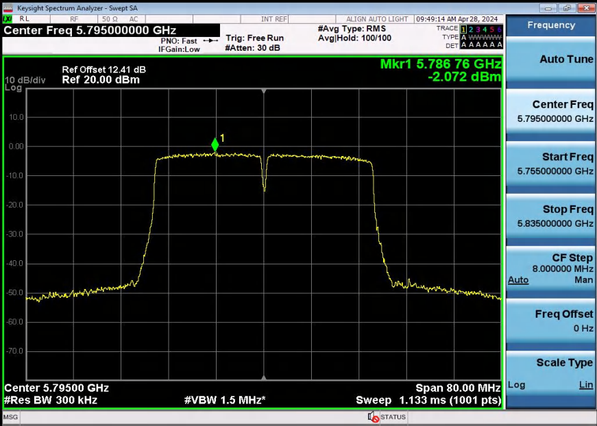
11AC40SISO-5795-PASS
