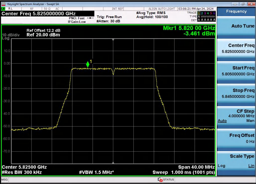
11A-5825-PASS
