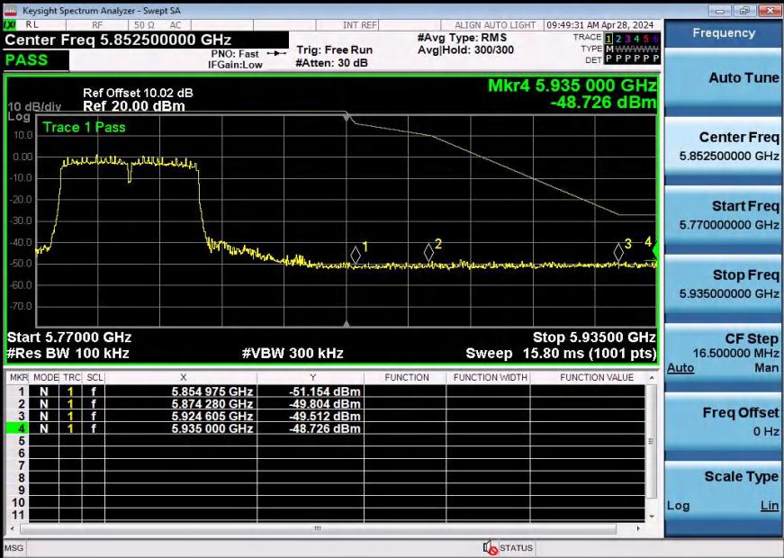
11AC40SISO-5795-PASS
