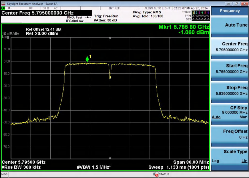
11N40SISO-5795-PASS
