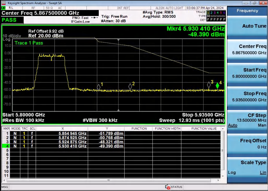
11A-5825-PASS
