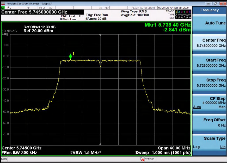
11AC20SISO-5745-PASS
