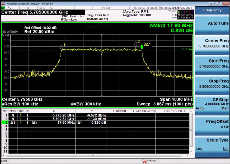
11AC20SISO-5785-PASS
