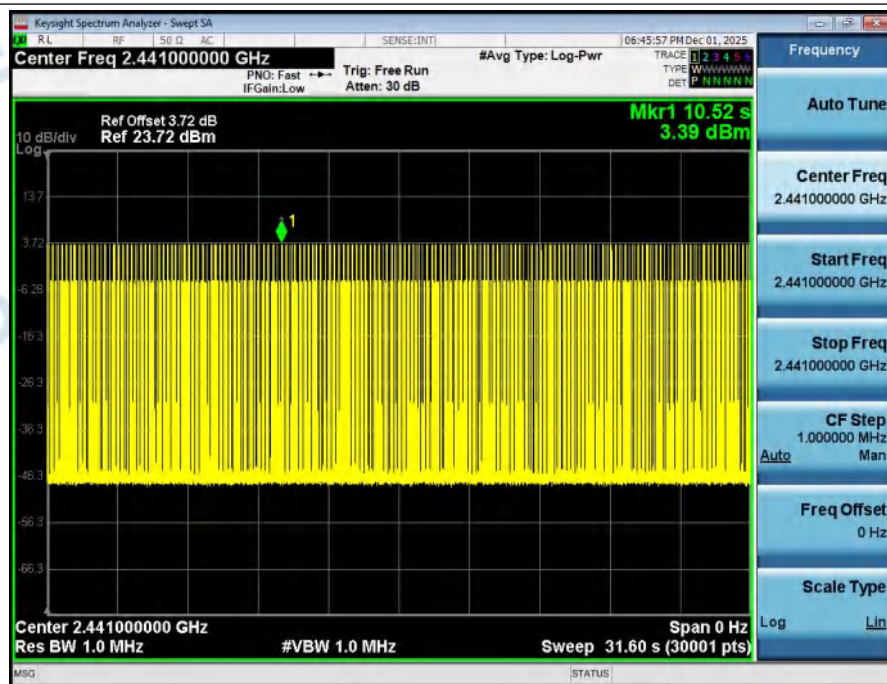
Dwell_Time_(Hopping)_NVNT_ANT1_3-DH3_2441_00_One_Burst_Time
