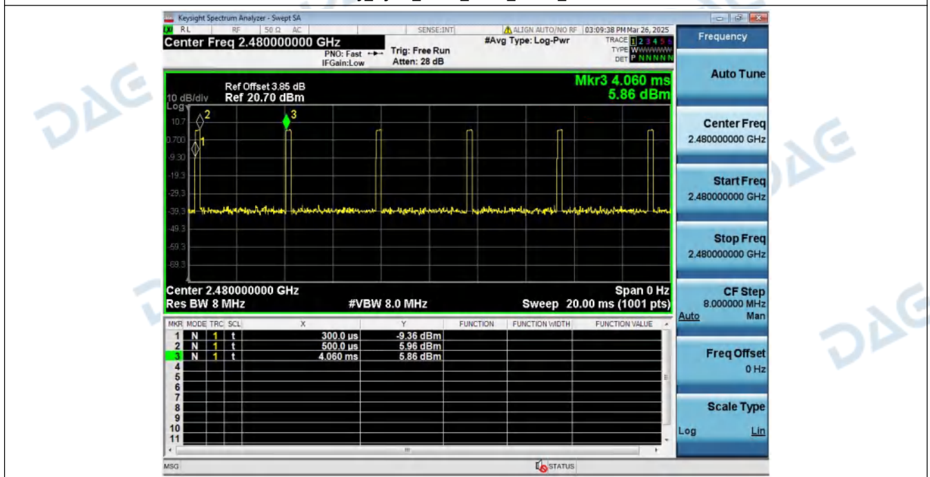
Duty_Cycle_NVNT_ANT1_3-DH5_2480
