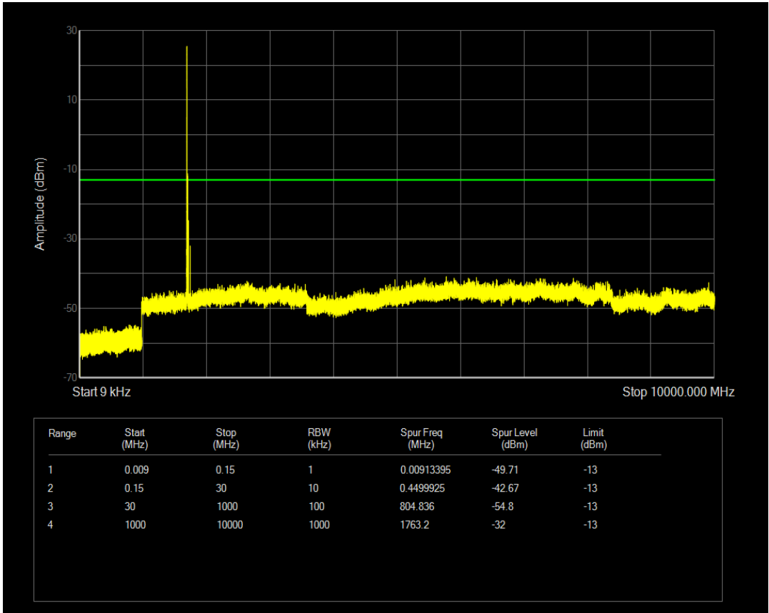
Band4 QPSK BW=1.4MHz Channel=20175 RB Size=1 Position=#Mid
