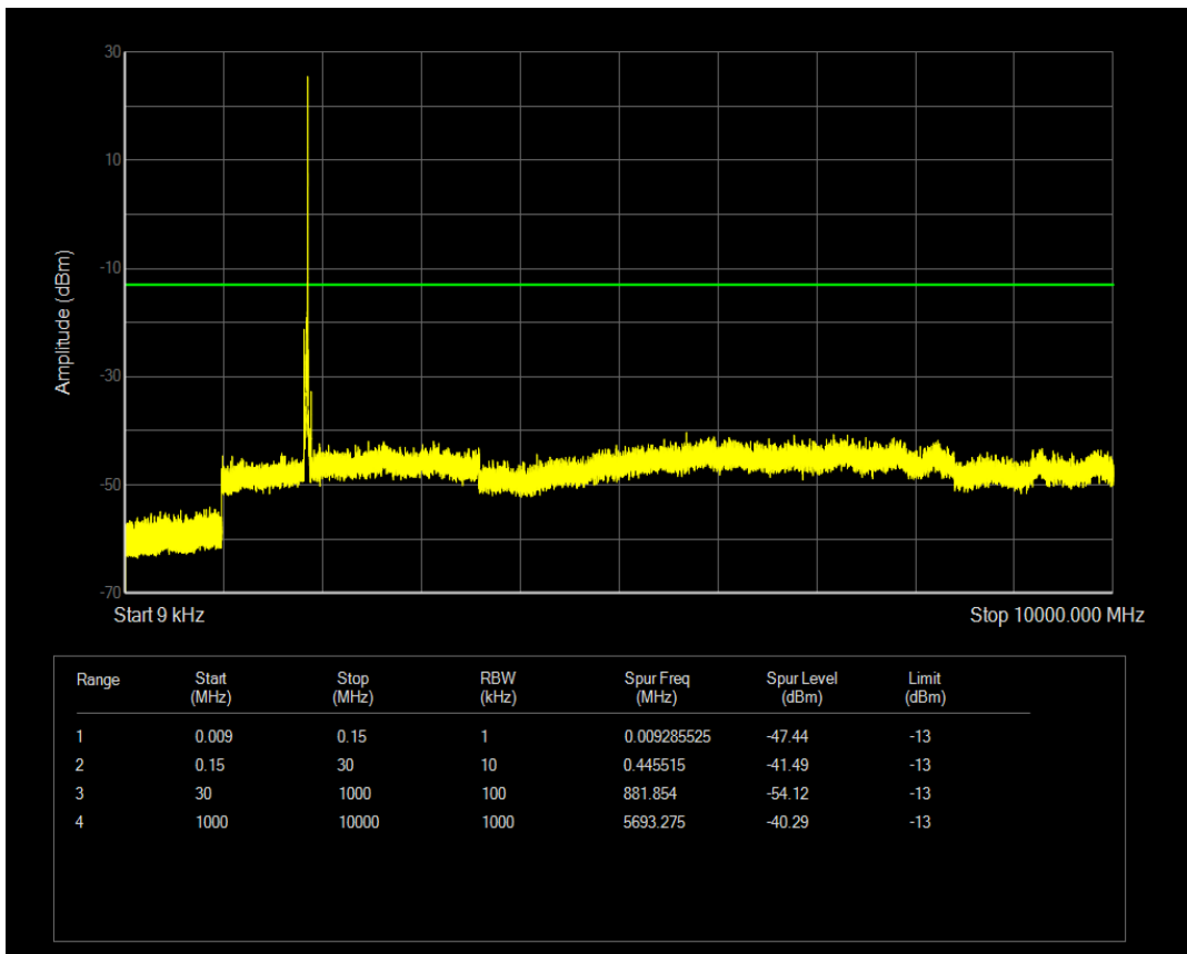
Band2 QPSK BW=20MHz Channel=18700 RB Size=50 Position=#0
