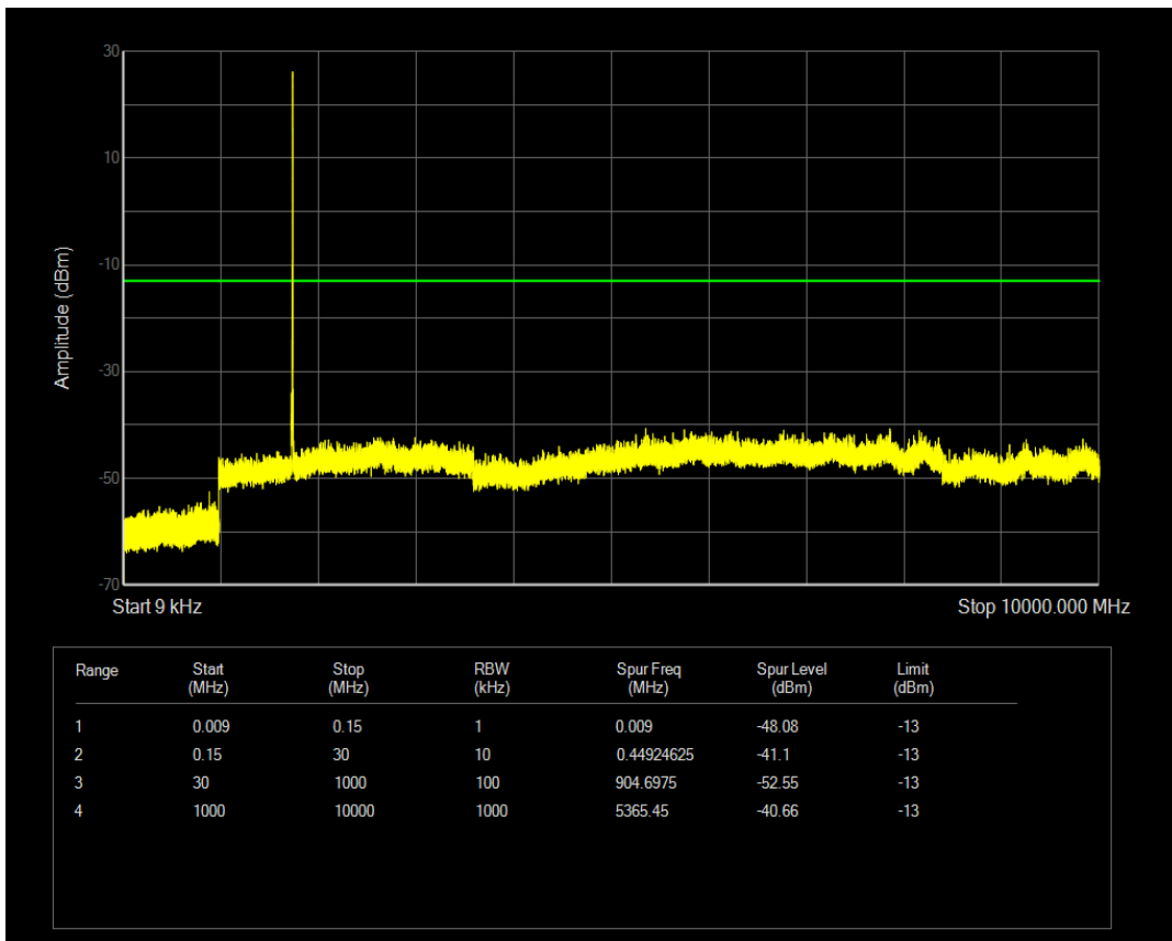
Band4 QAM16 BW=3MHz Channel=20385 RB Size=8 Position=#0
