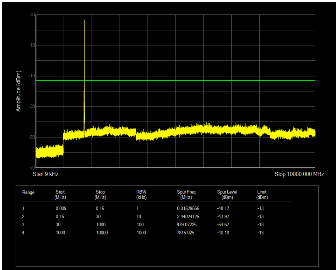
Band4 QAM16 BW=10MHz Channel=20350 RB Size=25 Position=#Max
