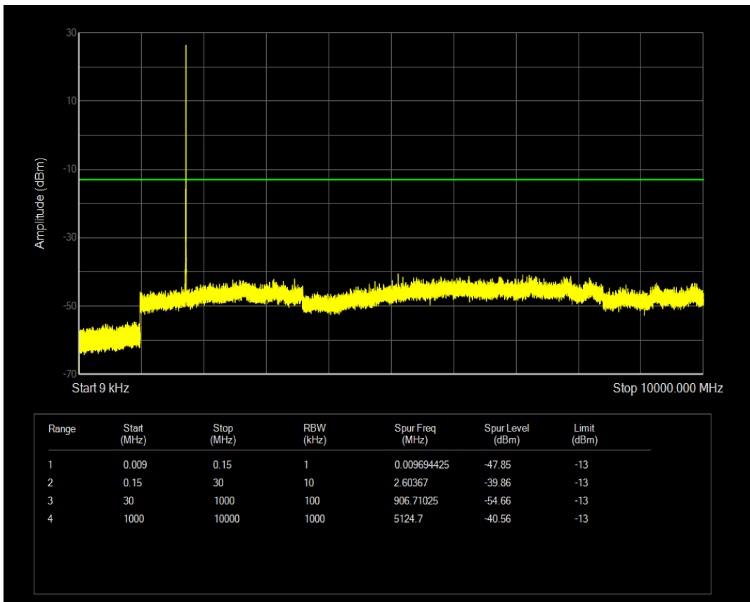
Band4 QPSK BW=3MHz Channel=20175 RB Size=8 Position=#Max
