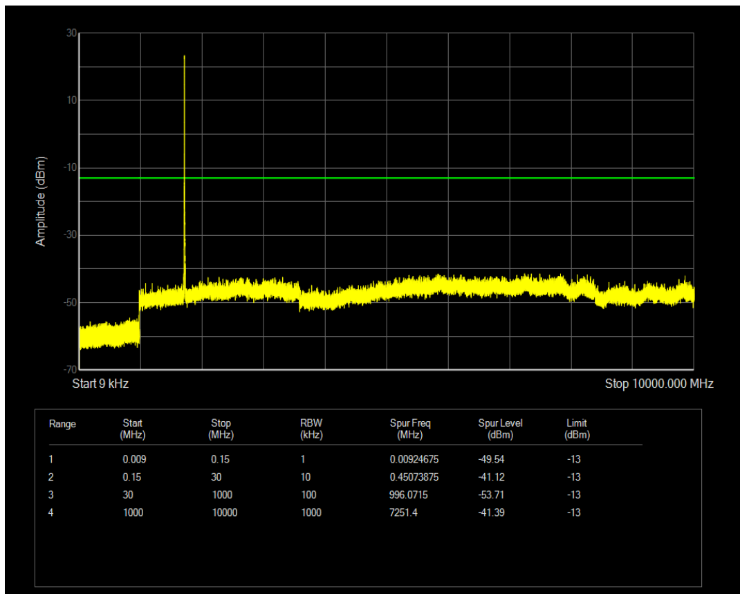
Band4 QAM16 BW=5MHz Channel=20175 RB Size=12 Position=#Max
