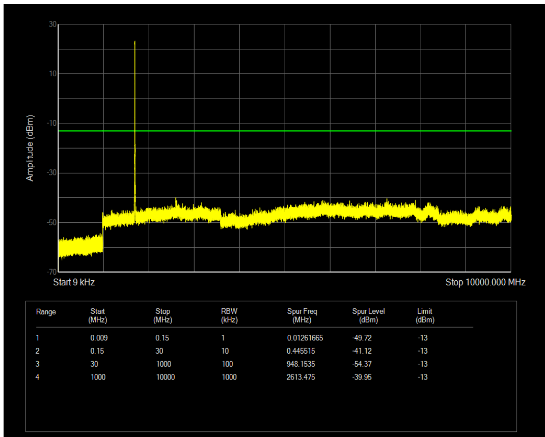
Band4 QAM16 BW=5MHz Channel=19975 RB Size=12 Position=#0
