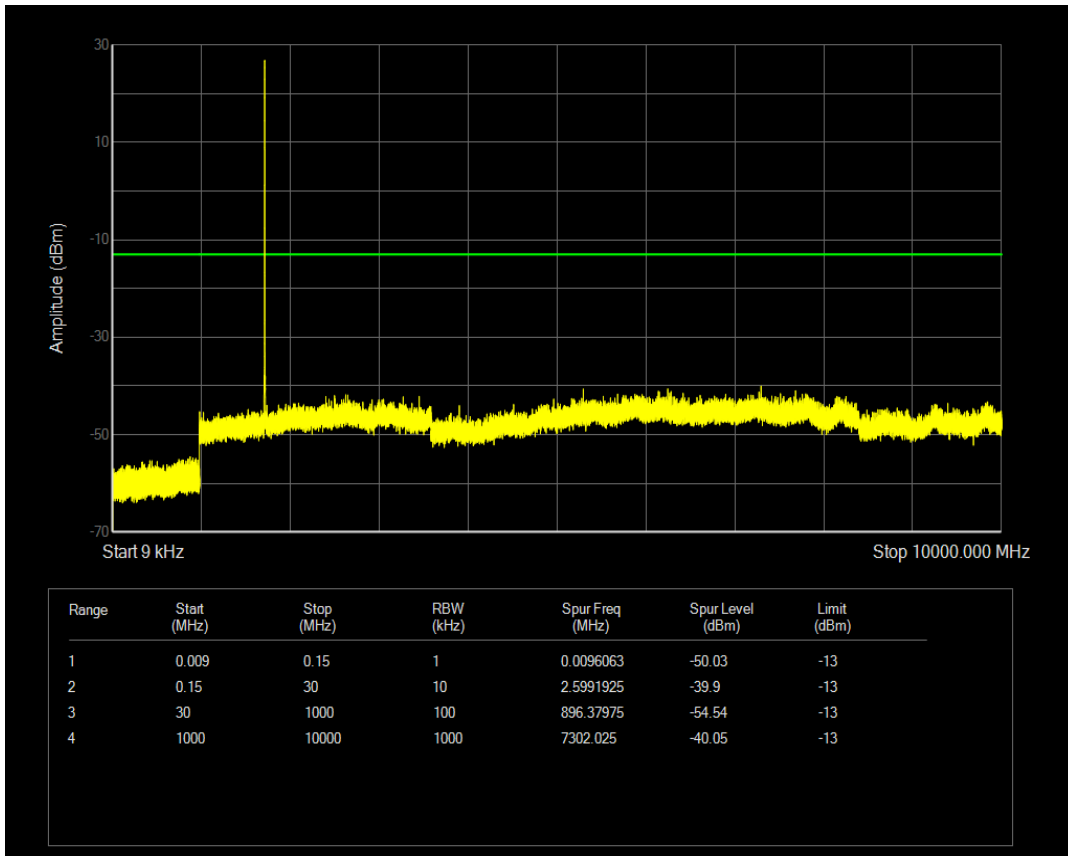
Band4 QPSK BW=3MHz Channel=20175 RB Size=1 Position=#Mid
