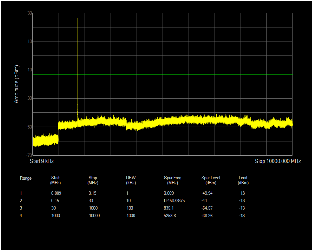
Band4 QAM16 BW=5MHz Channel=20375 RB Size=1 Position=#Mid
