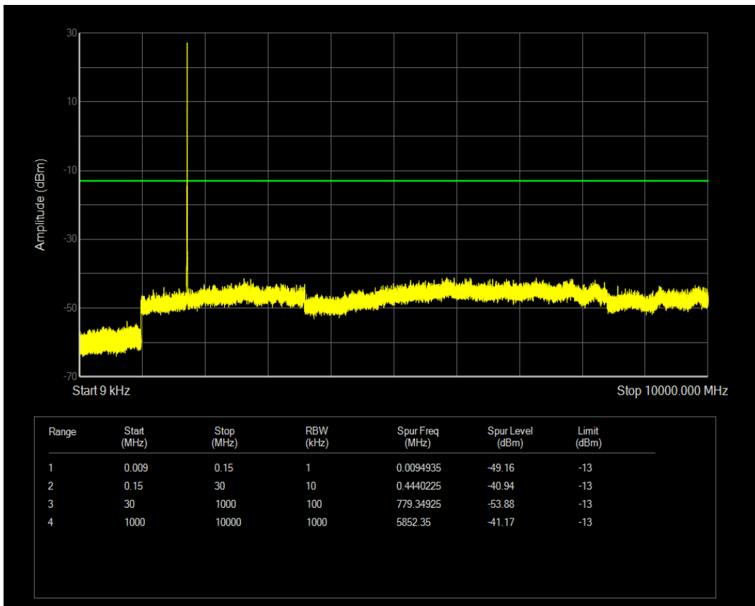
Band4 QAM16 BW=3MHz Channel=20175 RB Size=8 Position=#0
