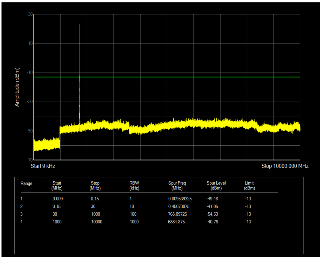
Band4 QAM16 BW=5MHz Channel=20375 RB Size=12 Position=#0
