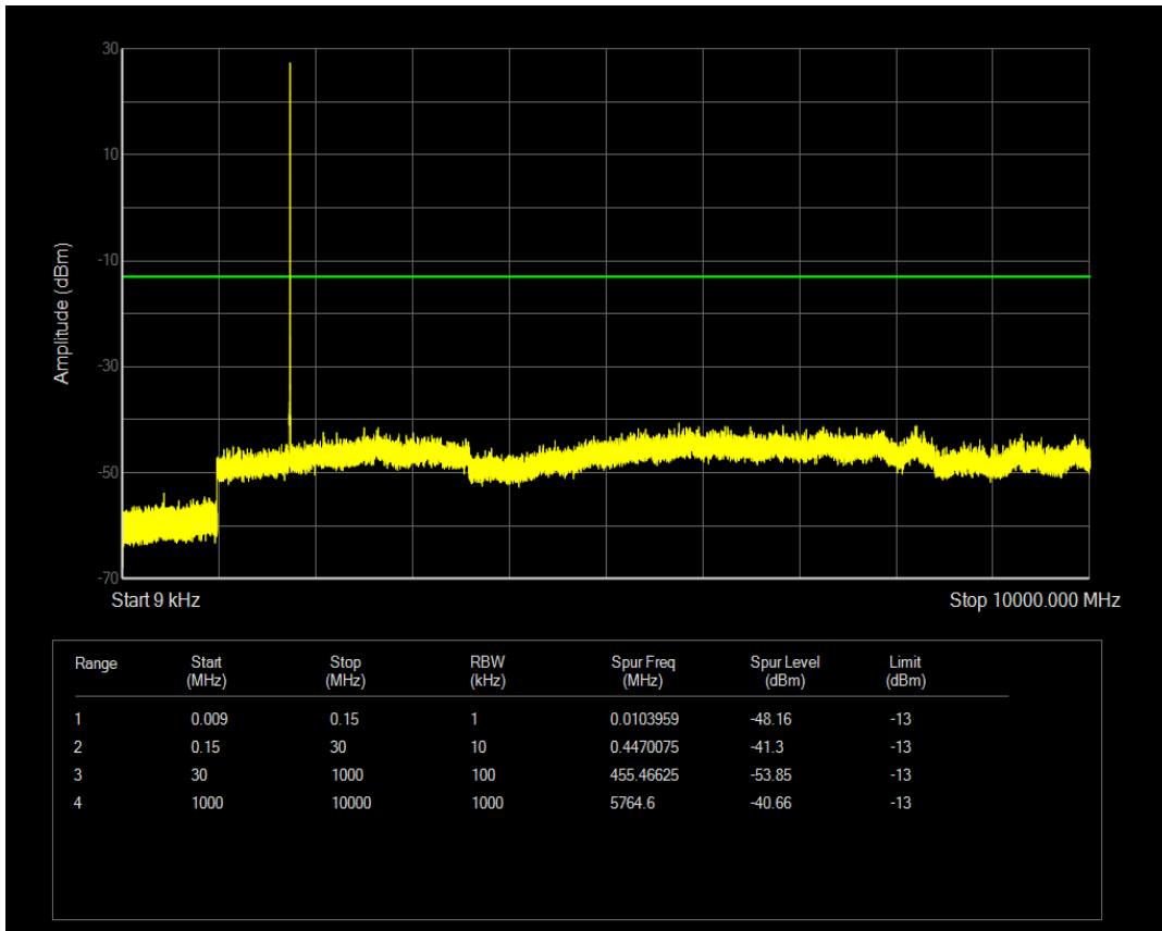
Band4 QAM16 BW=3MHz Channel=20385 RB Size=1 Position=#Mid
