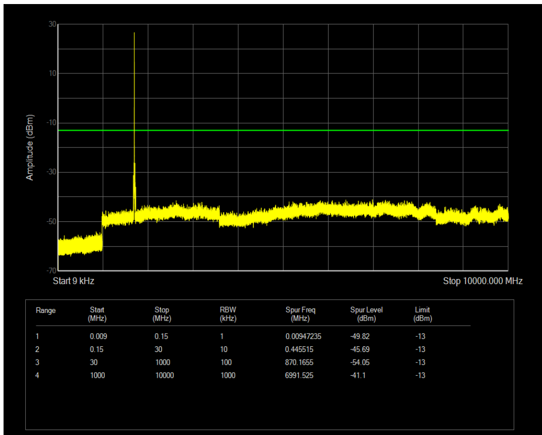
Band4 QAM16 BW=10MHz Channel=20000 RB Size=1 Position=#Mid
