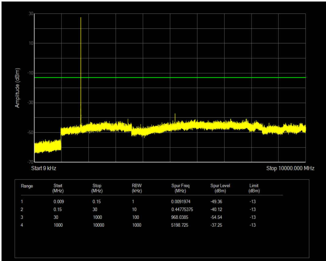
Band4 QAM16 BW=5MHz Channel=20175 RB Size=1 Position=#Mid
