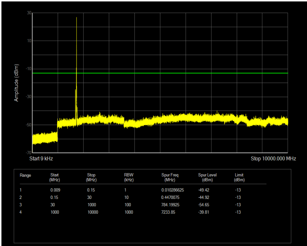
Band4 QAM16 BW=10MHz Channel=20350 RB Size=1 Position=#Mid
