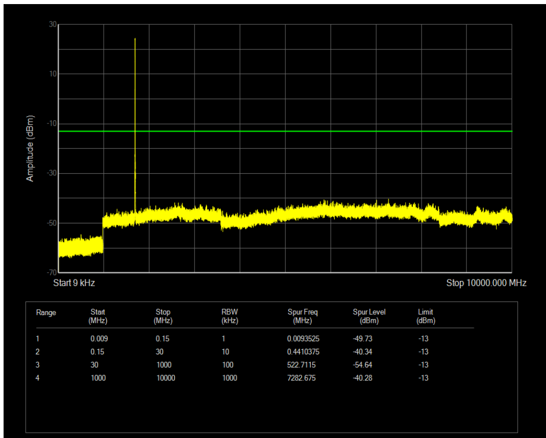
Band4 QAM16 BW=3MHz Channel=19965 RB Size=8 Position=#0
