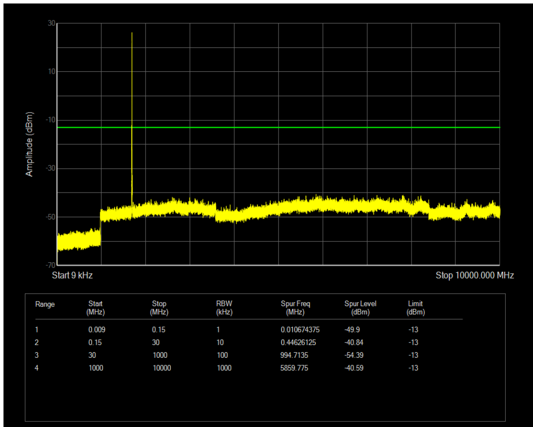
Band4 QAM16 BW=3MHz Channel=19965 RB Size=8 Position=#0
