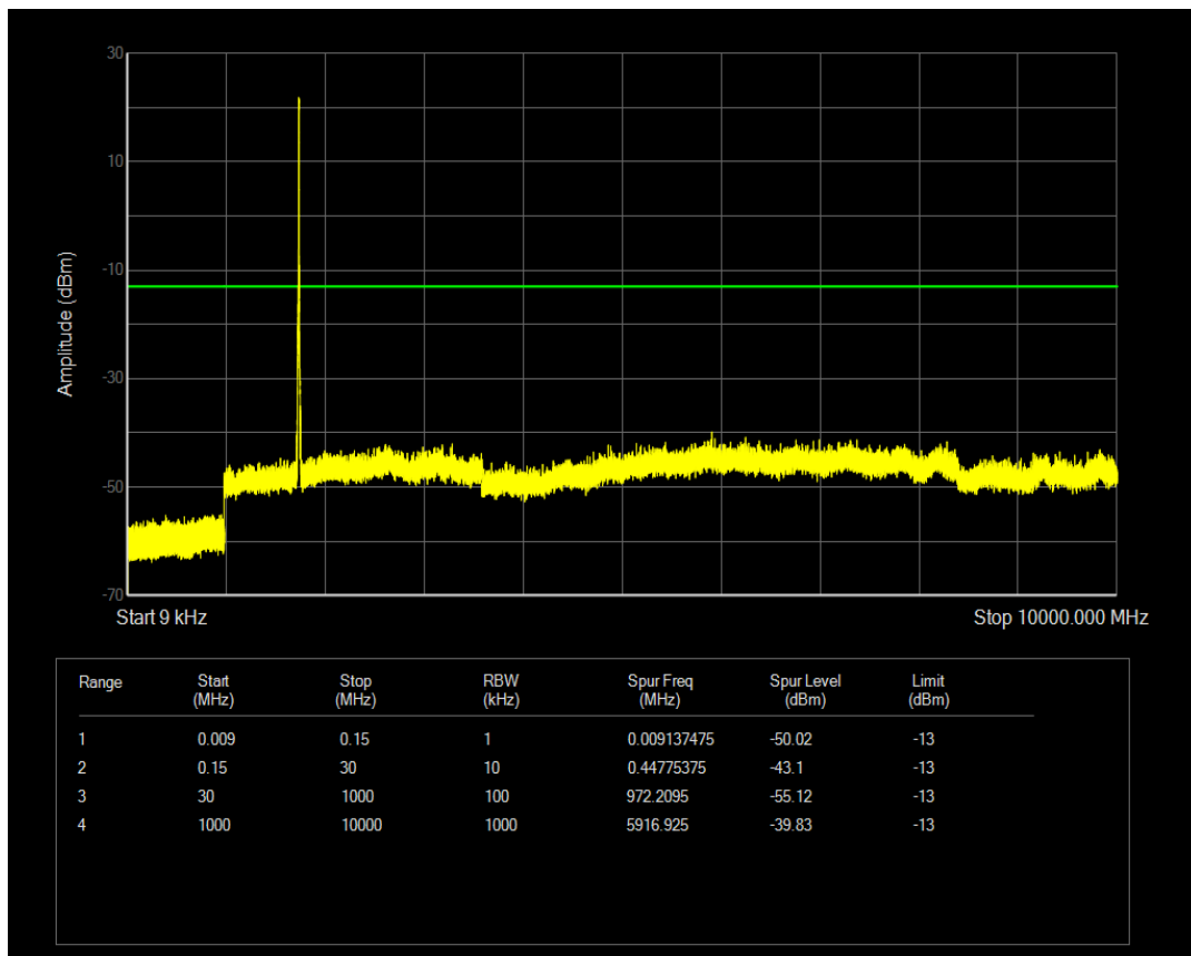
Band4 QAM16 BW=10MHz Channel=20350 RB Size=25 Position=#Max
