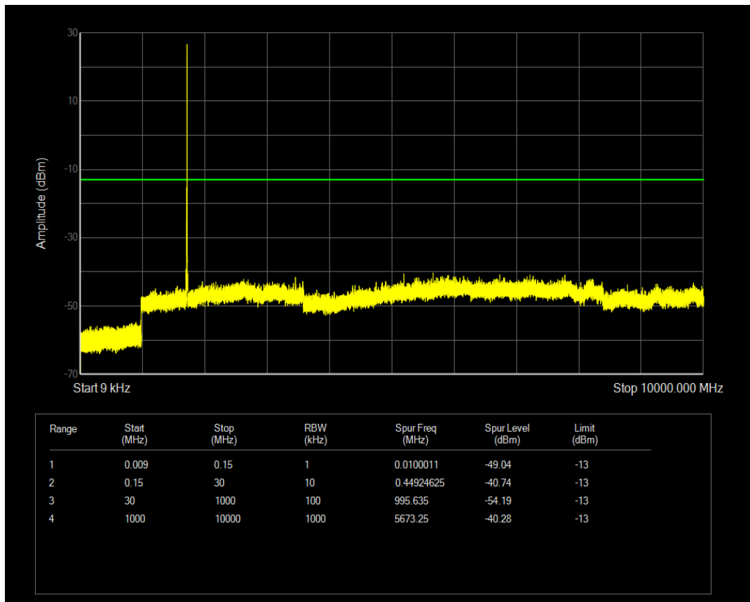
Band4 QAM16 BW=5MHz Channel=20175 RB Size=12 Position=#Max
