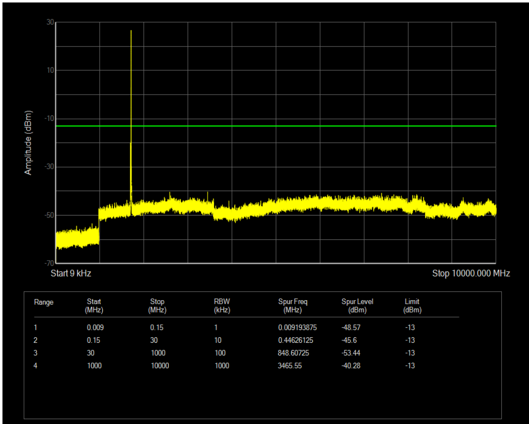
Band4 QAM16 BW=10MHz Channel=20175 RB Size=1 Position=#Mid
