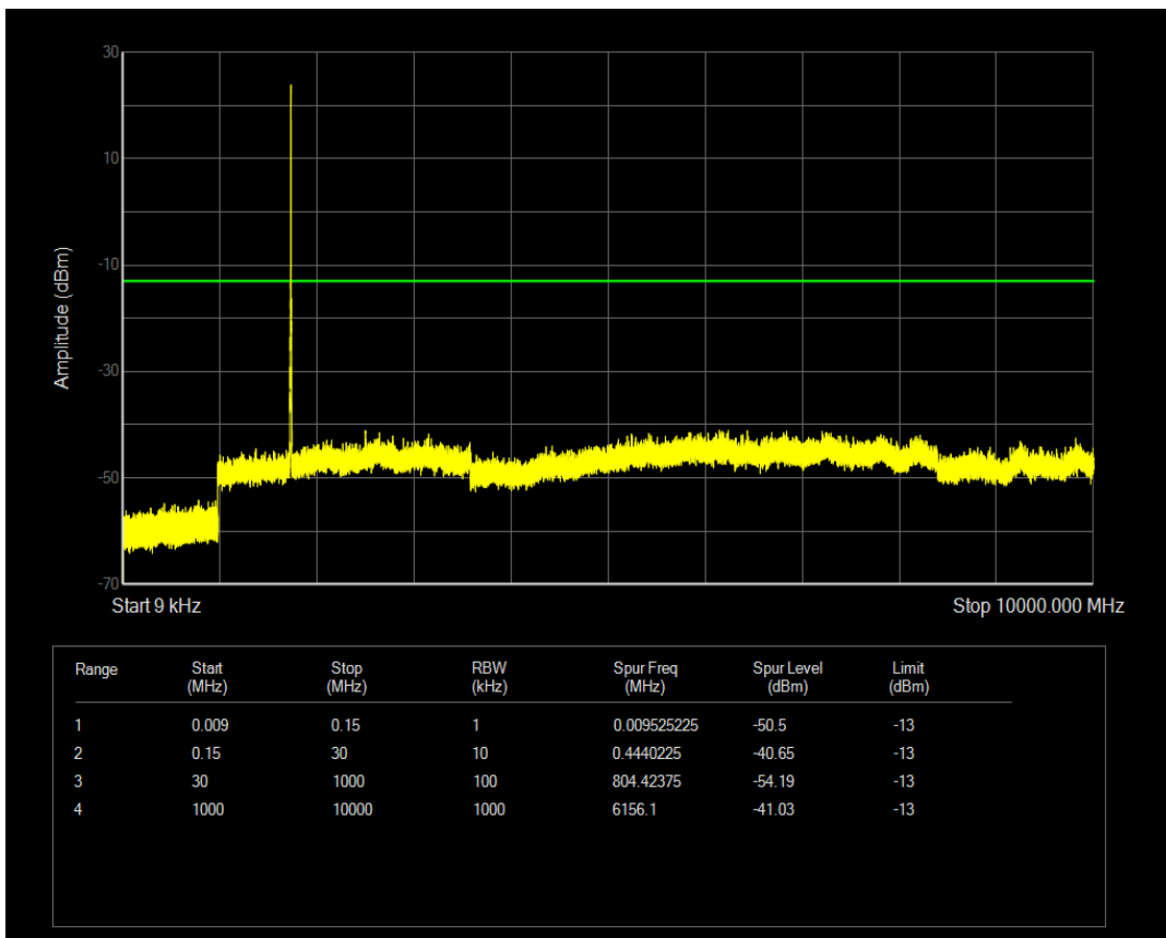
Band4 QPSK BW=5MHz Channel=20375 RB Size=12 Position=#0
