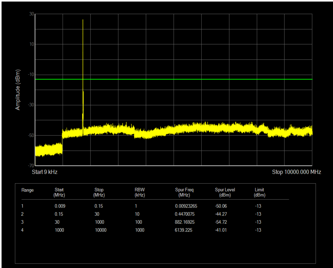
Band4 QAM16 BW=10MHz Channel=20350 RB Size=1 Position=#Mid
