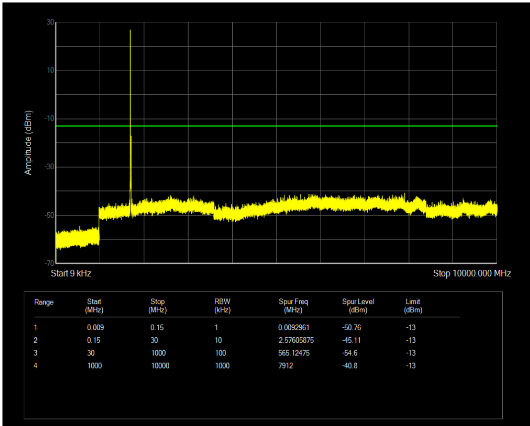
Band4 QPSK BW=10MHz Channel=20000 RB Size=1 Position=#Mid
