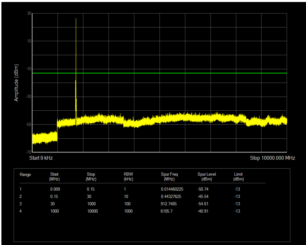
Band4 QPSK BW=10MHz Channel=20175 RB Size=25 Position=#0
