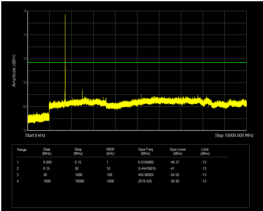
Band4 QAM16 BW=5MHz Channel=20175 RB Size=1 Position=#Mid
