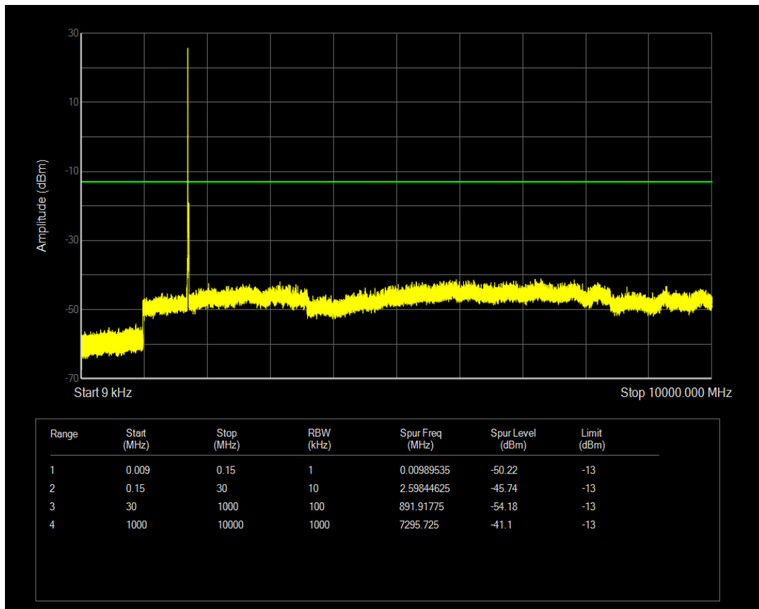
Band4 QAM16 BW=10MHz Channel=20000 RB Size=1 Position=#Mid
