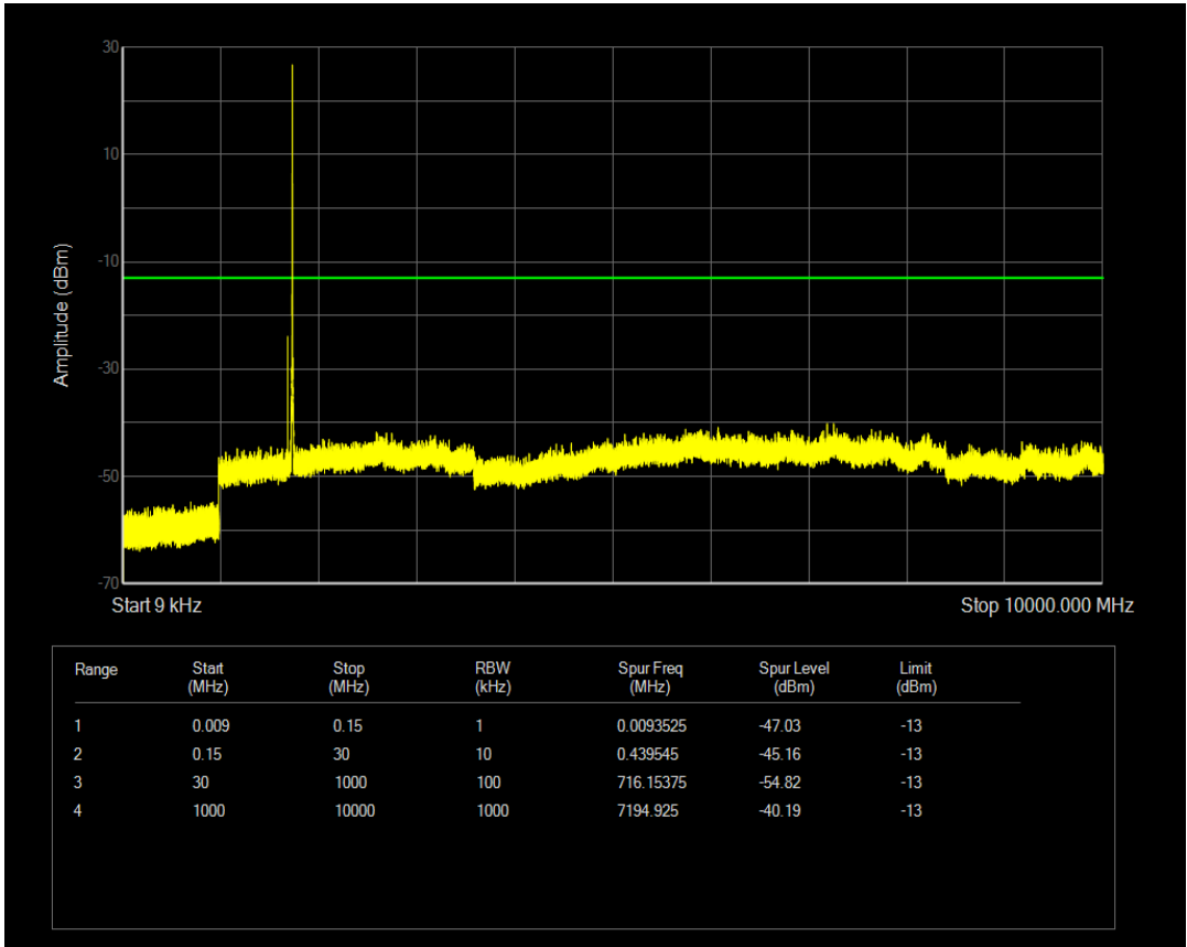
Band4 QPSK BW=10MHz Channel=20350 RB Size=25 Position=#0
