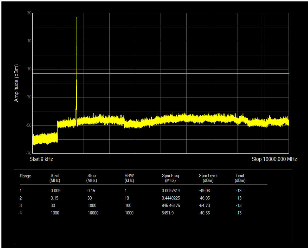
Band4 QAM16 BW=10MHz Channel=20175 RB Size=1 Position=#Mid
