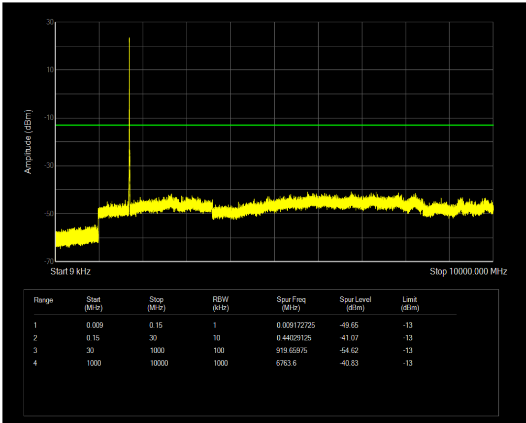
Band4 QPSK BW=3MHz Channel=20175 RB Size=1 Position=#Mid
