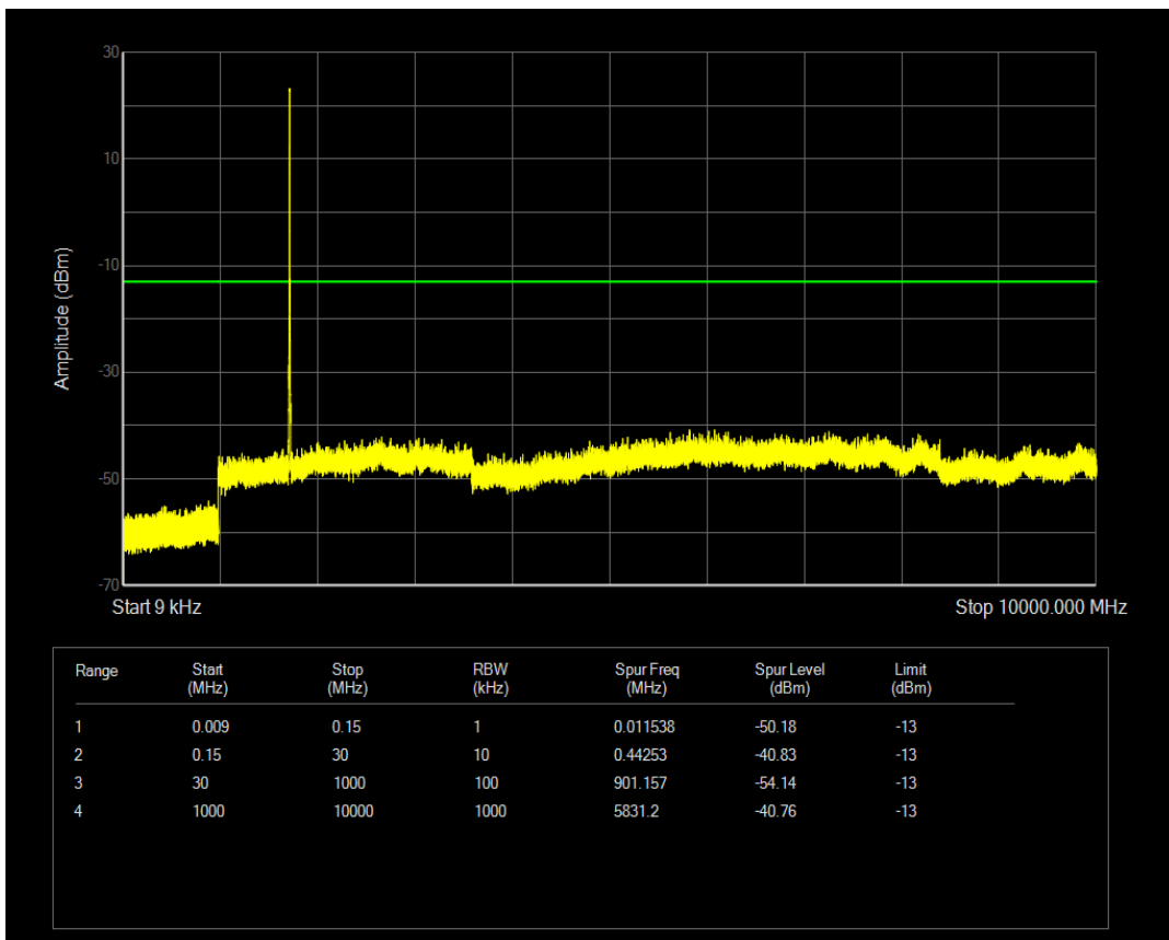
Band4 QPSK BW=5MHz Channel=20175 RB Size=12 Position=#0
