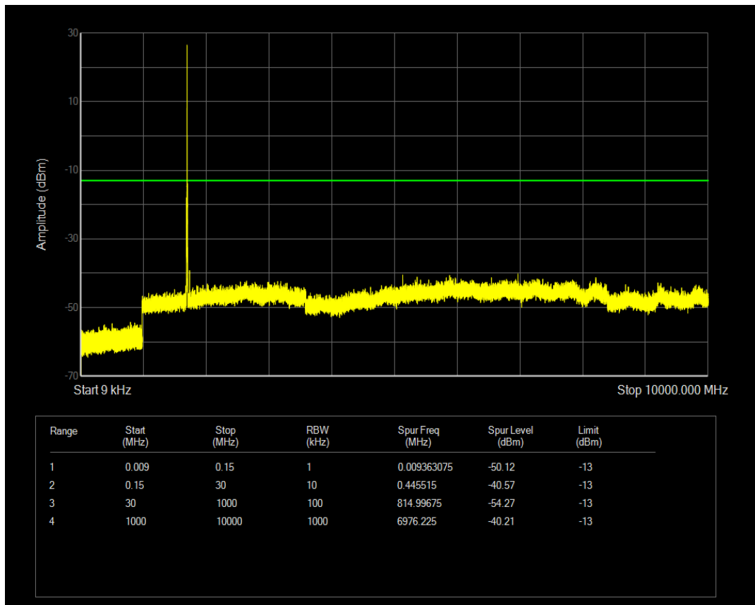
Band4 QAM16 BW=5MHz Channel=19975 RB Size=12 Position=#0
