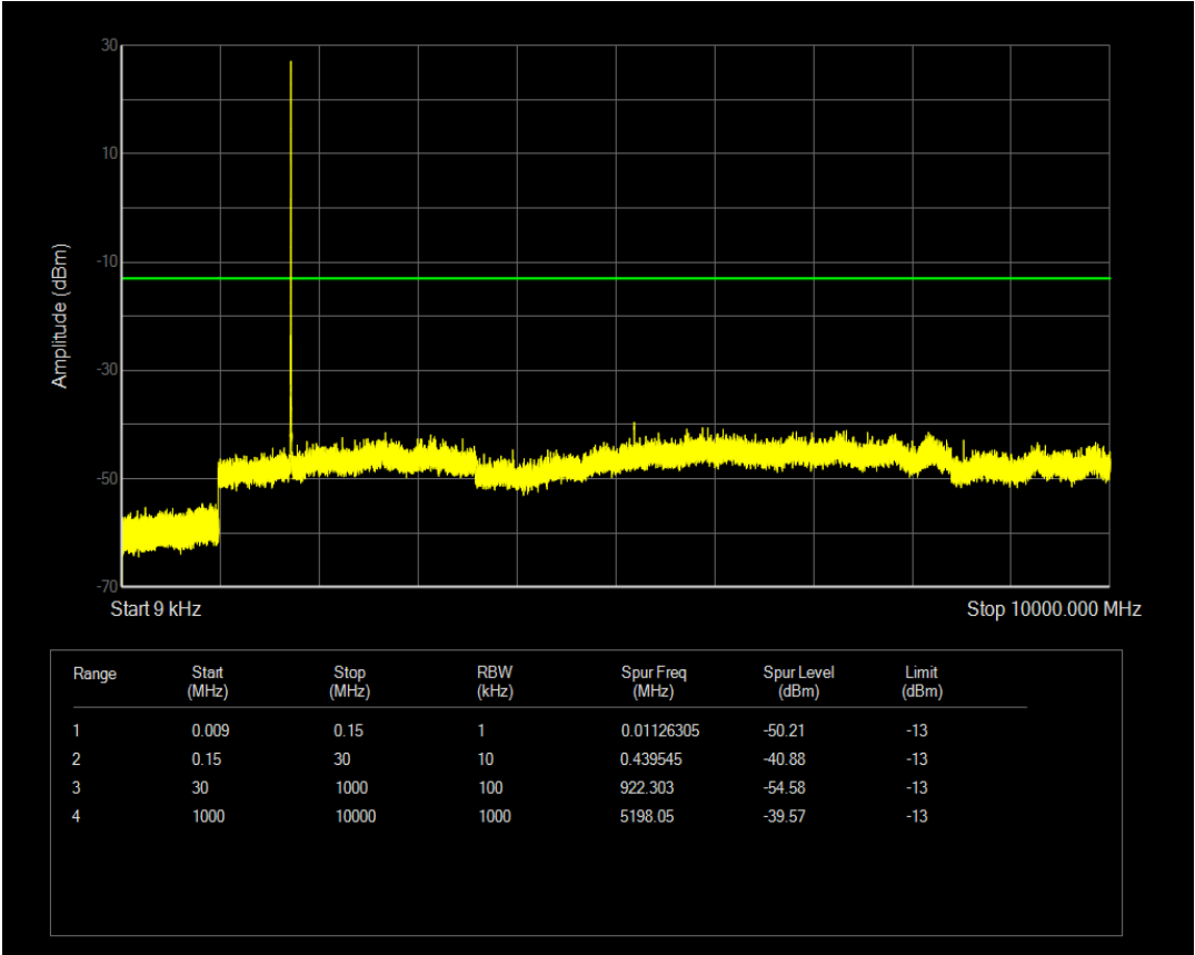
Band4 QPSK BW=5MHz Channel=20175 RB Size=1 Position=#Mid
