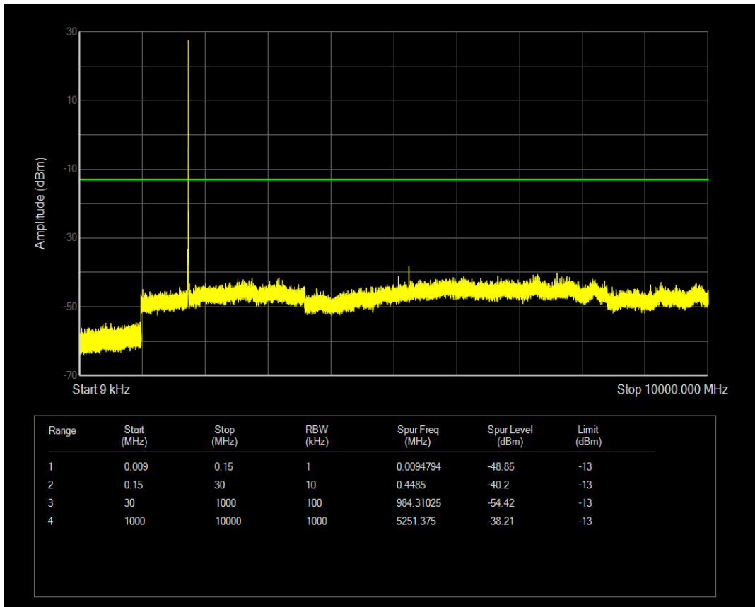
Band4 QAM16 BW=5MHz Channel=20375 RB Size=1 Position=#Mid
