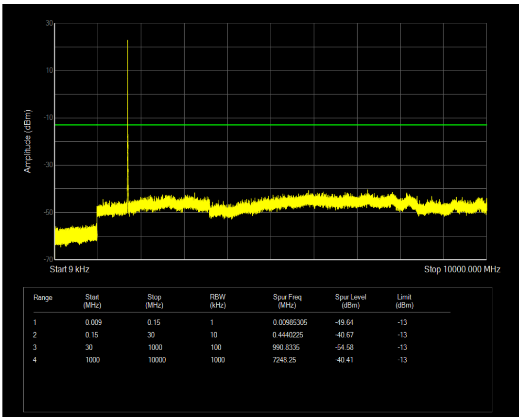
Band4 QPSK BW=5MHz Channel=19975 RB Size=12 Position=#0
