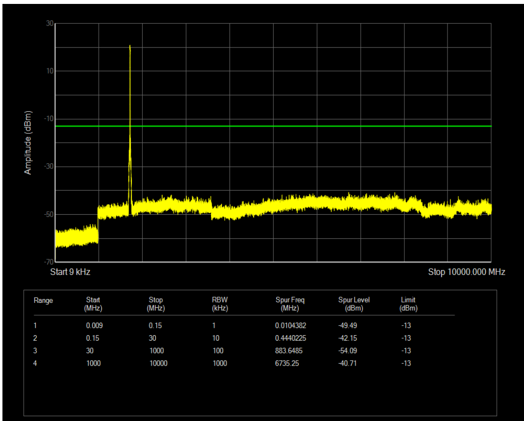
Band4 QPSK BW=20MHz Channel=20175 RB Size=50 Position=#Max
