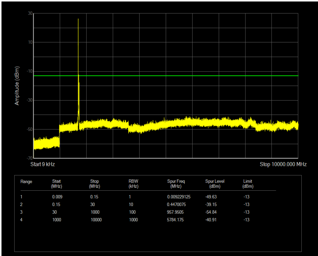
Band4 QAM16 BW=20MHz Channel=20050 RB Size=1 Position=#Mid
