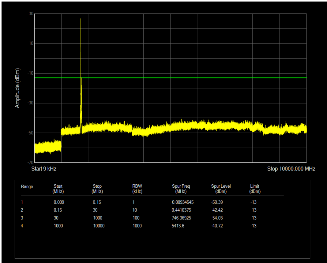
Band4 QPSK BW=20MHz Channel=20175 RB Size=1 Position=#Mid
