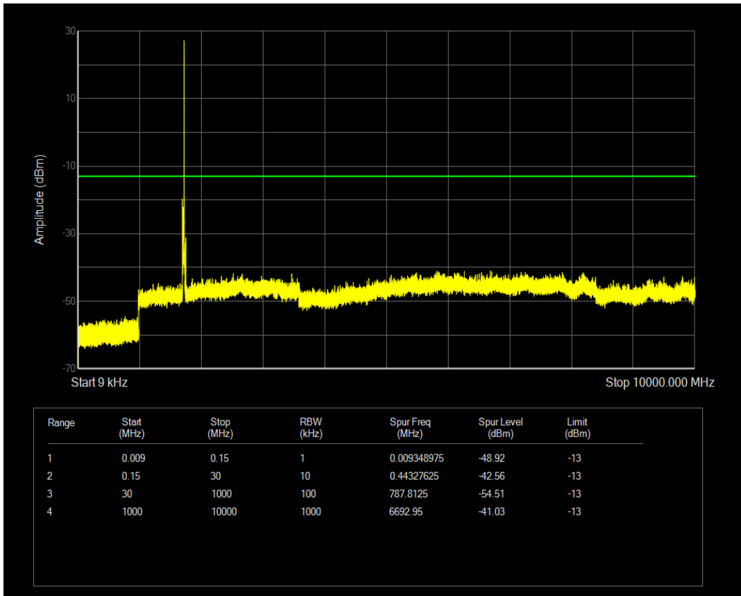
Band4 QAM16 BW=15MHz Channel=20175 RB Size=36 Position=#Max
