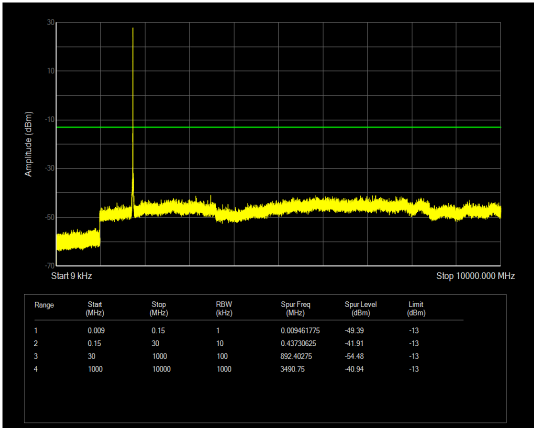
Band4 QPSK BW=20MHz Channel=20300 RB Size=1 Position=#Mid
