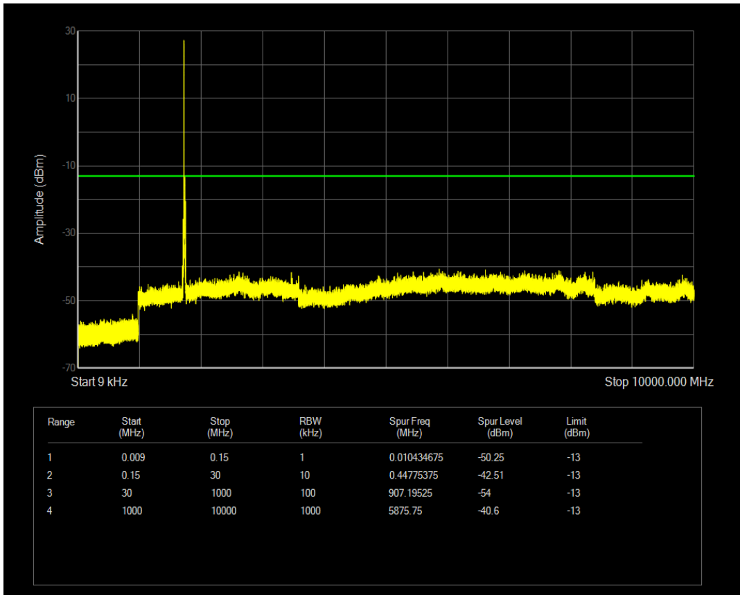
Band4 QPSK BW=15MHz Channel=20325 RB Size=1 Position=#Mid
