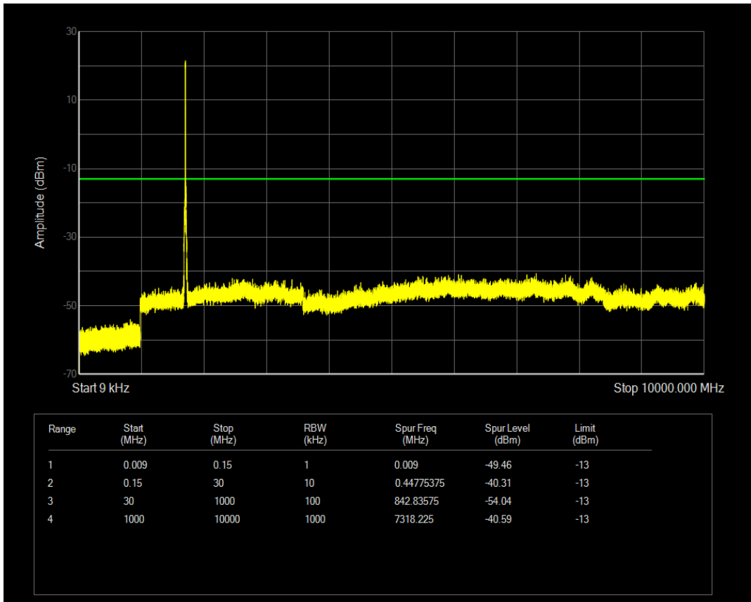
Band4 QPSK BW=15MHz Channel=20025 RB Size=36 Position=#Max
