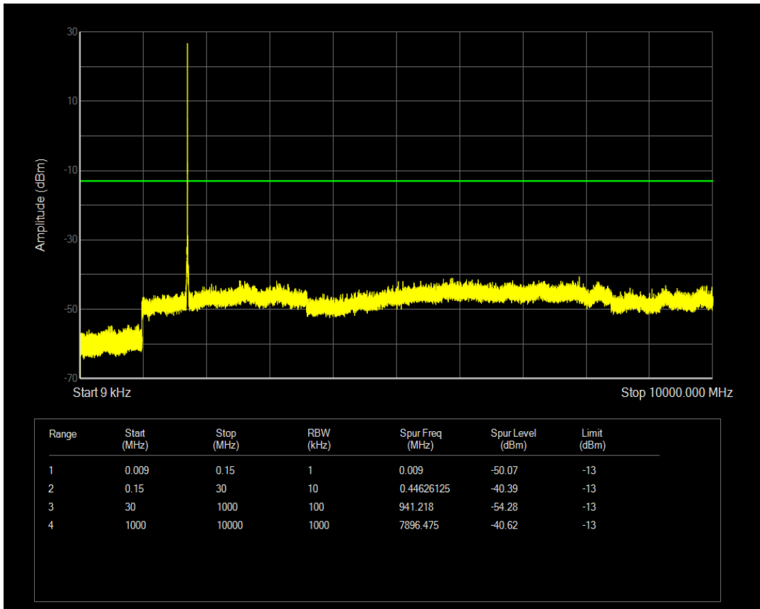
Band4 QAM16 BW=15MHz Channel=20025 RB Size=1 Position=#Mid
