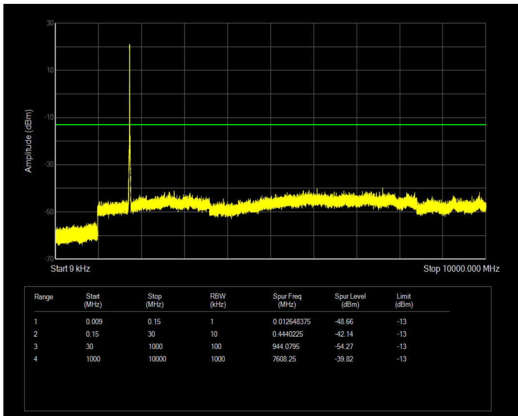
Band4 QAM16 BW=15MHz Channel=20325 RB Size=36 Position=#0
