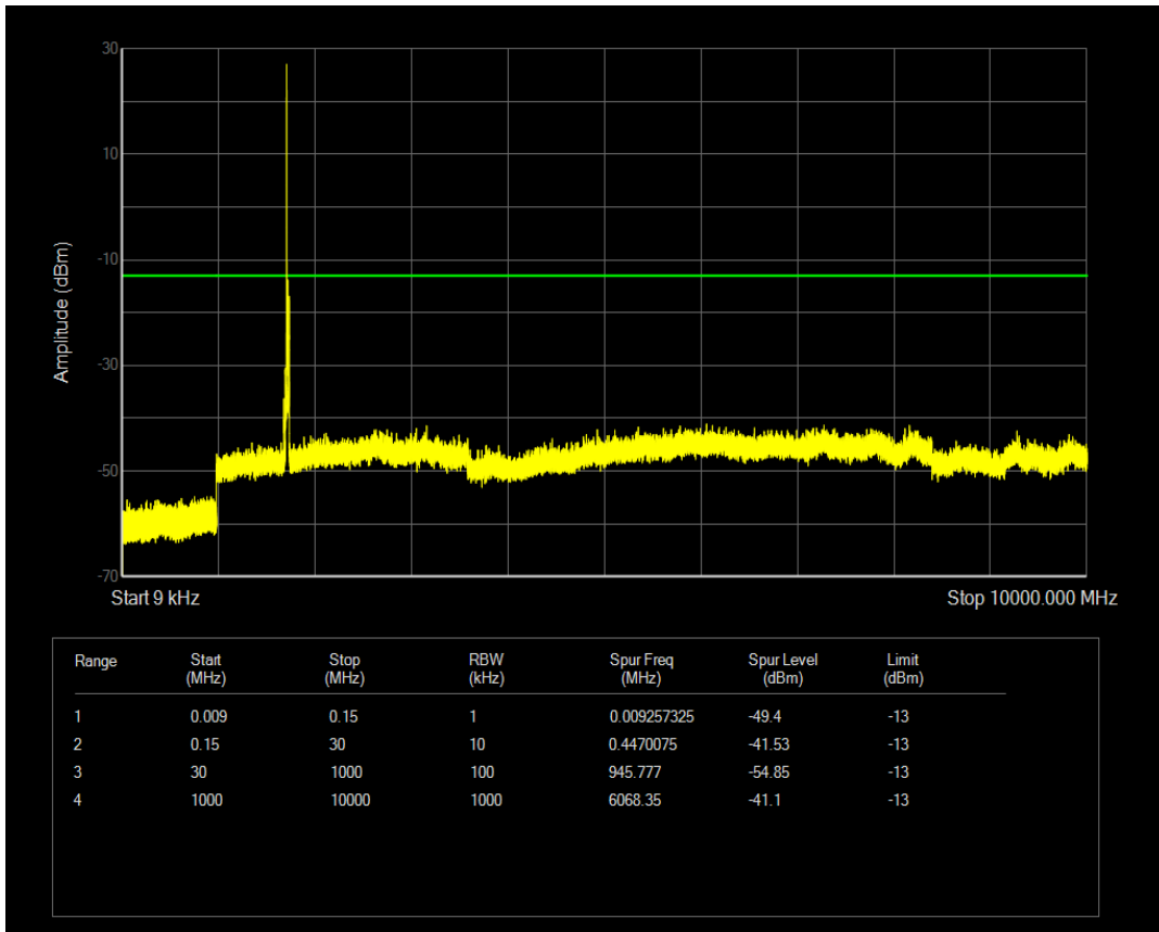
Band4 QPSK BW=15MHz Channel=20175 RB Size=1 Position=#Mid
