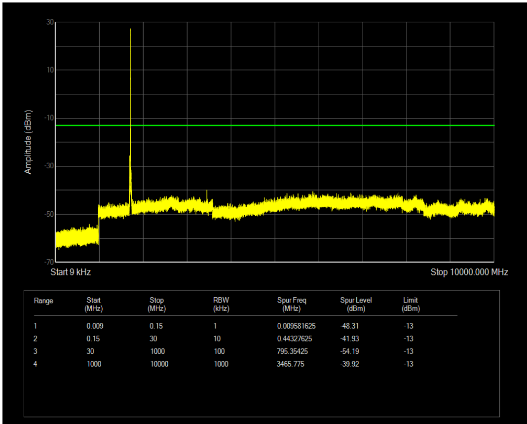
Band4 QAM16 BW=20MHz Channel=20175 RB Size=50 Position=#0
