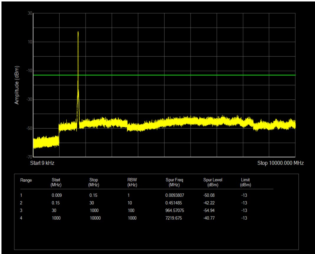
Band4 QPSK BW=20MHz Channel=20300 RB Size=1 Position=#Mid
