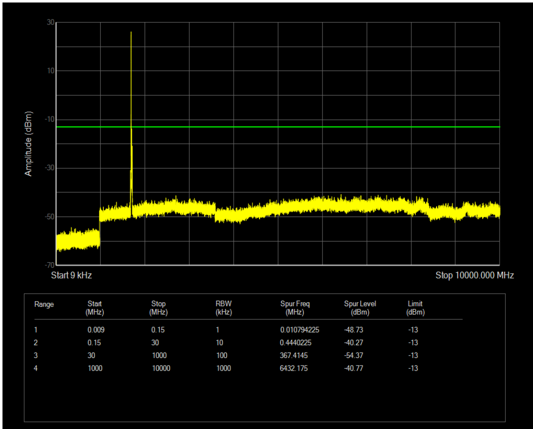
Band4 QAM16 BW=15MHz Channel=20025 RB Size=1 Position=#Mid
