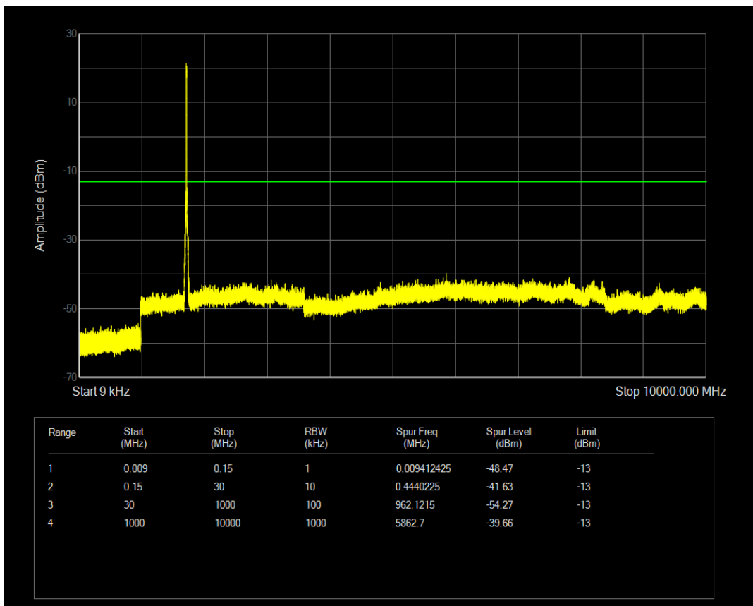
Band4 QPSK BW=20MHz Channel=20175 RB Size=50 Position=#0
