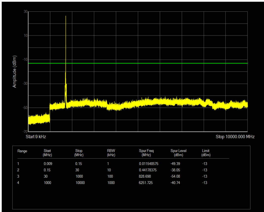
Band4 QPSK BW=20MHz Channel=20050 RB Size=50 Position=#0
