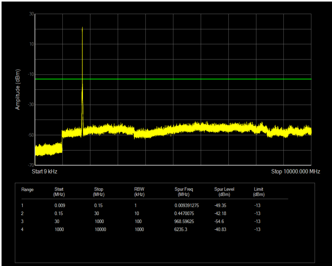
Band4 QAM16 BW=15MHz Channel=20175 RB Size=36 Position=#Max
