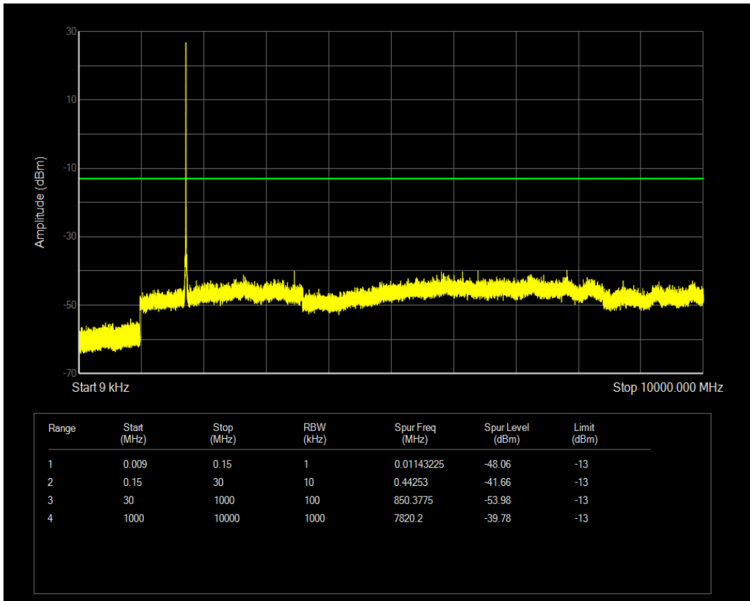
Band4 QPSK BW=15MHz Channel=20175 RB Size=1 Position=#Mid
