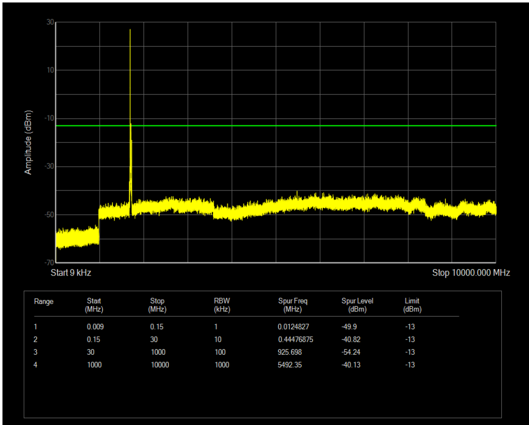
Band4 QPSK BW=20MHz Channel=20050 RB Size=1 Position=#Mid
