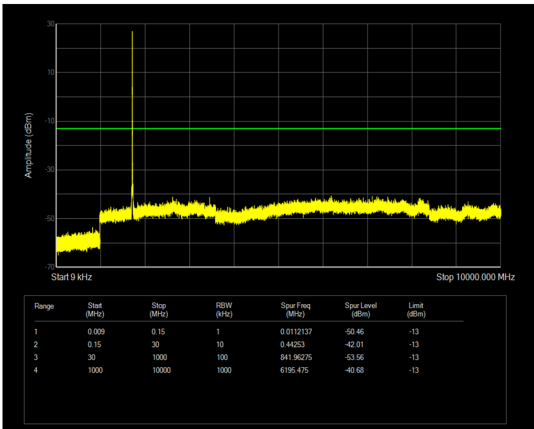
Band4 QAM16 BW=15MHz Channel=20175 RB Size=1 Position=#Mid
