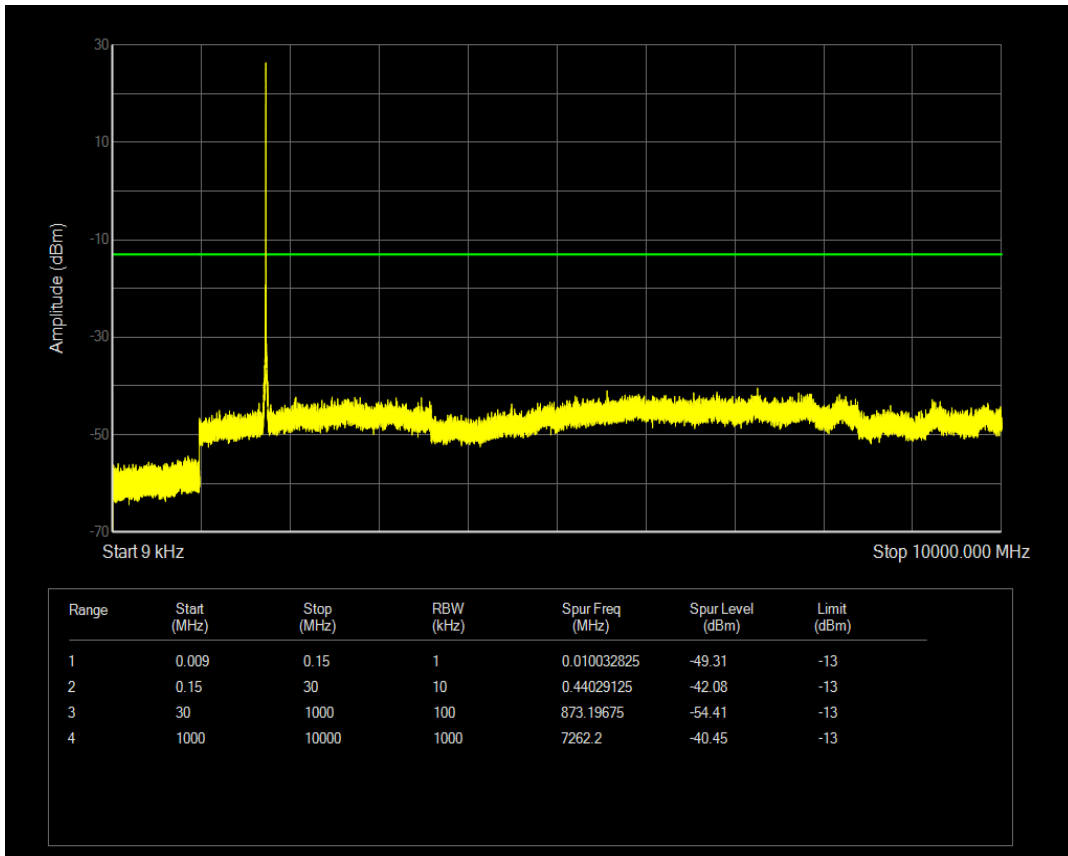
Band4 QAM16 BW=20MHz Channel=20300 RB Size=1 Position=#Mid
