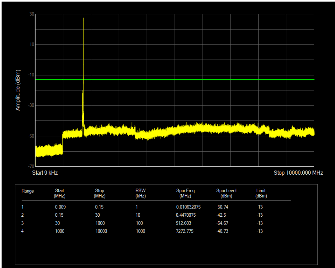
Band4 QAM16 BW=20MHz Channel=20175 RB Size=1 Position=#Max
