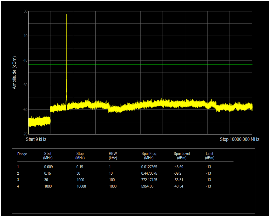
Band4 QAM16 BW=20MHz Channel=20050 RB Size=1 Position=#Mid
