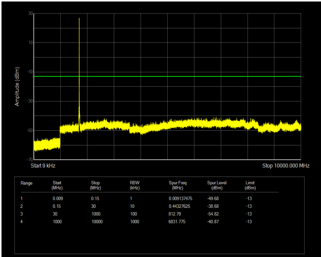
Band4 QPSK BW=20MHz Channel=20050 RB Size=1 Position=#Mid
