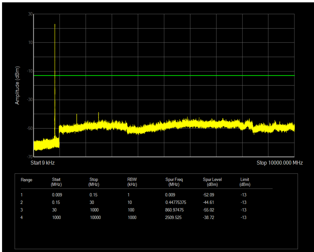
Band5 QAM16 BW=1.4MHz Channel=20525 RB Size=3 Position=#0
