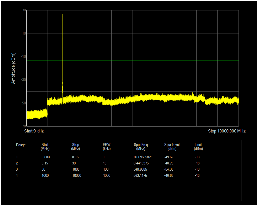
Band4 QPSK BW=15MHz Channel=20025 RB Size=36 Position=#0
