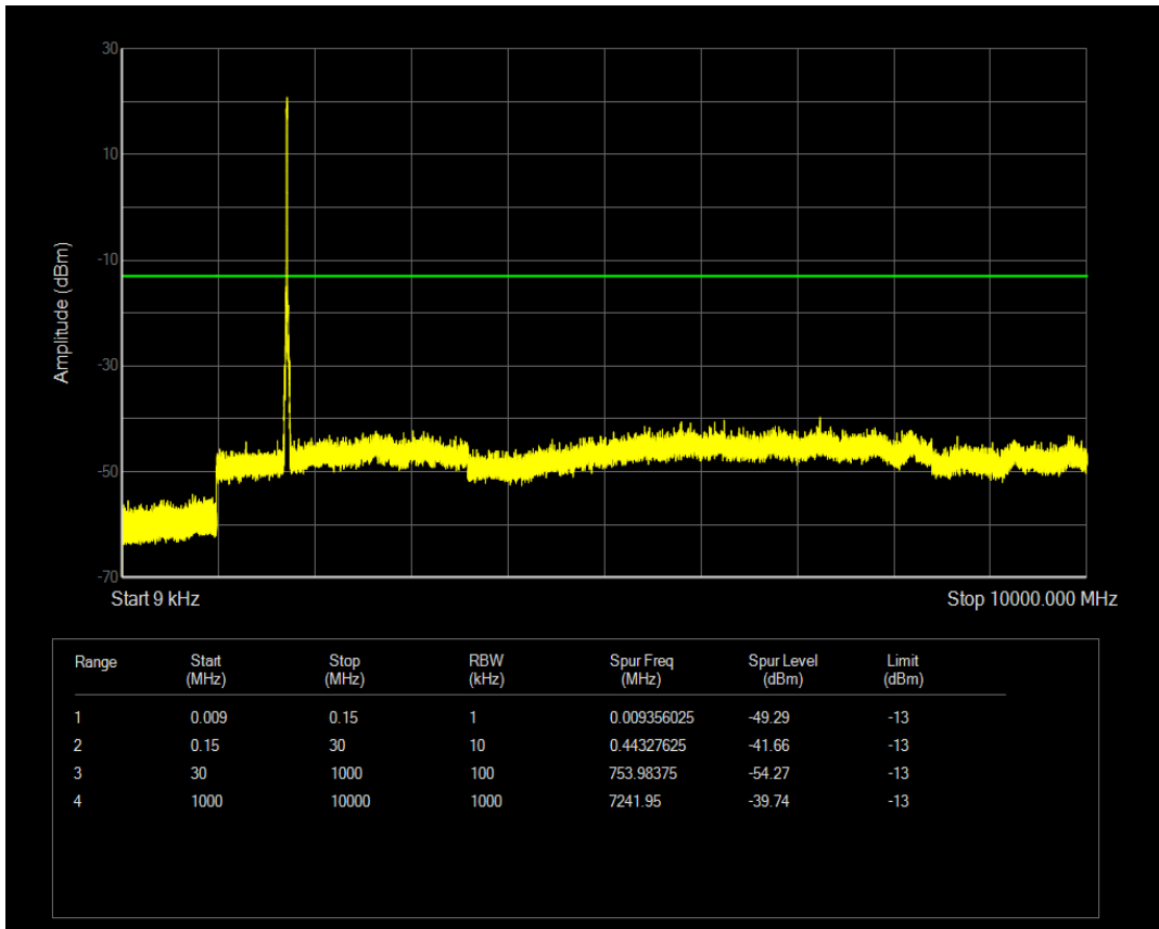
Band4 QAM16 BW=20MHz Channel=20175 RB Size=50 Position=#0
