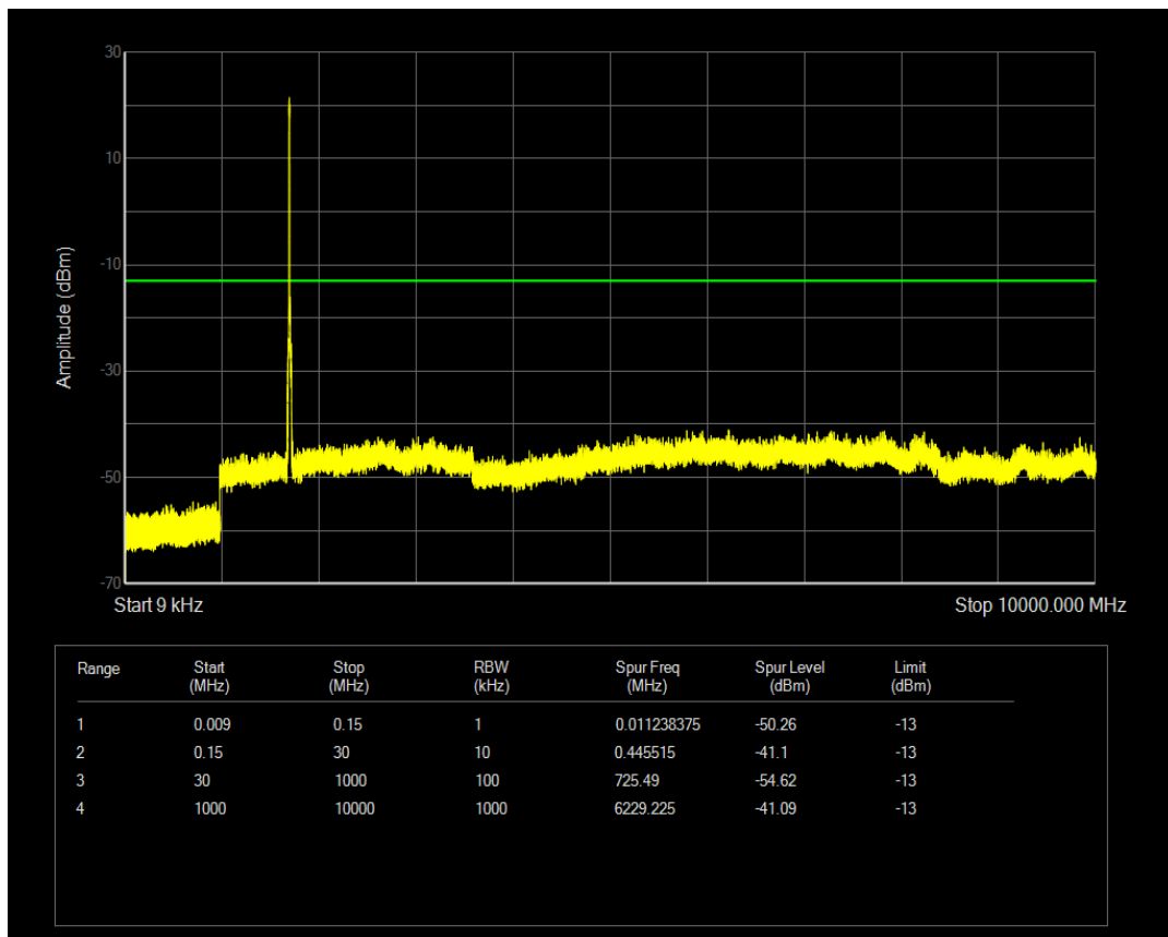
Band4 QAM16 BW=15MHz Channel=20025 RB Size=36 Position=#0
