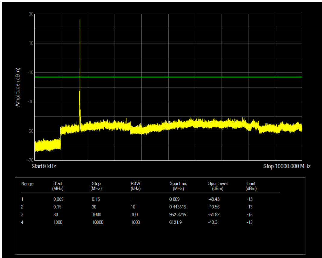
Band4 QAM16 BW=15MHz Channel=20025 RB Size=36 Position=#0
