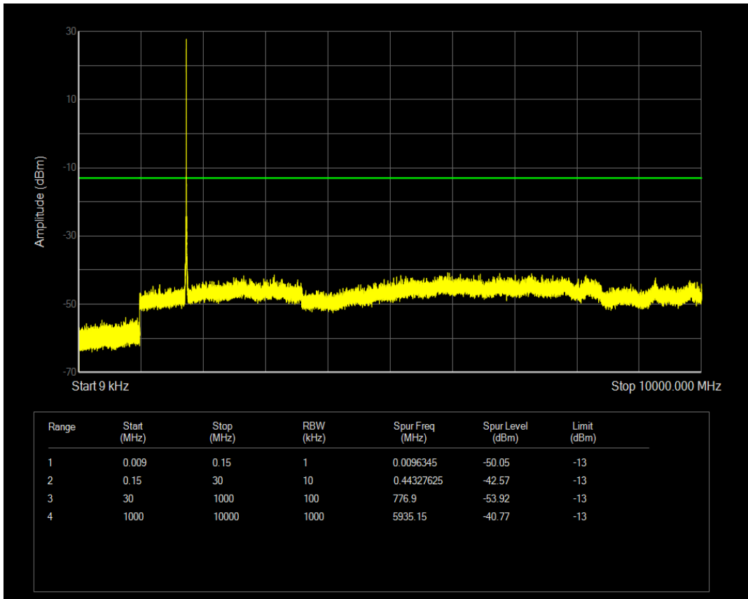
Band4 QPSK BW=15MHz Channel=20325 RB Size=1 Position=#Mid
