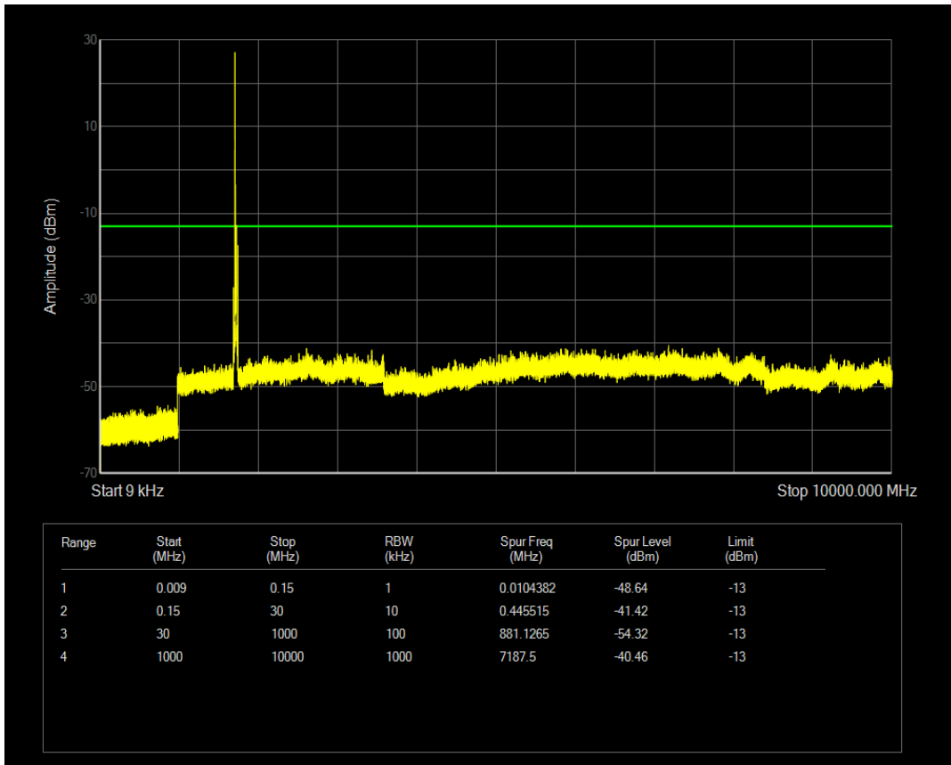
Band4 QAM16 BW=20MHz Channel=20175 RB Size=1 Position=#Max
