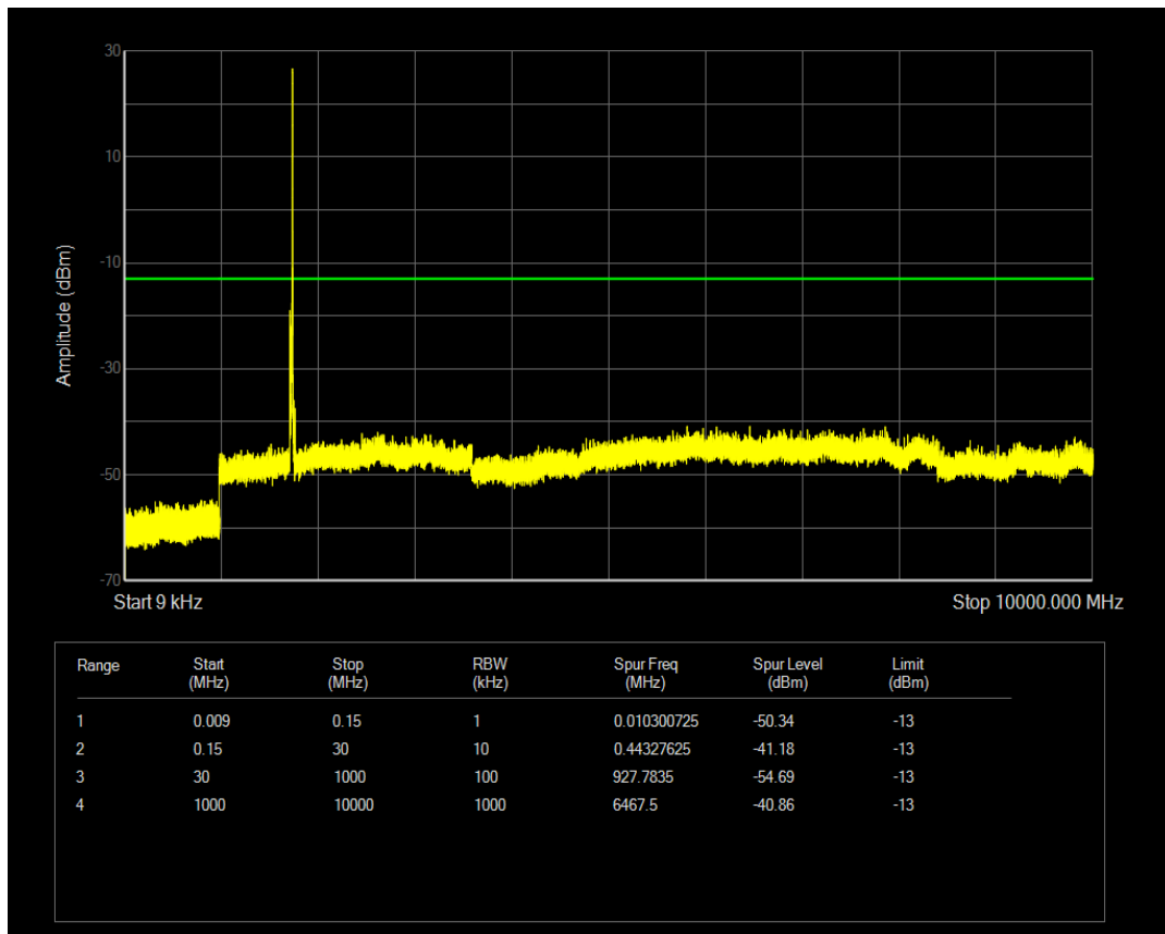
Band4 QAM16 BW=15MHz Channel=20325 RB Size=36 Position=#0
