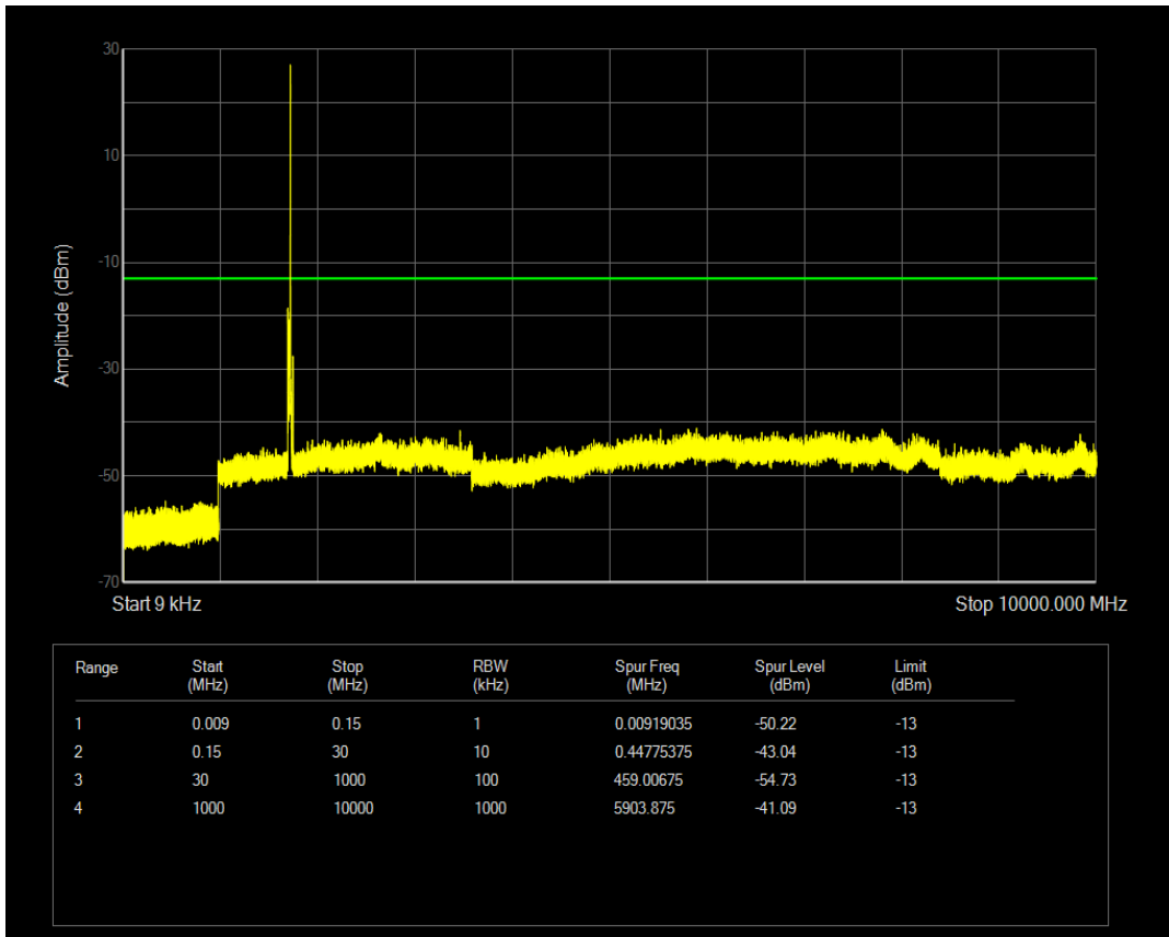
Band4 QPSK BW=15MHz Channel=20175 RB Size=1 Position=#Max
