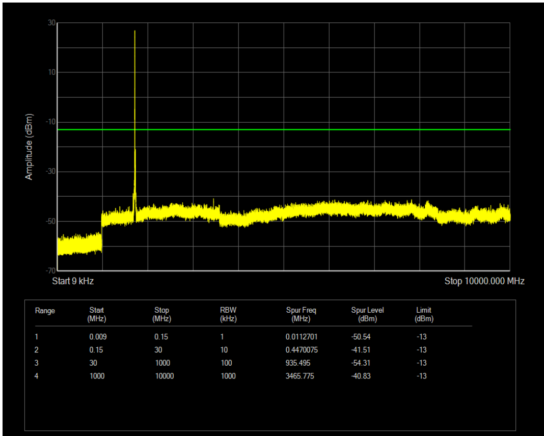
Band4 QPSK BW=20MHz Channel=20175 RB Size=1 Position=#Mid
