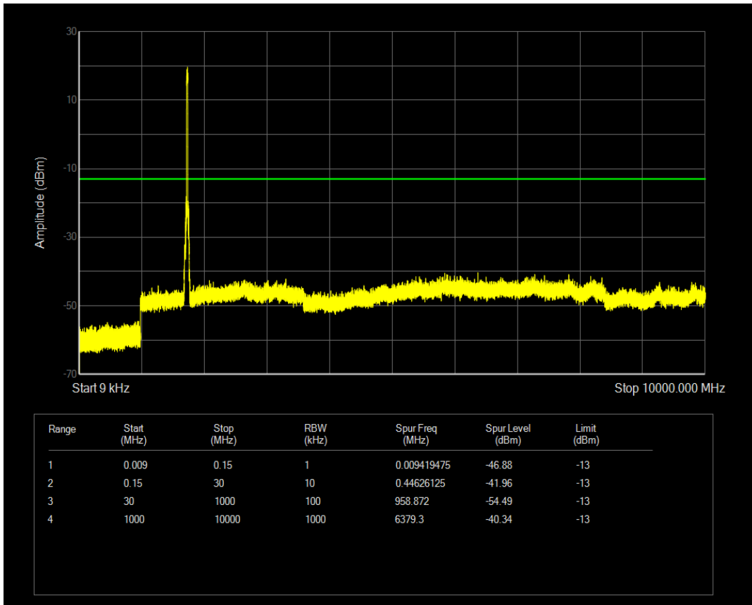
Band4 QAM16 BW=20MHz Channel=20300 RB Size=1 Position=#Mid
