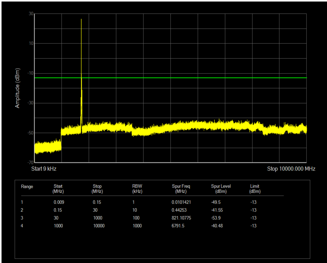
Band4 QAM16 BW=15MHz Channel=20325 RB Size=1 Position=#Mid
