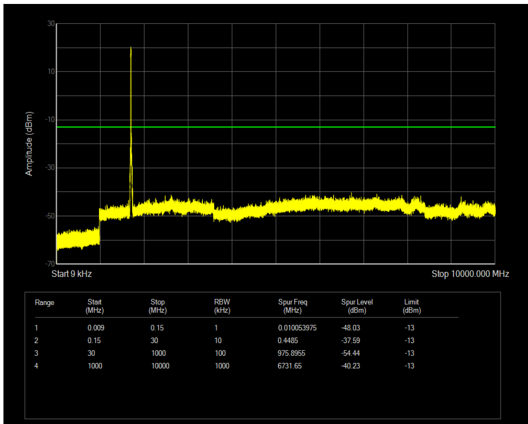
Band4 QPSK BW=20MHz Channel=20050 RB Size=50 Position=#0
