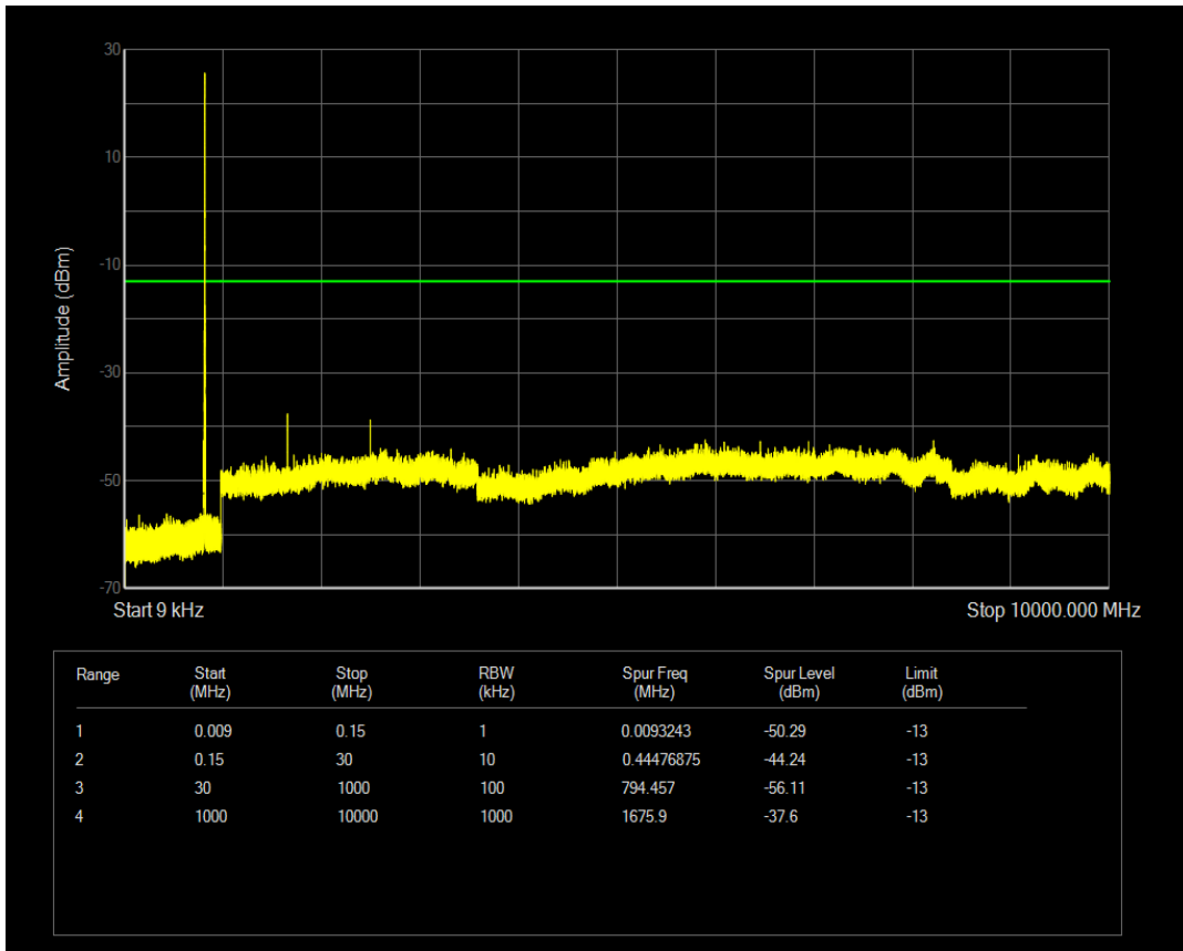
Band5 QPSK BW=3MHz Channel=20525 RB Size=8 Position=#0
