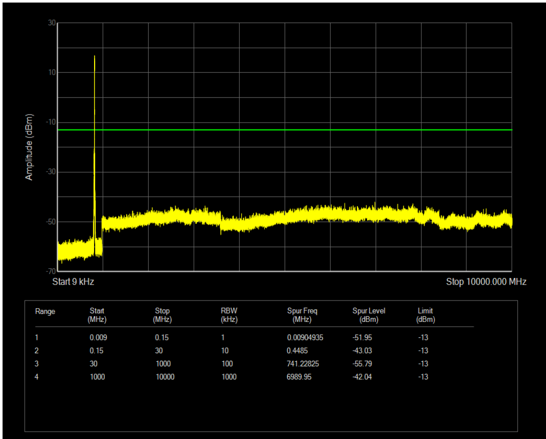
Band5 QAM16 BW=5MHz Channel=20525 RB Size=1 Position=#Max
