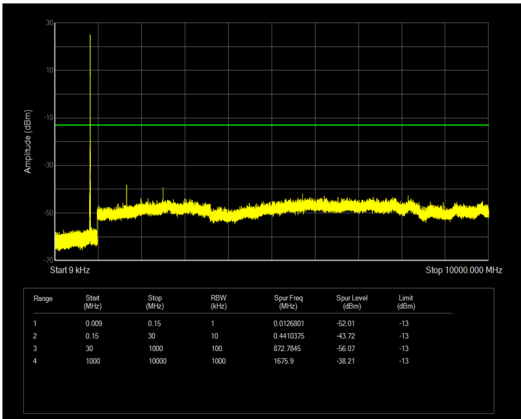
Band5 QAM16 BW=3MHz Channel=20525 RB Size=8 Position=#Max
