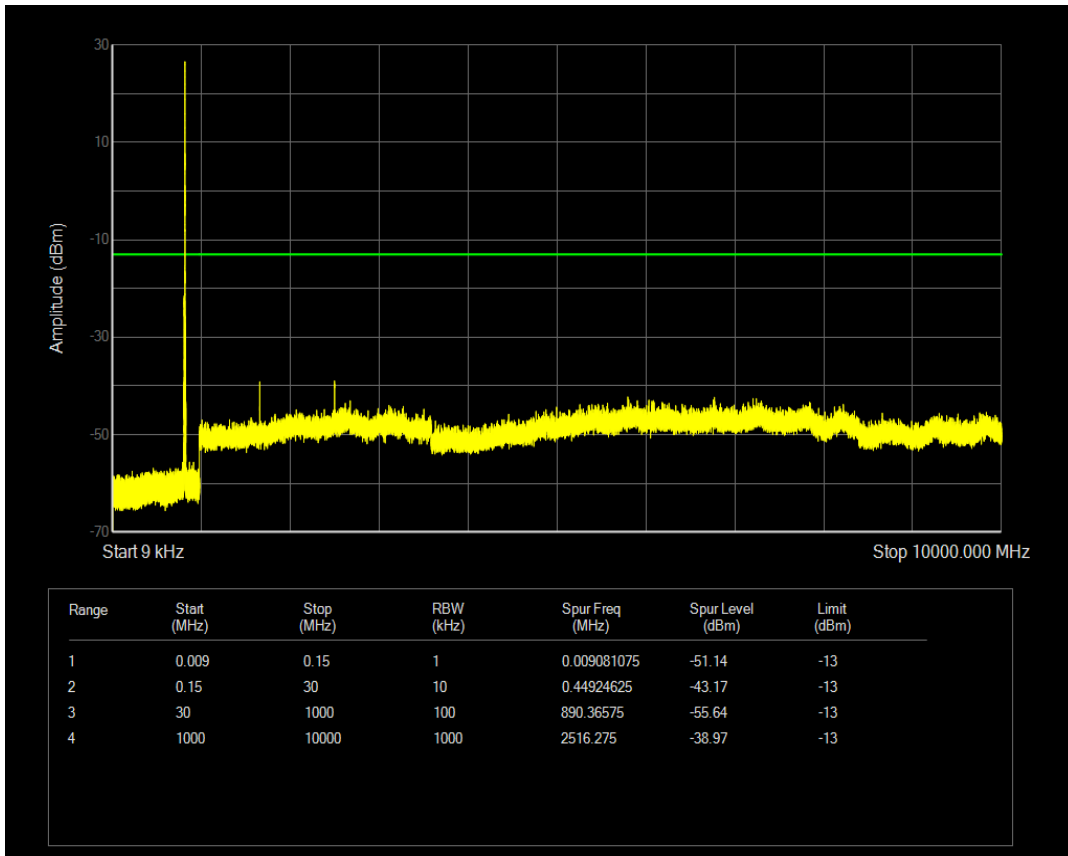
Band5 QAM16 BW=5MHz Channel=20525 RB Size=1 Position=#Max
