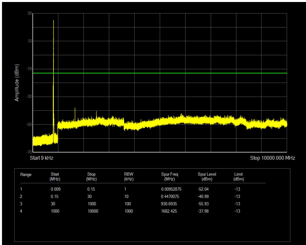
Band5 QAM16 BW=10MHz Channel=20525 RB Size=25 Position=#Max
