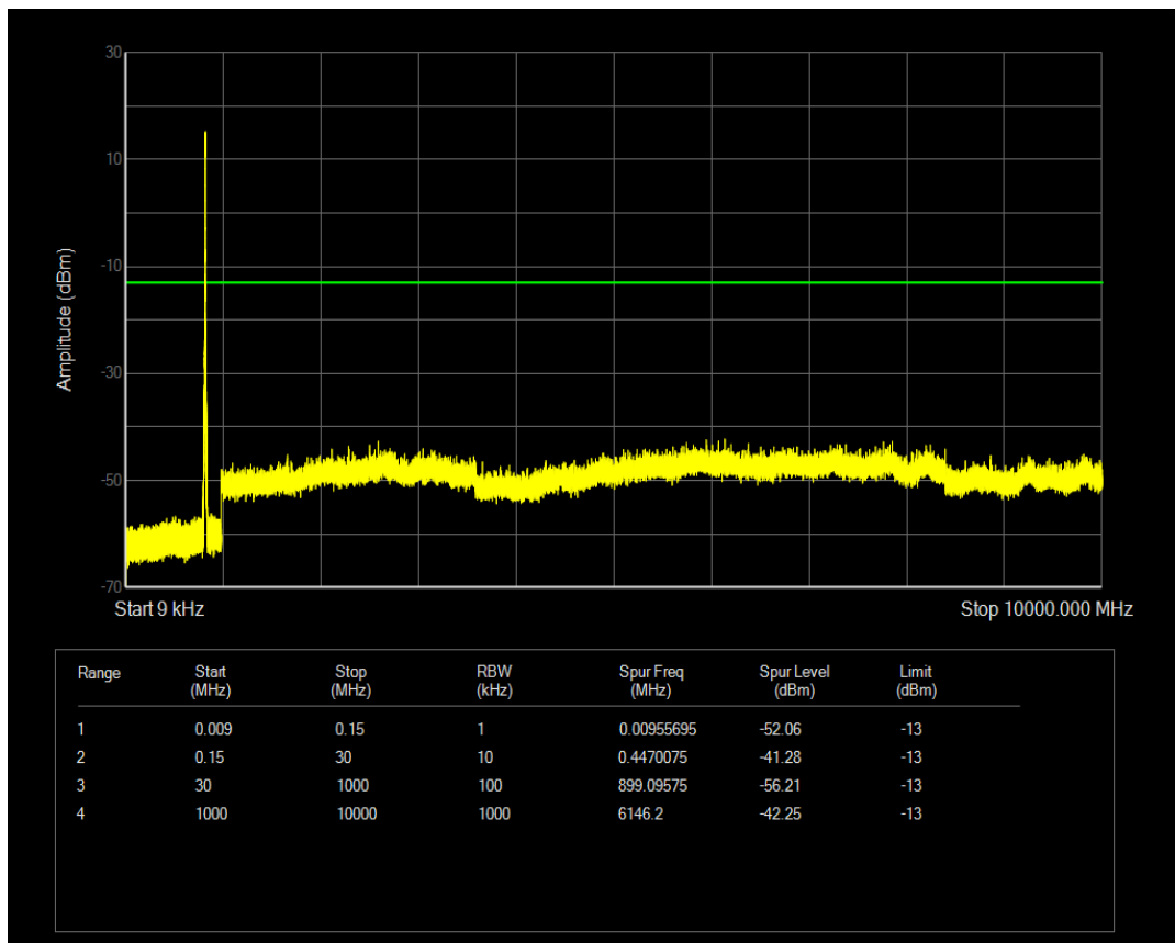
Band5 QAM16 BW=10MHz Channel=20525 RB Size=25 Position=#Max
