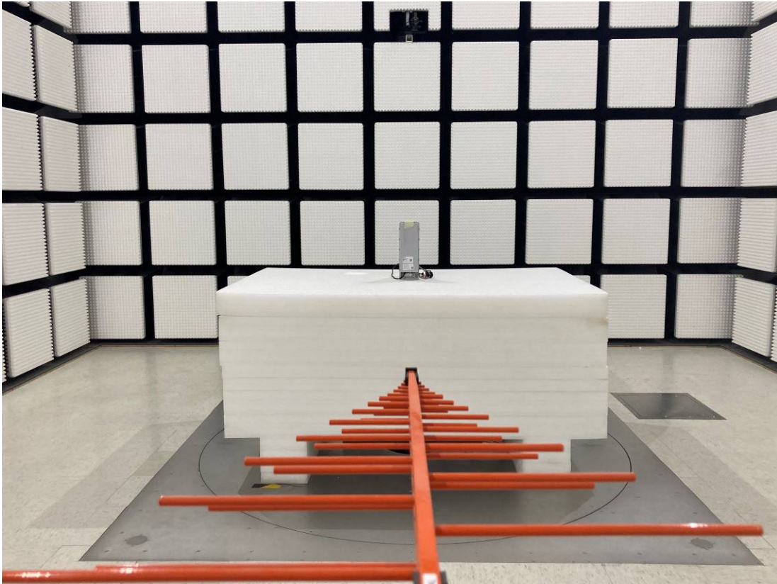
Radiated Emission Below 1GHz View DC Power
