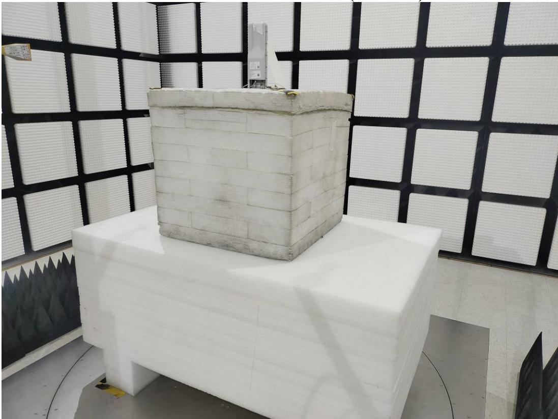
Radiated Emission Above 1GHz View-(40-60GHz) POE
