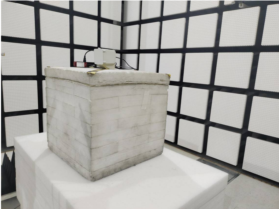
Radiated Emission Above 1GHz View-(140-200G)
