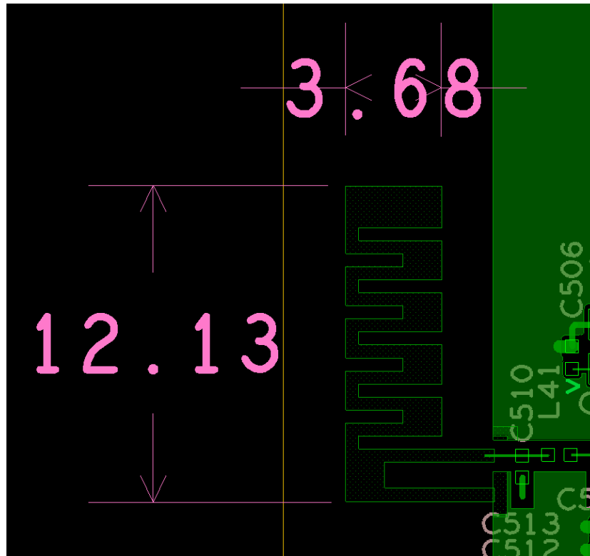
Bluetooth 2.4G Antenna
