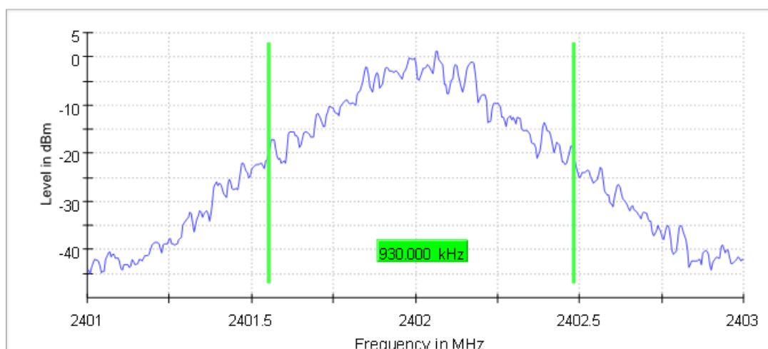
20 dB Bandwidth
