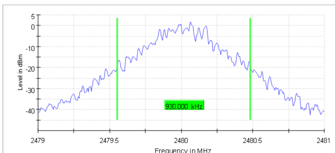
20 dB Bandwidth
