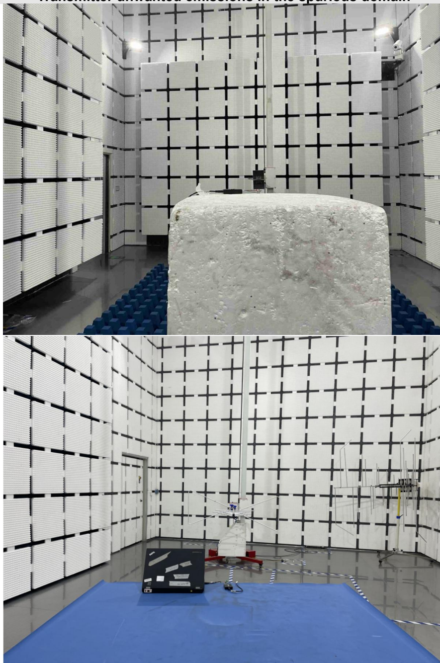
Transmitter unwanted emissions in the spurious domain
