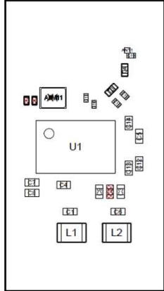
View from Top side (Scale 4:1)
