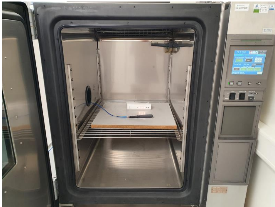
Test Setup: Frequency Stability Measurements
