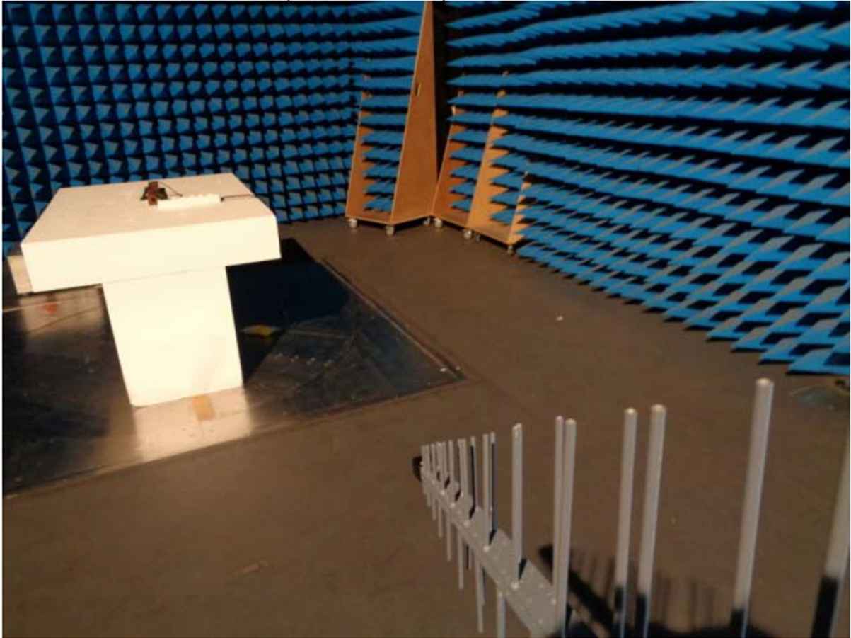
Photo : radiates emission (200-1000MHz)
