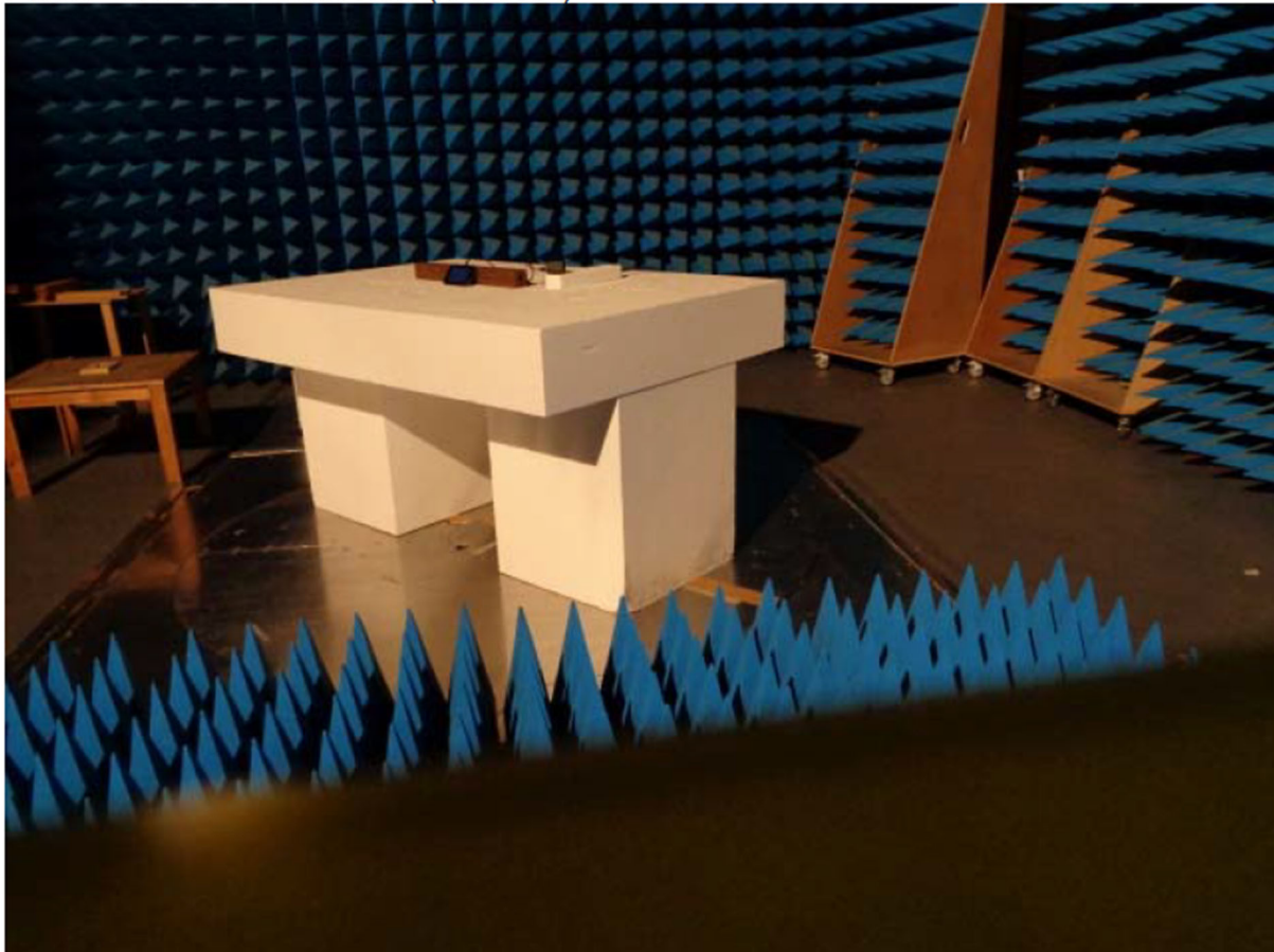
Photo : radiates emission (1-6GHz)
