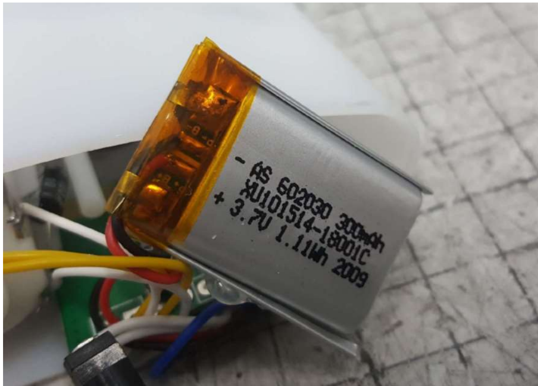
Battery
