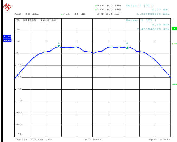
Channel Separation Plot on Channel 00 - 01
