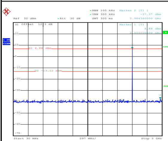
CSE Plot on CH 00 between 30 MHz ~ 3 GHz
