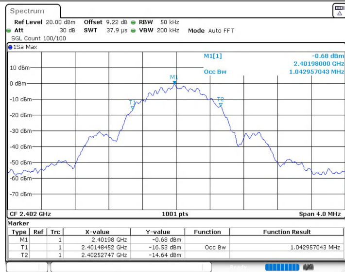
BLE_1M_Ant1_2402
