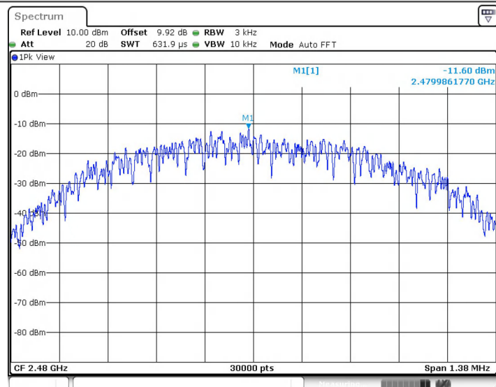
BLE_1M_Ant1_2480
