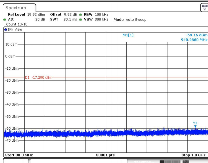
BLE_2M_Ant1_2480_0~Reference
